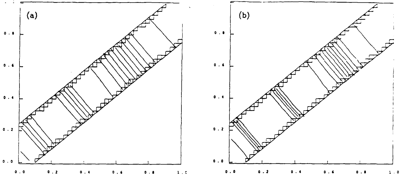
Figure 9.1 Density contours for a shock tube at 40^\circ to the grid. The irregular boundary cells of the computational grid are also shown. (a) First order method. (b) With high resolution correction waves included.
