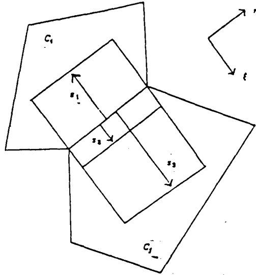
Figure 6.1. Two grid cells C_i and C_j from an unstructured grid. Wave propagation from the cell interface is determined by solving a one dimensional Riemann problem in the \xi -direction, giving rise to waves propagating with velocities s_1 , s_2 , and s_3 .
