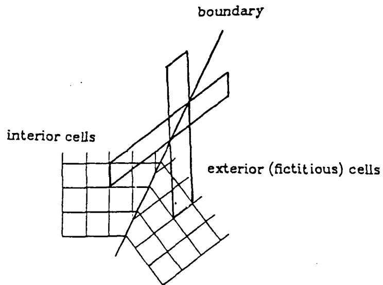
Figure 8.1. Cartesian mesh cut by a flat boundary. Reflecting the interior cells through this boundary gives the fictitious exterior cells. Each wave propagating across the boundary from an interior cell interface is matched by a wave propagating into the region from a fictitious interface. This can also be viewed as a reflection of the interior wave at the boundary.
