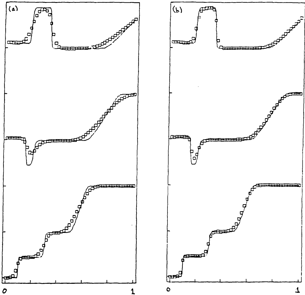
Figure 5.1. The density \rho in the shock tube problem at three different times (reading upward). Figure (a) shows the values obtained with slopes \sigma_{jp} = 0 . Figure (b) shows the values obtained with minmod slopes (3.9c).
