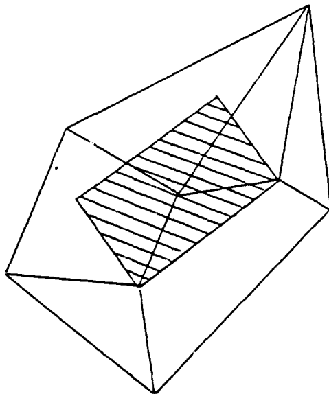
Figure 6.2. Propagation of a wave over a general unstructured grid. Cell values are updated in every cell the wave intersects. The contribution to each cell is proportional to the ratio of the shaded area within that cell to the total cell area.
