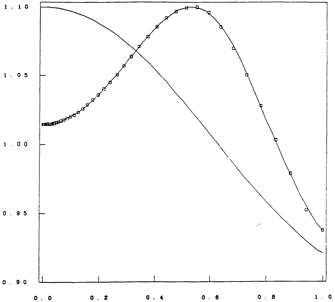
Figure 5.2. Density in a smooth solution computed on a uniform grid (solid line) and on nonuniform grid (squares) with Courant number 2500. The initial conditions \rho(x,0) are also shown.
