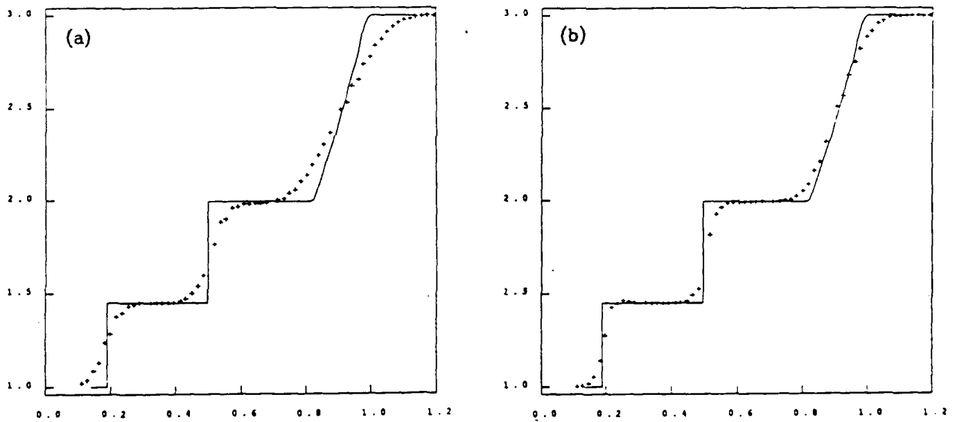
Figure 9.2 Density in the shock tube along the lower wall. Values in the boundary cells are plotted versus arclength. The solid line is the true solution. (a) First order method. (b) With high resolution correction waves included.
