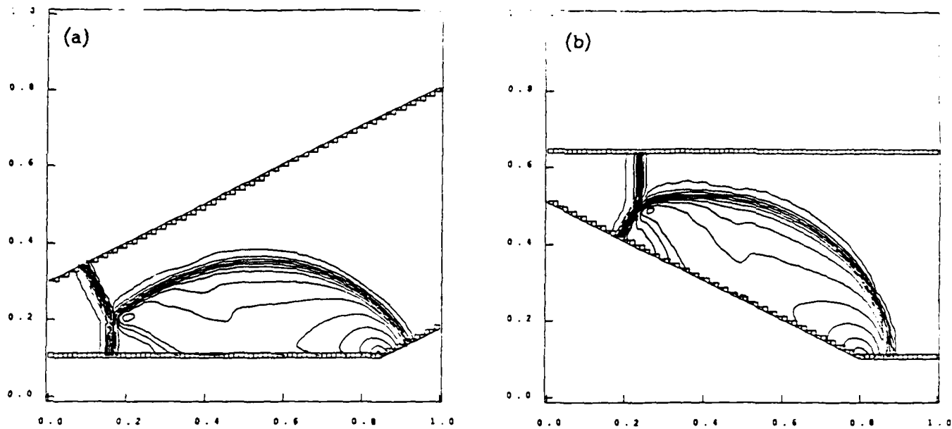
Figure 9.3 Density contours for Mach 2.03 shock reflection off a 27° ramp. (a) Case I: grid aligned with ramp. (b) Case II: grid aligned with incident shock.
