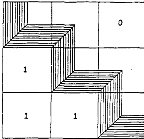
Figure 6.3. Wave propagation for the scalar problem (6.12) when tangential wave propagation is included. Shown for a time step k = h/2 .
