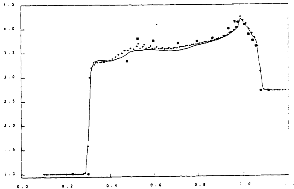
Figure 9.4 Density along the lower boundary. The solid line shows results from Case I, the + symbols are results from Case II. The squares are experimental results taken from [9].
