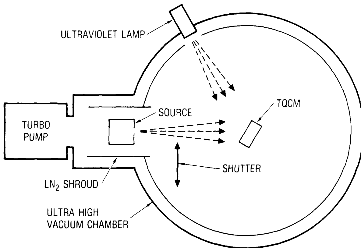
Fig. A-1. Schematic Representation of the Photochemical Deposition Apparatus
