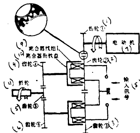
Fig. 2-10. Principle of the electrical steering mechanism.
