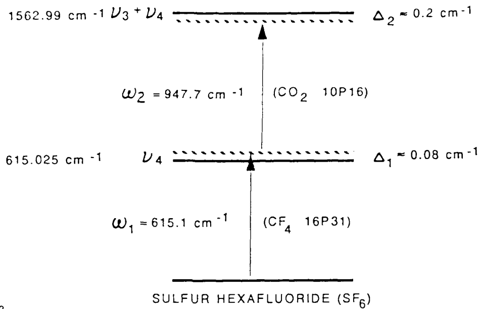
Figure 1. Energy levels and laser lines
