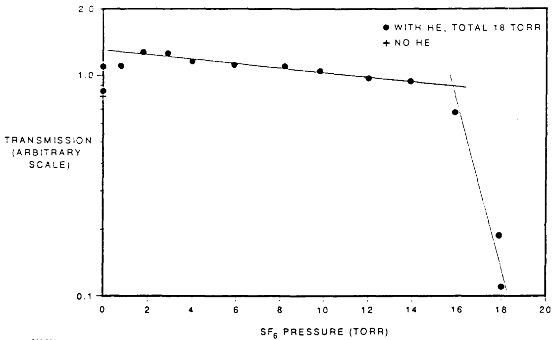
Figure 4. 16.26 μm absorption with helium
