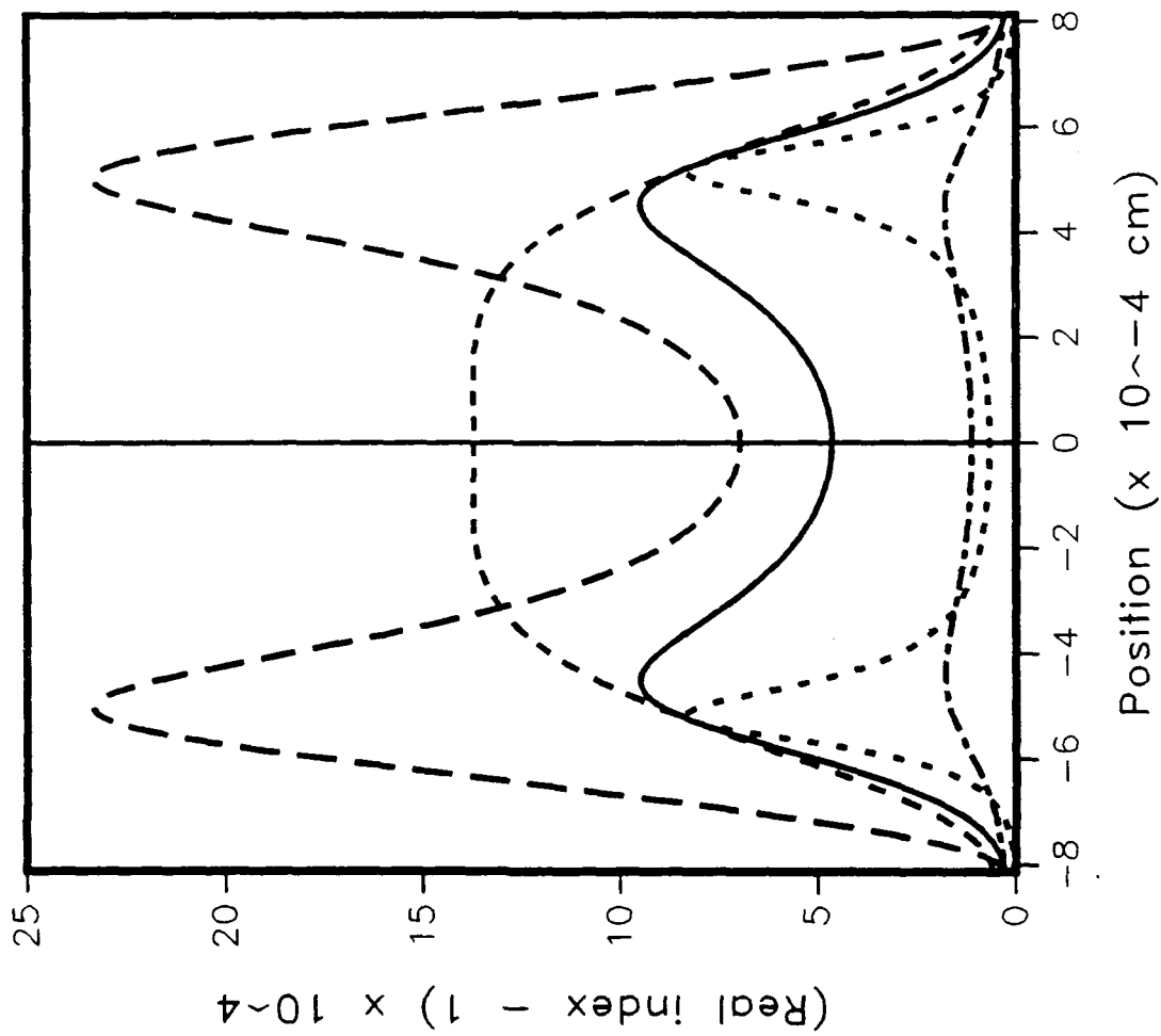
Figure 2.1.7 Effect of field strength on grating profile; SF 6 pressure, 0.1 Torr
