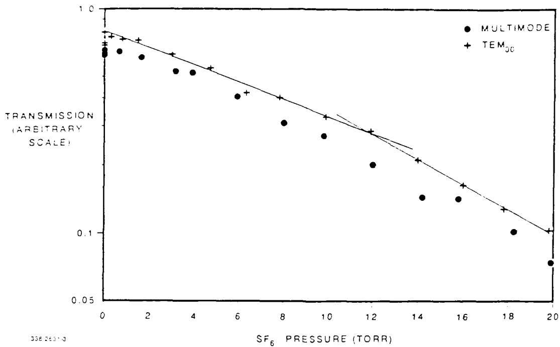
Figure 3. 16.26 μm absorption without helium
