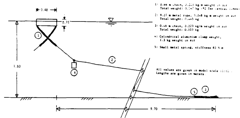
Fig. 2.9 A mooring line of the breakwater model.
