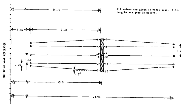
Fig. 2.10 The mooring system of the model, seen from above. The numbers marked at the pontoons denote the force sensors. Thus the corresponding mooring lines are seen on the opposite sides of the pontoons.
