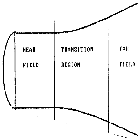
Figure 12: Antenna Regions
