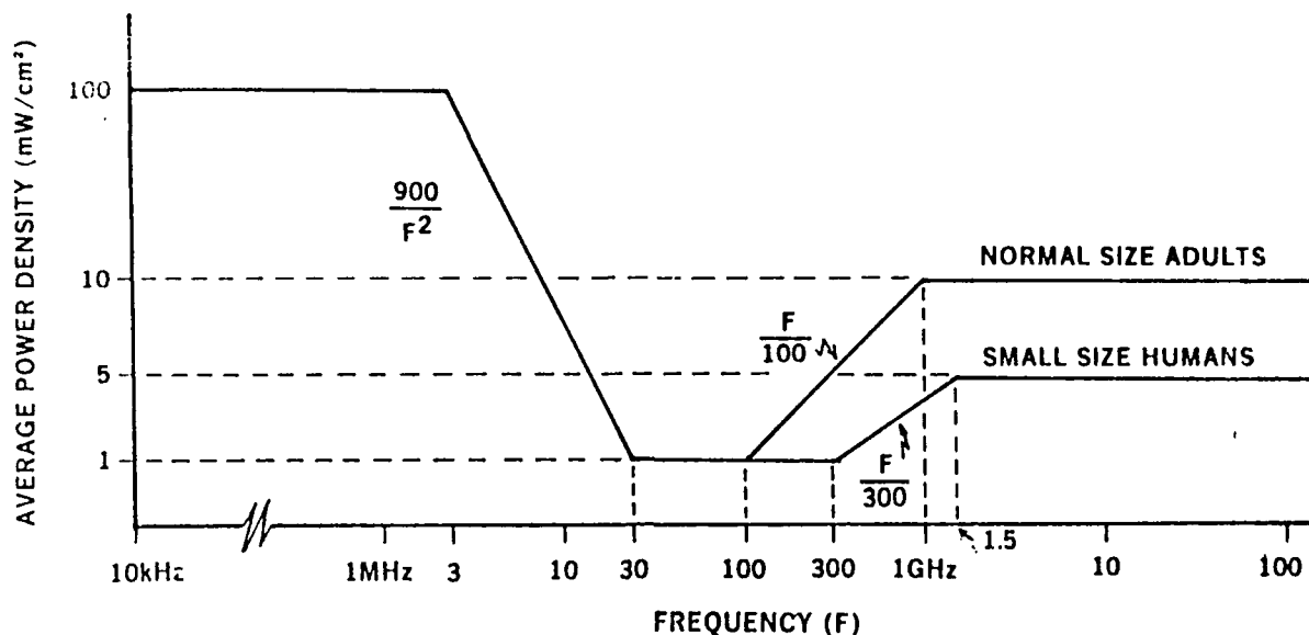
Figure 15: Permissible Exposure Limits
