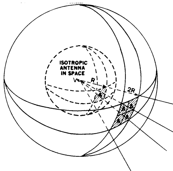
Figure 11: Isotropic Emitter
