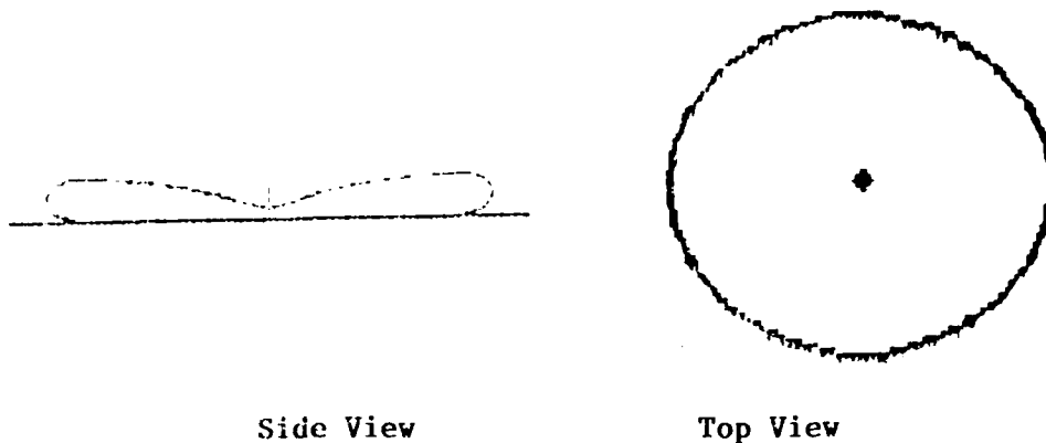
Figure H-2: Radiation Pattern of Monopole Antennas
