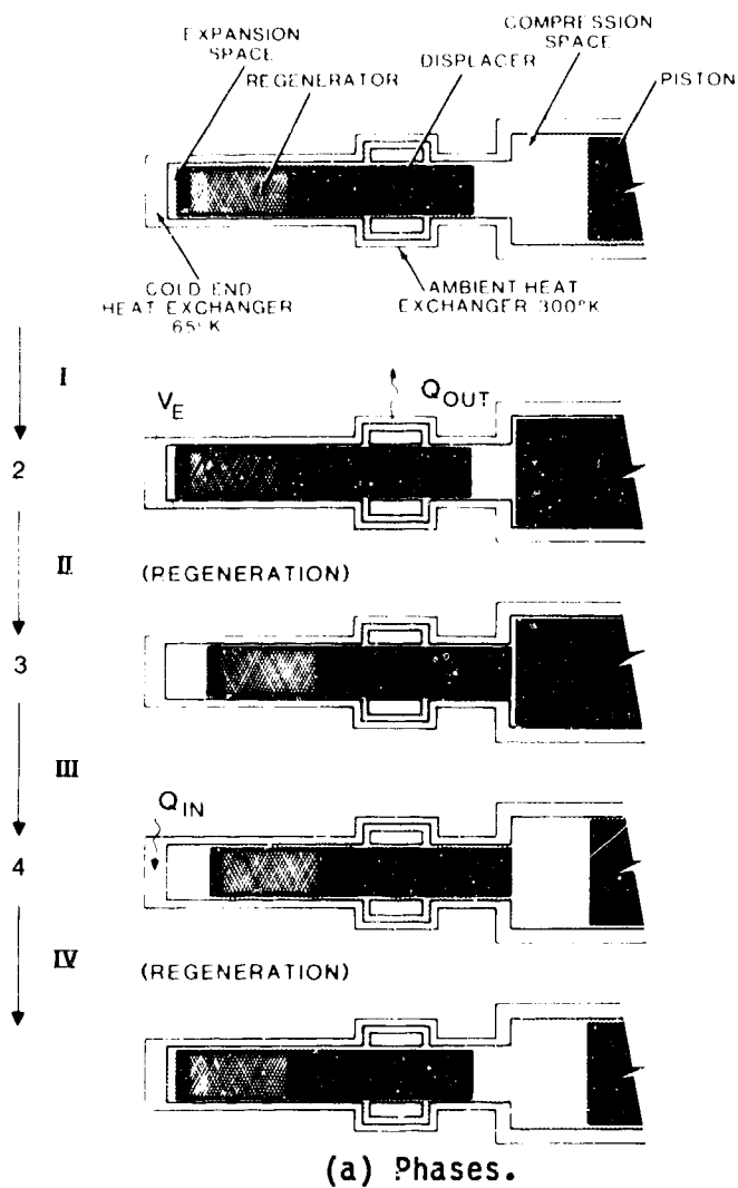
Figure 1. Phases, p-v diagram and volume variations for ideal Stirling cycle.
