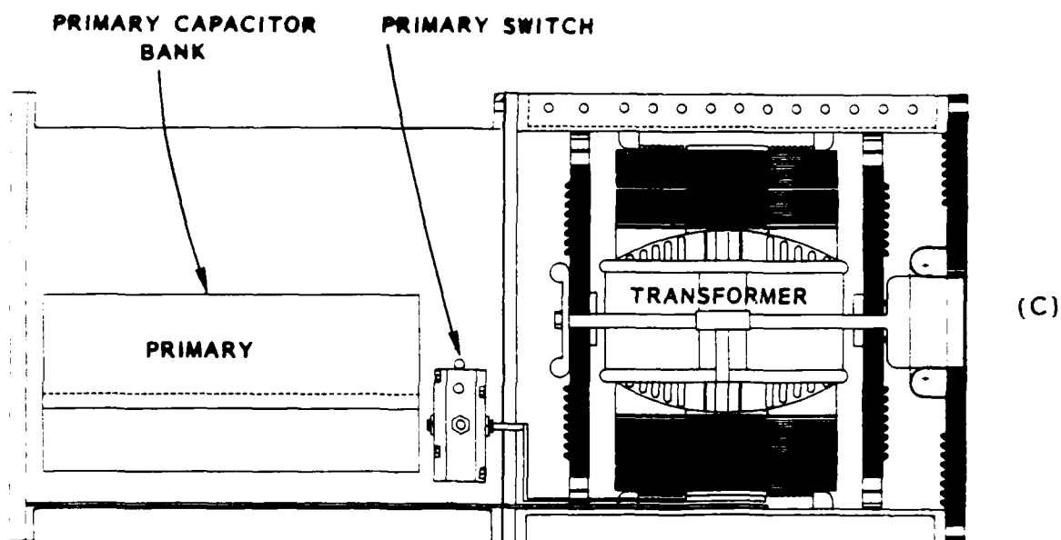
Figure 16. Layout of 3-4 kJ pulser: (A) overall layout (inductors not shown), (B) PFN (inductors not shown), (C) primary circuit and transformer.
