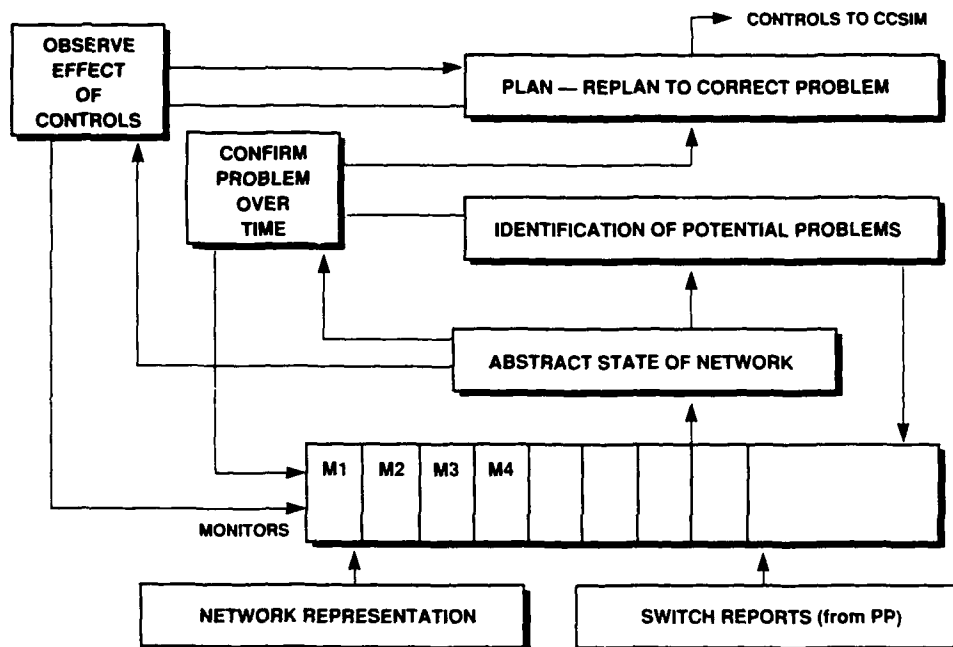
Figure 2-3. Expert system structure.
