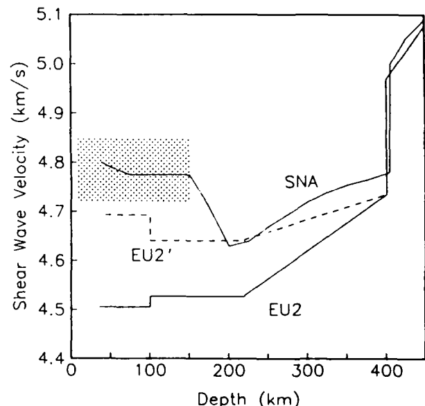
Fig. 1. Shear velocity as a function of depth for continental models EU2 and SNA. Stippling indicates the range of regional Sn velocities typical of continental cratons [Heustis et al., 1973]. The dashed line labeled EU2' is the SH velocity structure corresponding to the RI model in Table 1.
