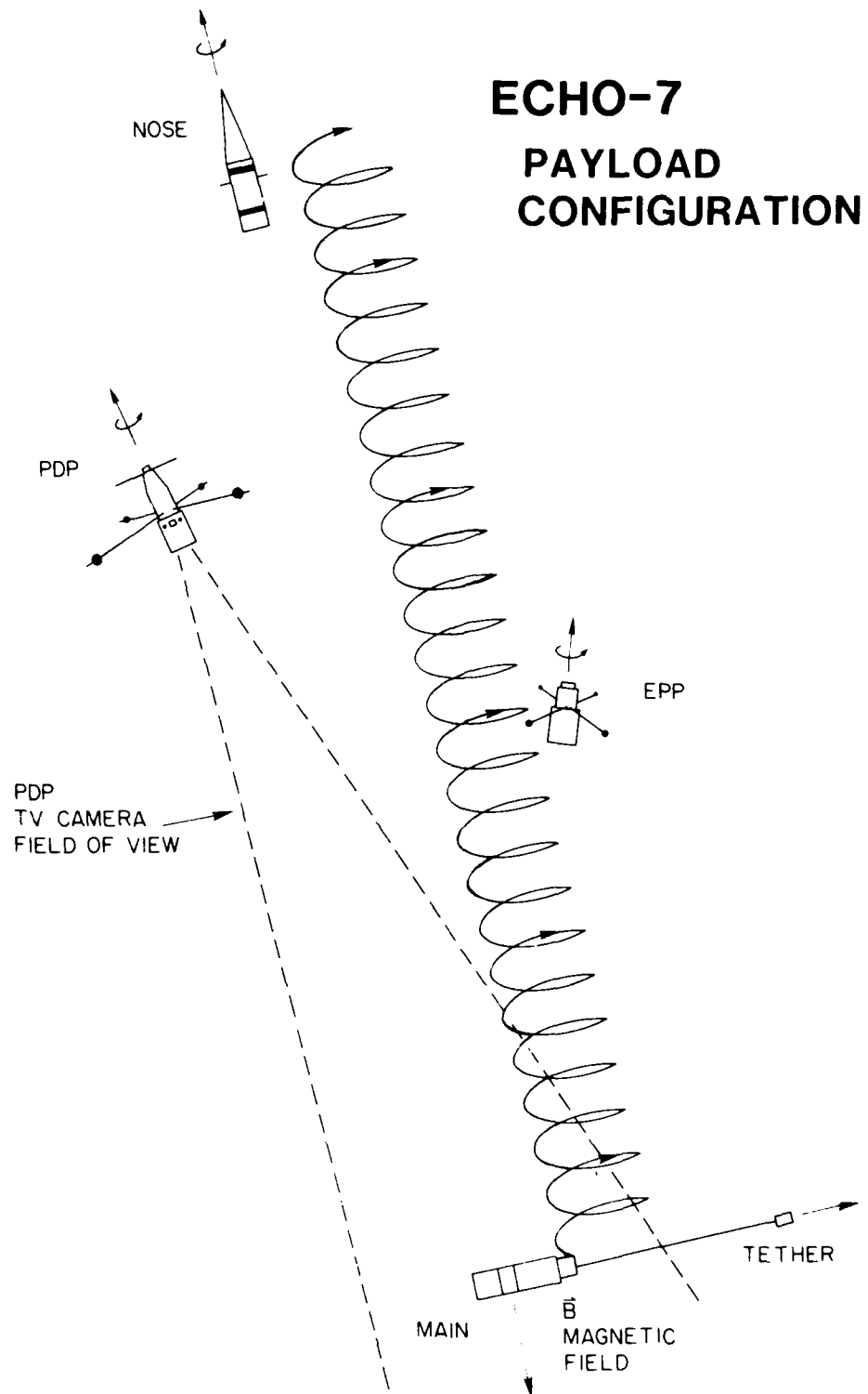
Figure 3. Configuration of the Four Free-Flying ECHO-7 Payloads. NOSE was ejected straight up the magnetic field line, the Plasma Diagnostics Payload 10^\circ to the magnetic south and the Energetic Electron Payload 25^\circ to the magnetic west of the electron beam emitting MAIN payload.
