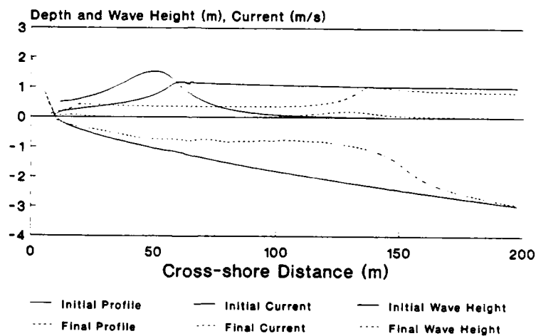
(b) beach profile at initial and final time step and corresponding wave height and longshore current distribution at profile closest to groin
