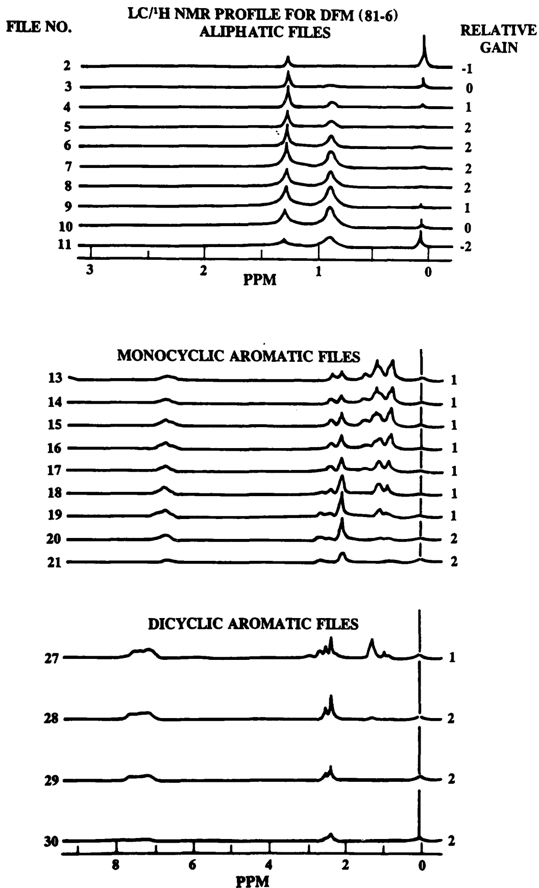
Figure 42. Sample 1 H NMR Spectrum
