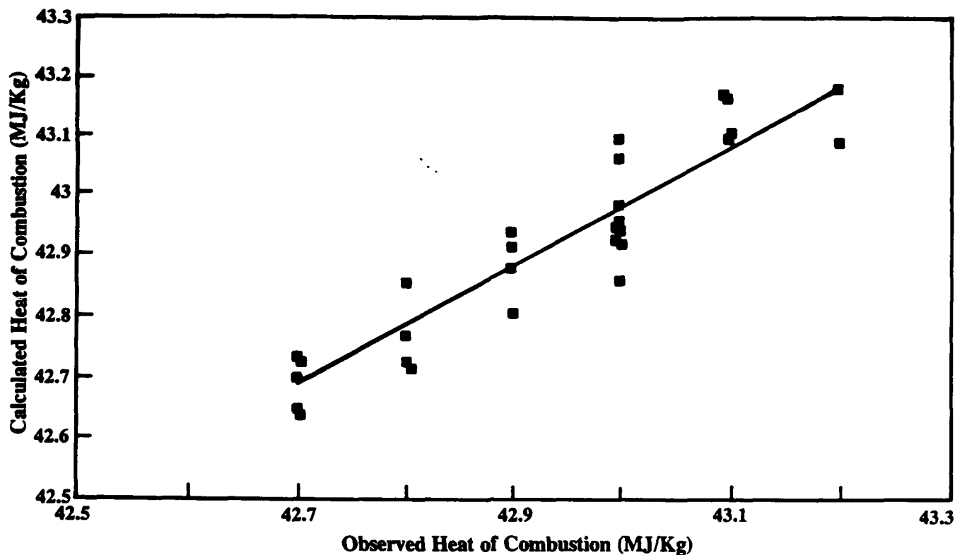
Figure 19. Correlation Plot for Heat of Combustion
