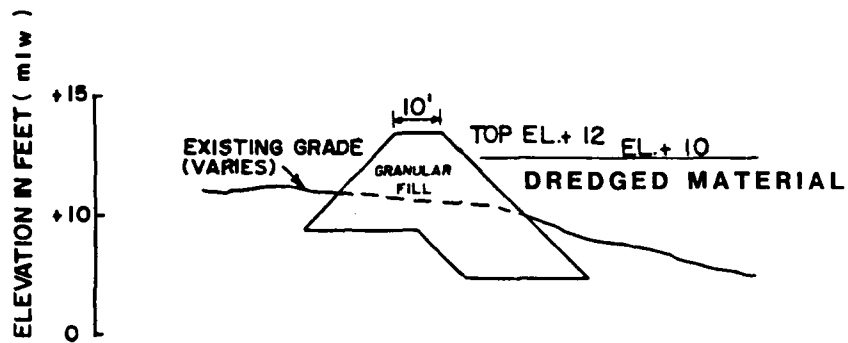
a. Typical land dike (site 1B) - unlined
