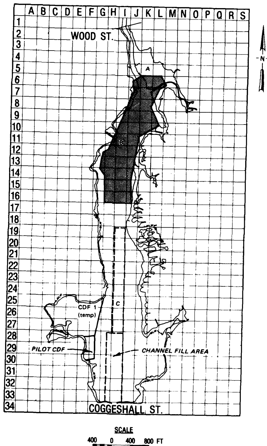
Figure 34. Layout of CDF and CAD sites for CAD option C
