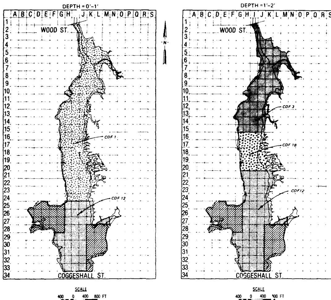
Figure 22. Sediment removal and placement in CDFs for CDF Option B
