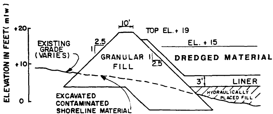
b. Typical land dike (site 1B) - lined
