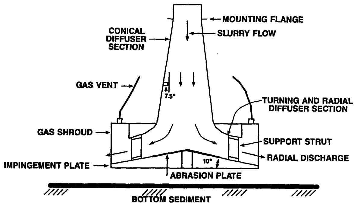
Figure 30. Submerged diffuser
