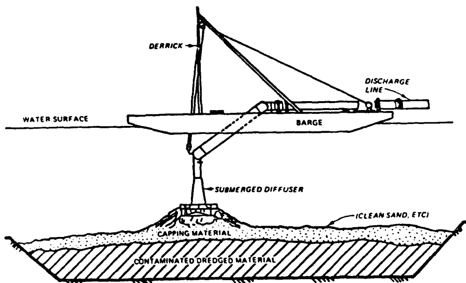
Figure 26. Concept of contained aquatic disposal
