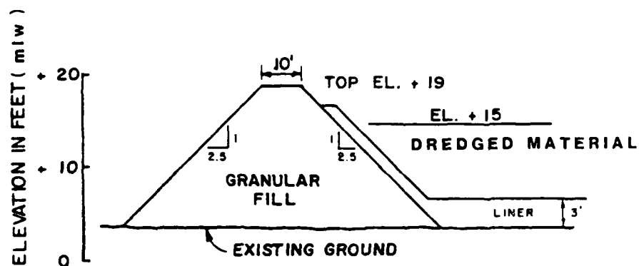
Figure 21. Design features for upland sites 6 and 12
