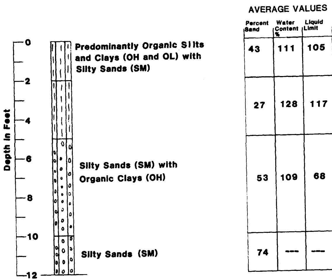
Figure 11. Average physical characteristics of estuary sediment
