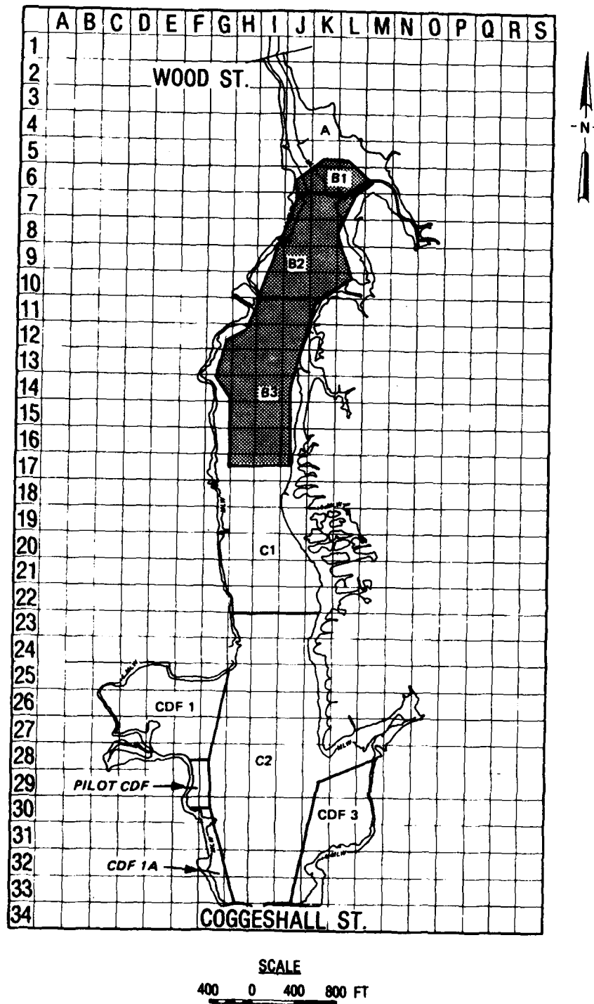
Figure 32. Layout of CDF and CAD sites for CAD option A
