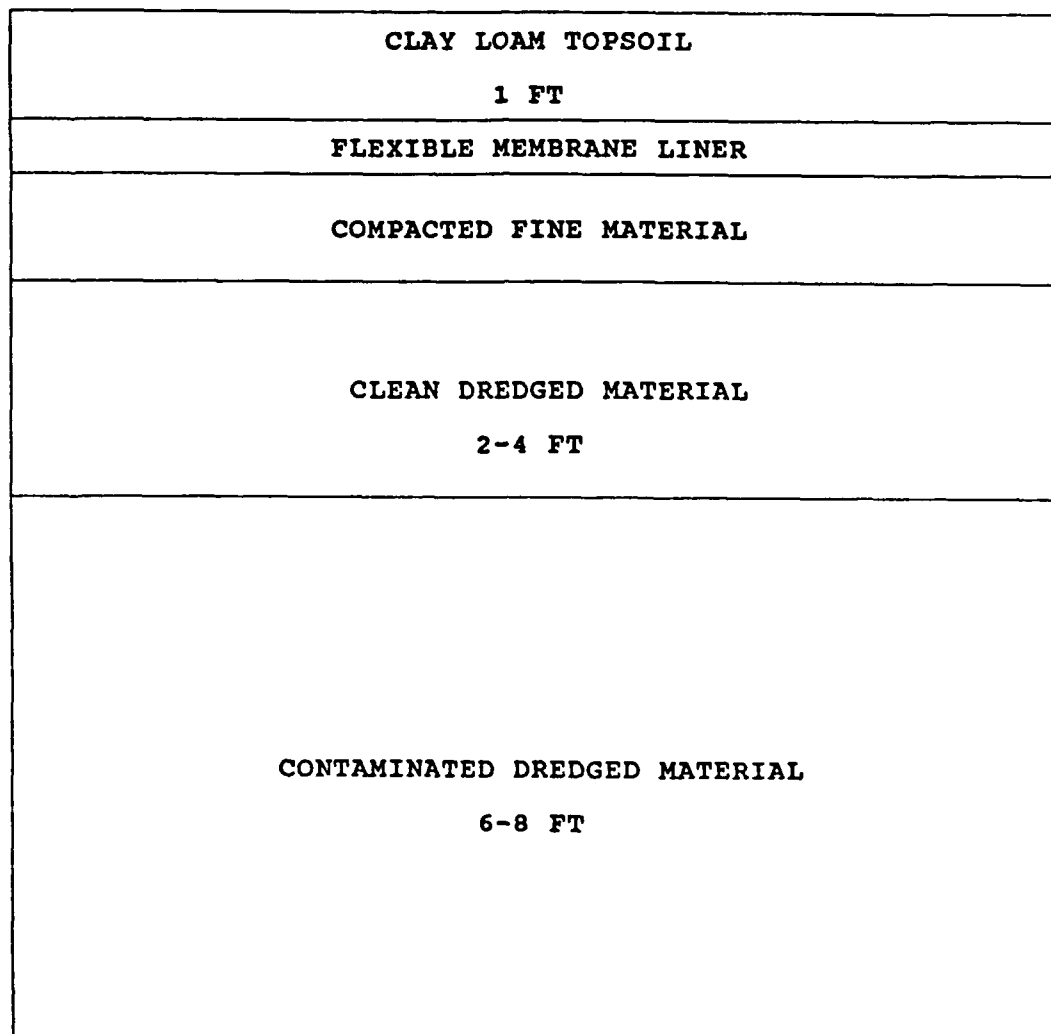
Figure 24. Typical CDF surface cover design
