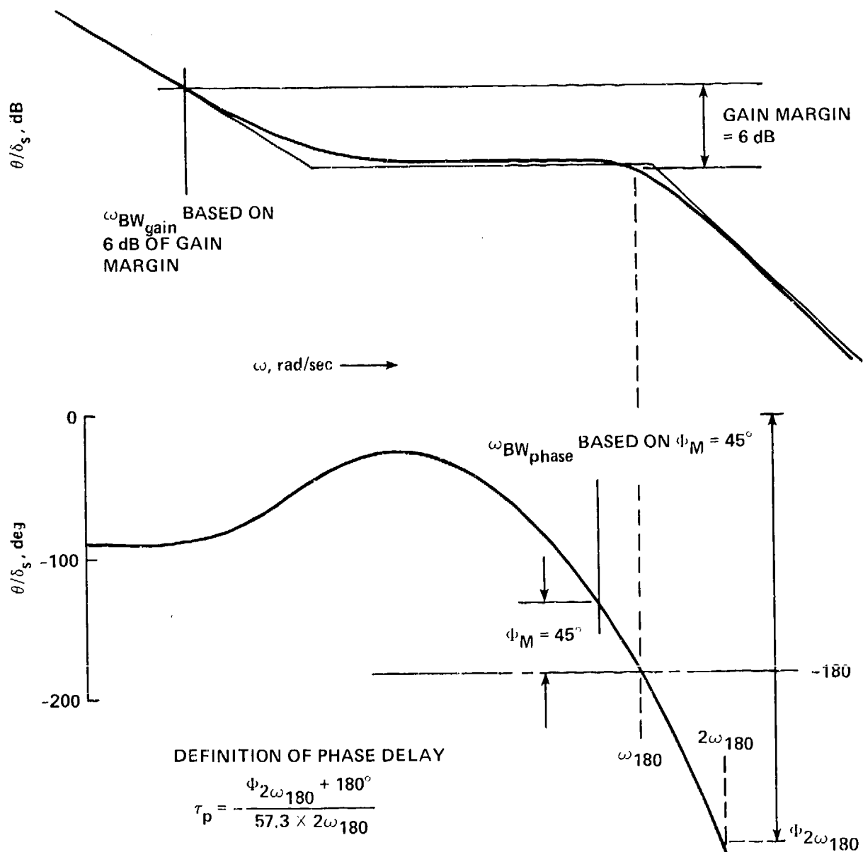
Figure 2.— Definition of bandwidth ( \omega_{BW} ) and phase delay ( \tau_p ). For attitude response type, \omega_{BW} = \omega_{BW_{\text{phase}}} . For rate response type, \omega_{BW} is the lesser of \omega_{BW_{\text{phase}}} and \omega_{BW_{\text{gain}}} .
