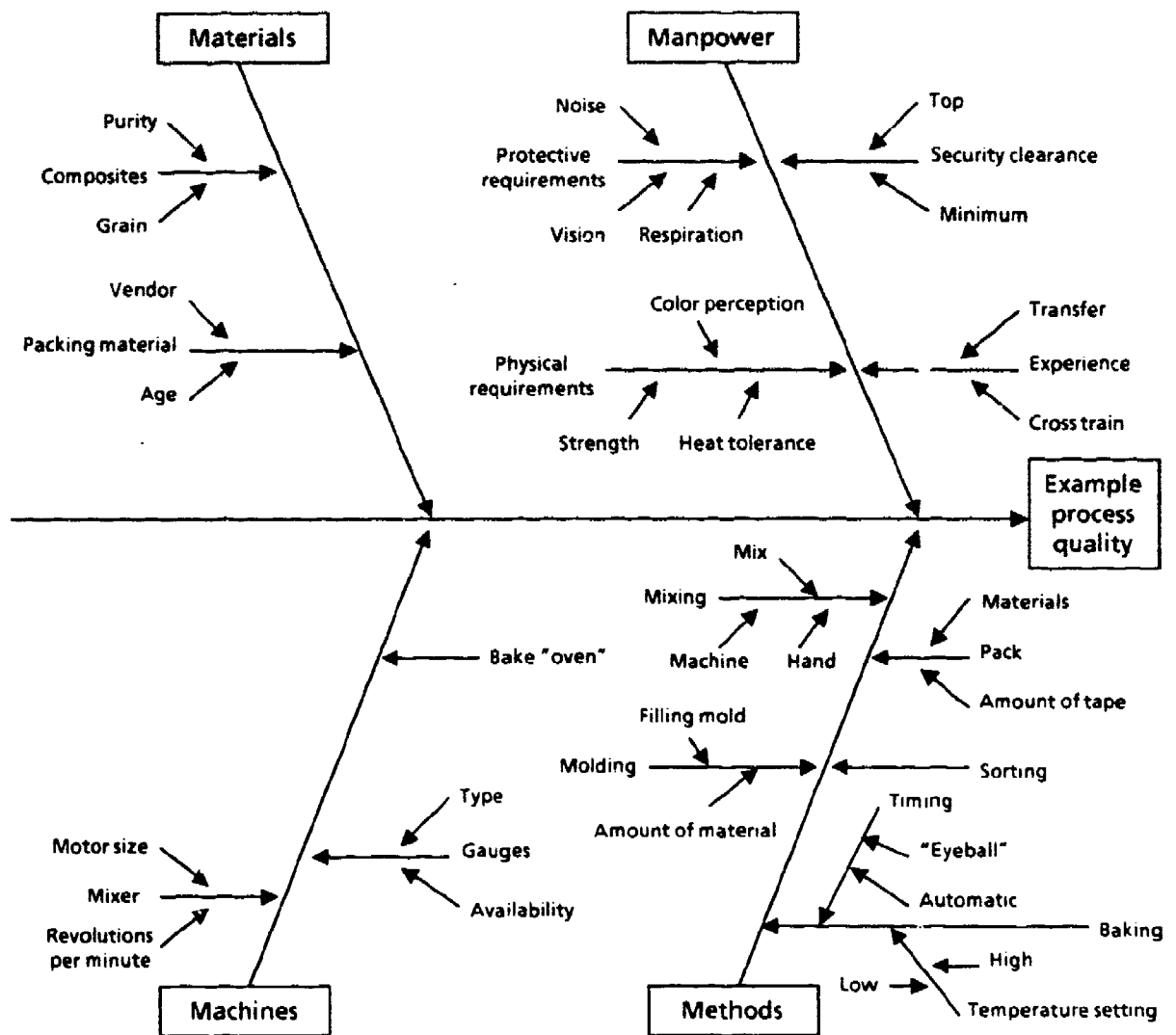
FIG. 4-12. CAUSE-AND-EFFECT DIAGRAM
