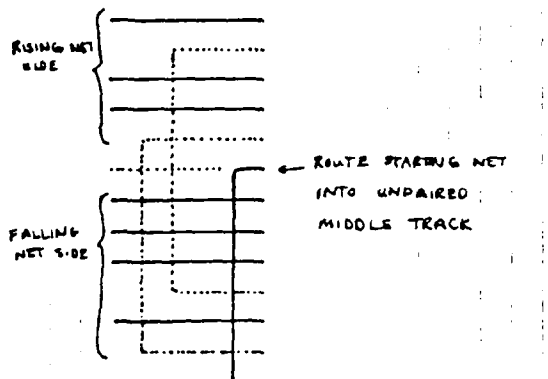
a) CASE 1: STARTING NET, UNPAIRED MIDDLE TRACK.
