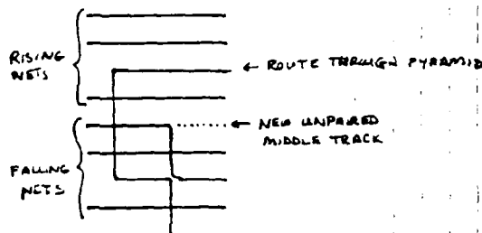
b) CASE 2: STARTING NET, NO UNPAIRED MIDDLE TRACK.
