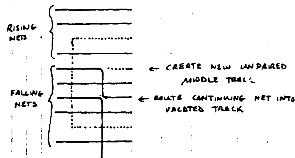
d) CASE 4: ENDING NET, NO UNPAIRED MIDDLE TRACK.
