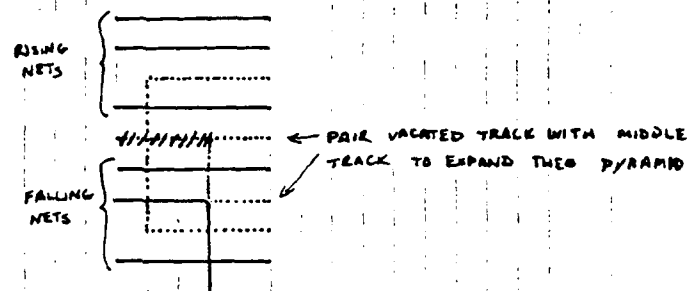
c) CASE 3: ENDING NET, UNPAIRED MIDDLE TRACK.
