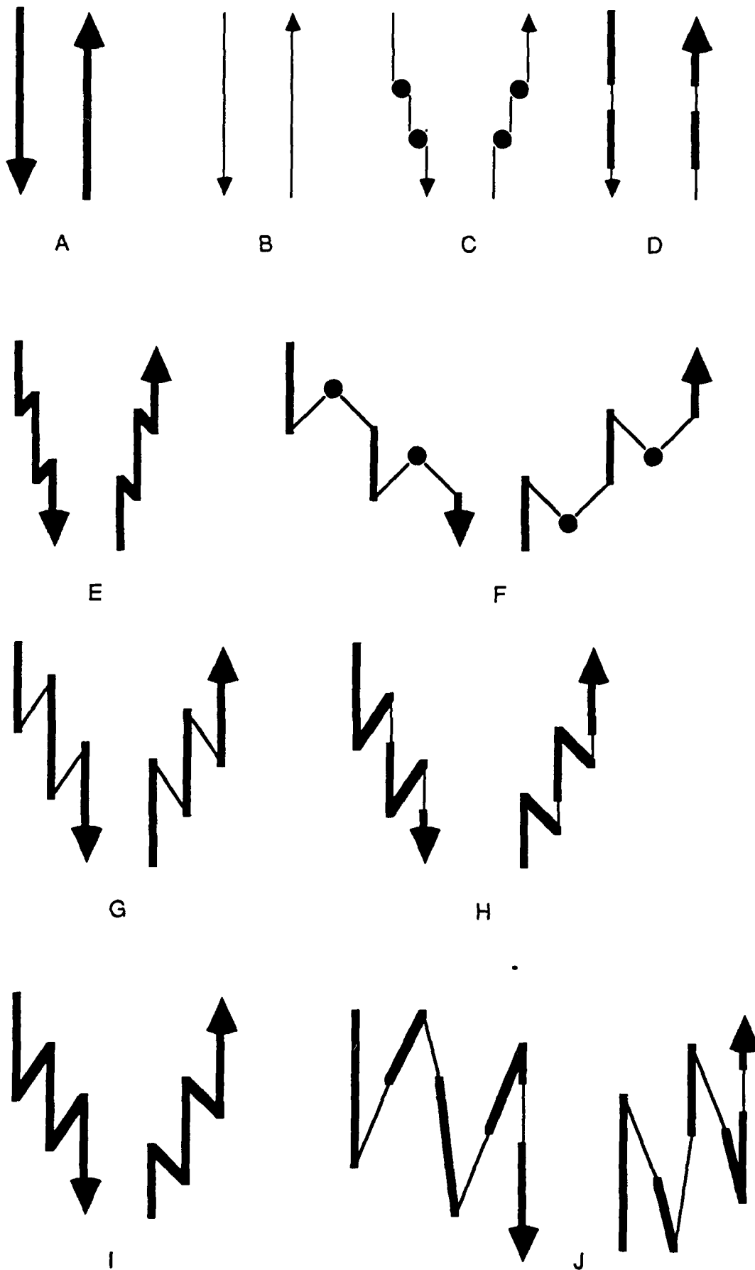
Figure 7: Backtracking Strategies
