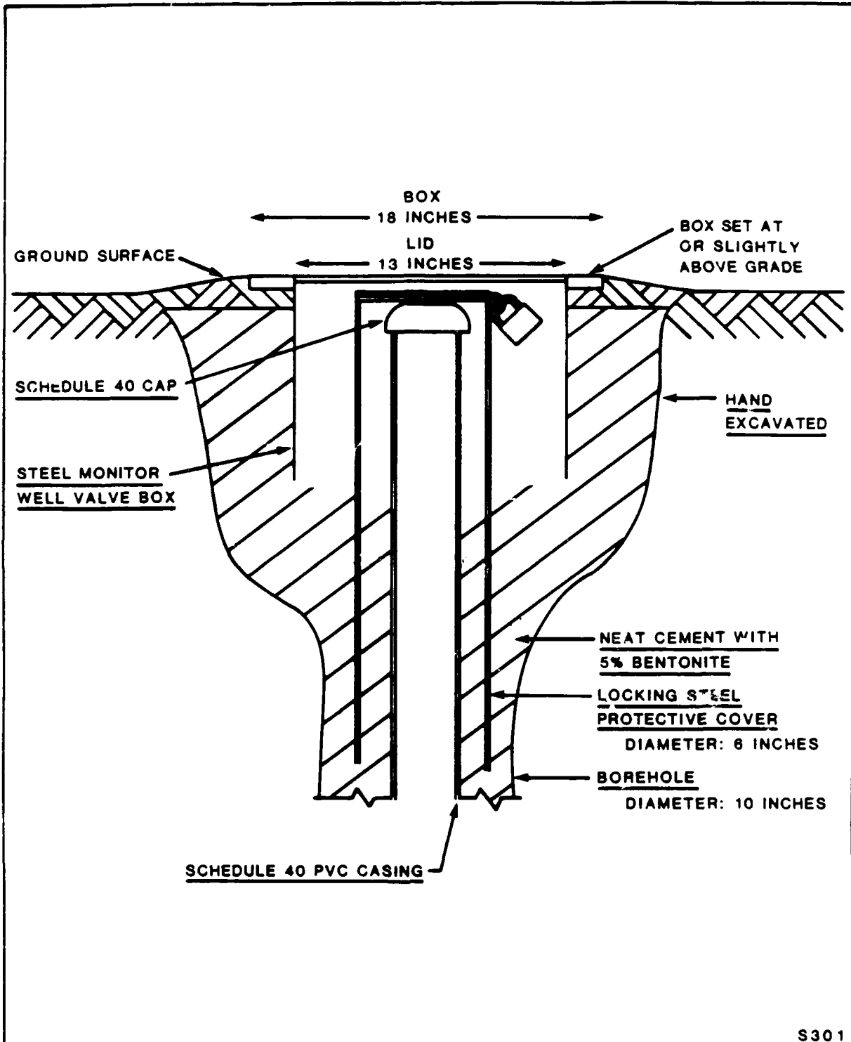
Figure 5-10. Surface Completion for Monitoring Wells.
