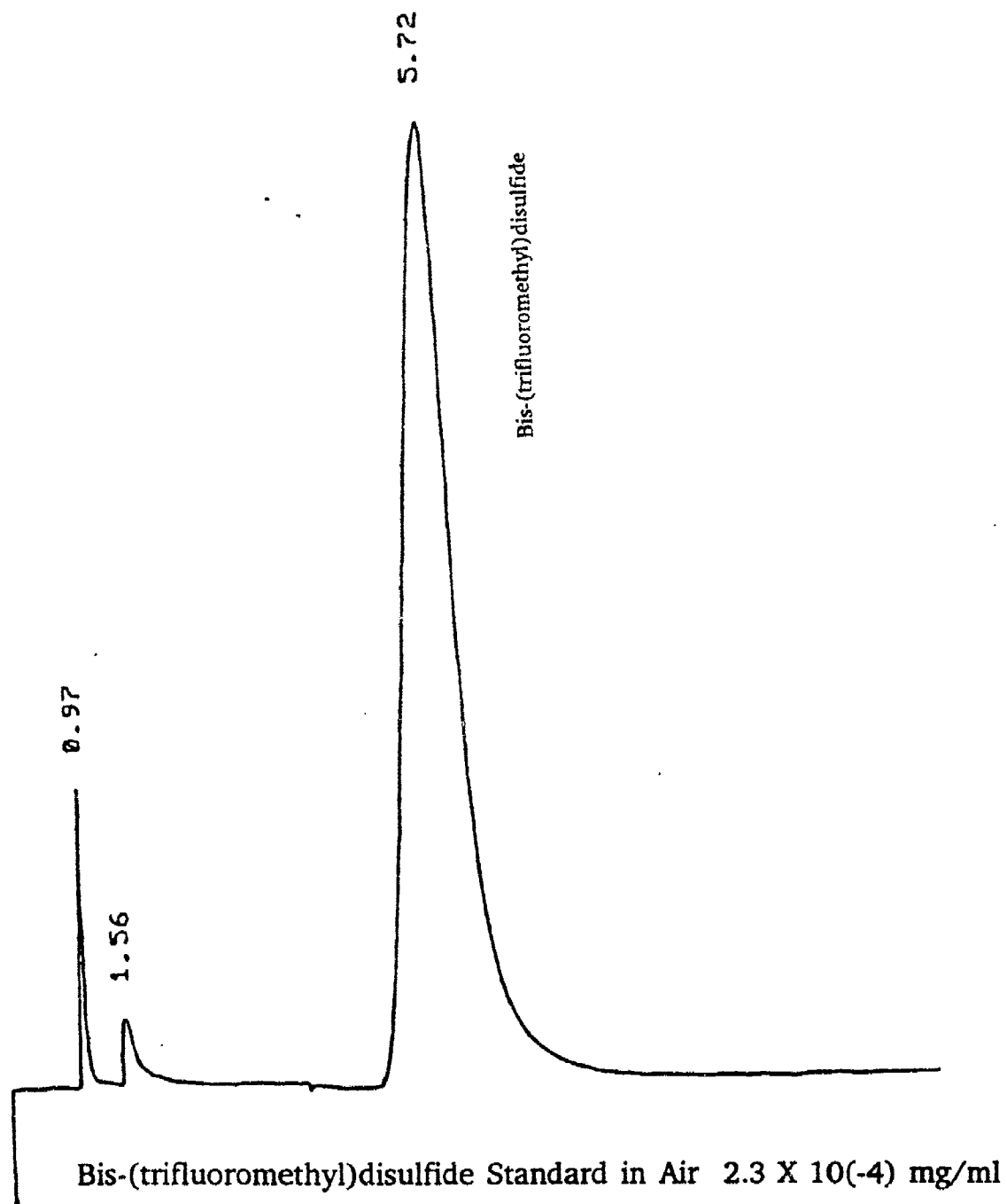
Figure 3. GC/EC Chromatogram of Bis-(trifluoromethyl)disulfide
