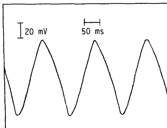
B. Sawtooth Input Current
