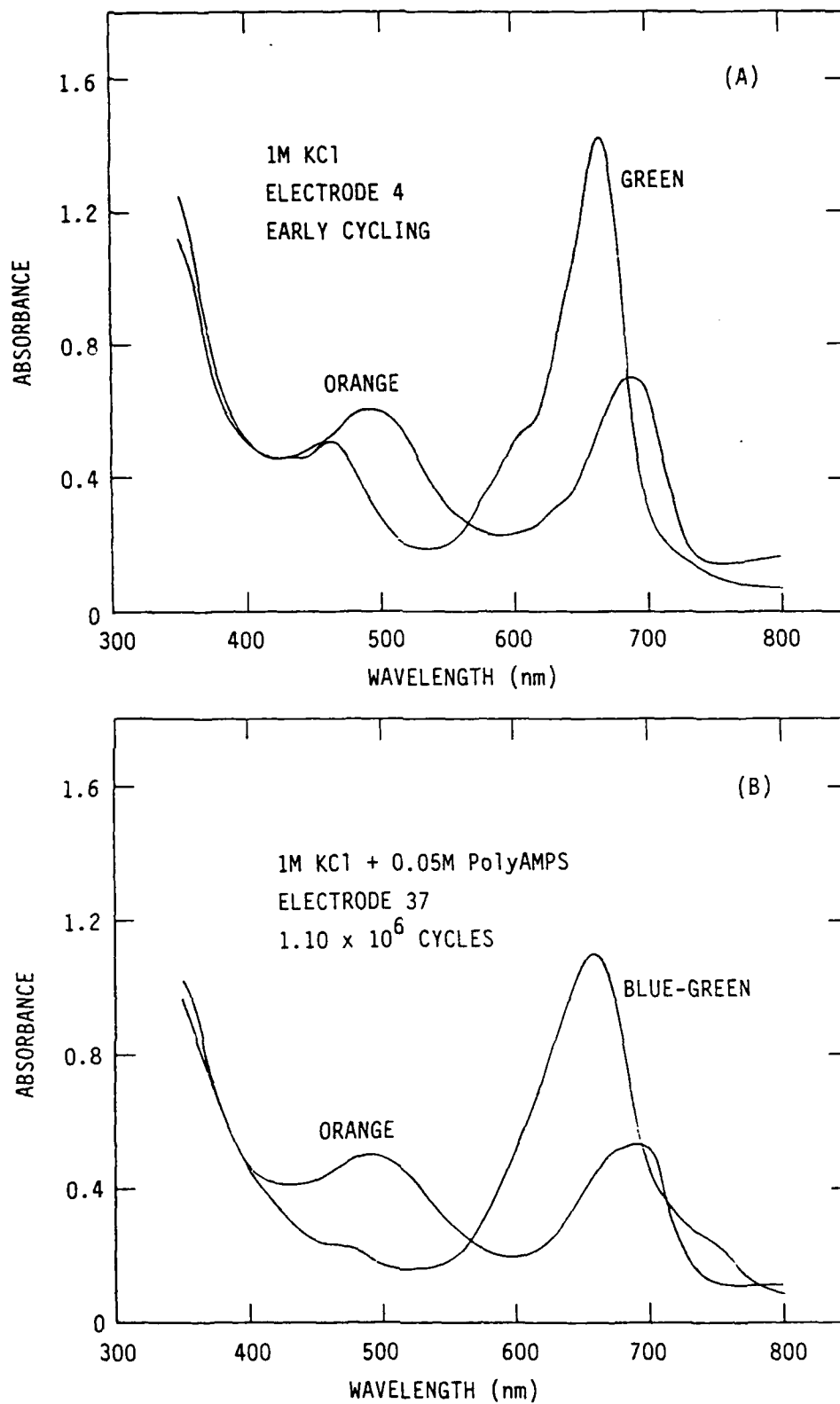
Figure 5. Absorption Spectra at Constant Potentials
