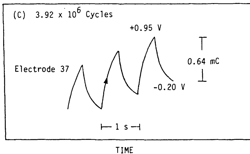
Figure 4. Switching Charge Transients in Early and Later Cycling Stages
