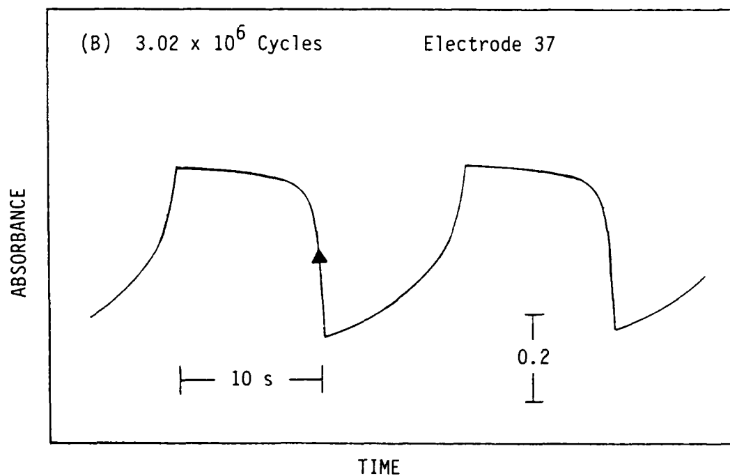
Figure 6. Optical Transients at Different Cycling Stages
