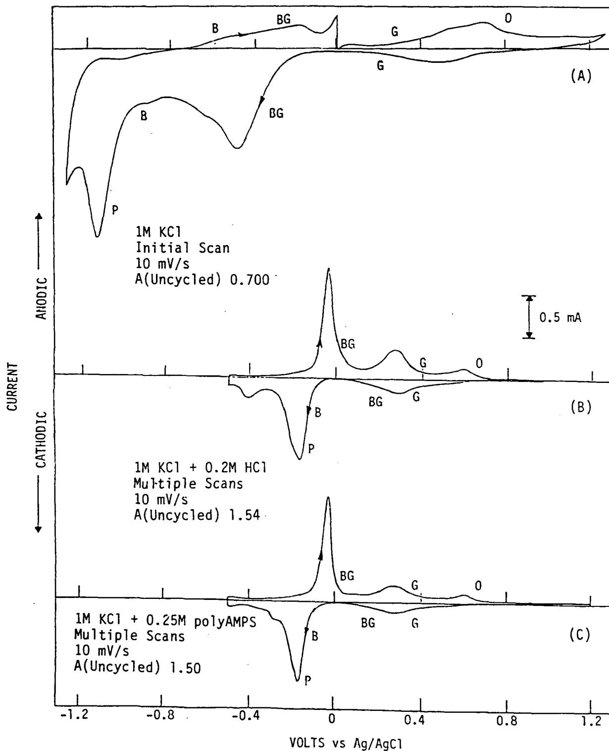
Figure 17. Cyclic Voltammograms for Lutetium Diphthalocyanine Electrodes in Aqueous Chloride Electrolytes
