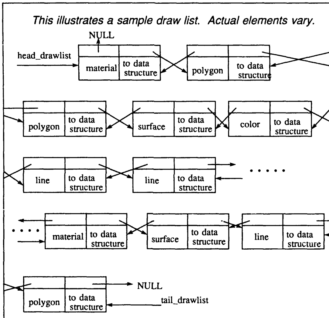
Figure 4.2 Object Draw List Illustrated
