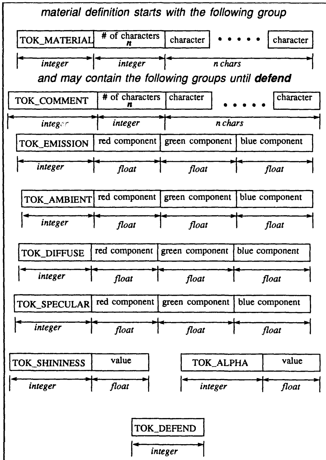
Figure 3.4 Material Definition Storage
