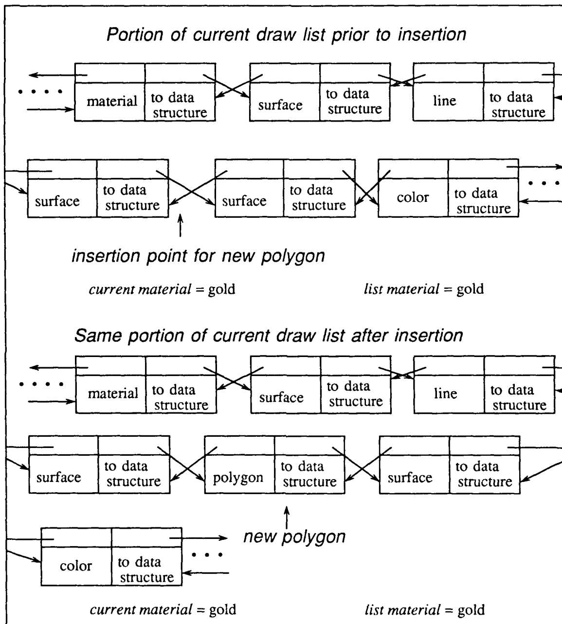
Figure 6.1 Node Insertion with Same Material Illustrated
