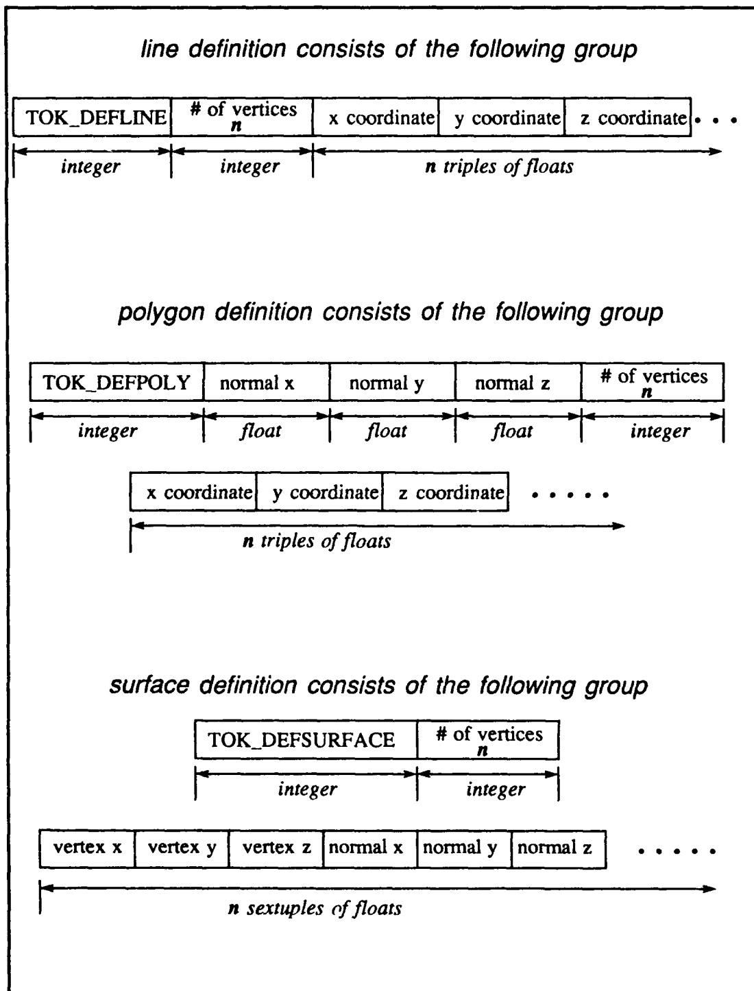
Figure 3.6 Line, Polygon and Surface Storage
