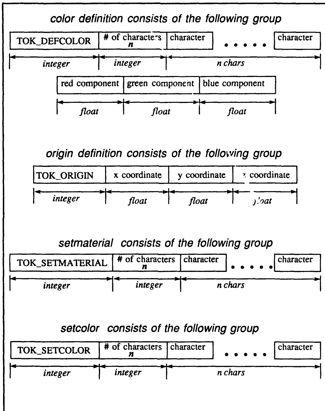
Figure 3.5 Storage of Defcolor, Origin, Setmaterial, Setcolor
