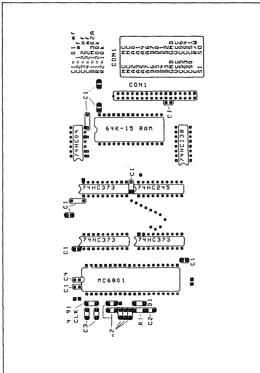
Figure 26 Main Computer Board (Component Layout)
