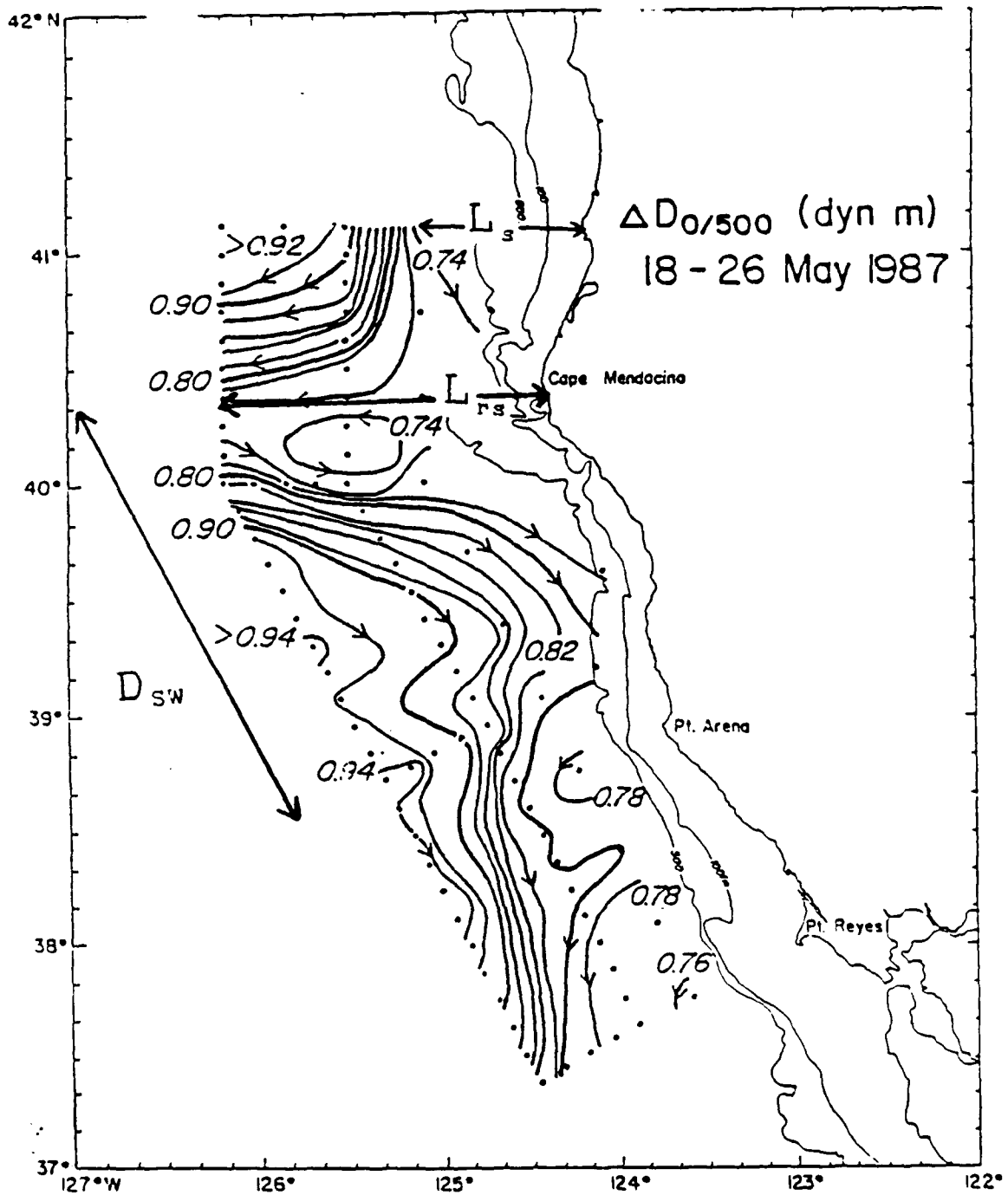
Figure 3.2 Map of dynamic height of the sea surface relative to 500db for the May 1987 data. This shows measures for L_s , L_{rs} , and D_{sw} . [From "OSU Data Report for CTD Observations in the Coastal Transition Zone Off Northern California, 18-26 May 1987".]
