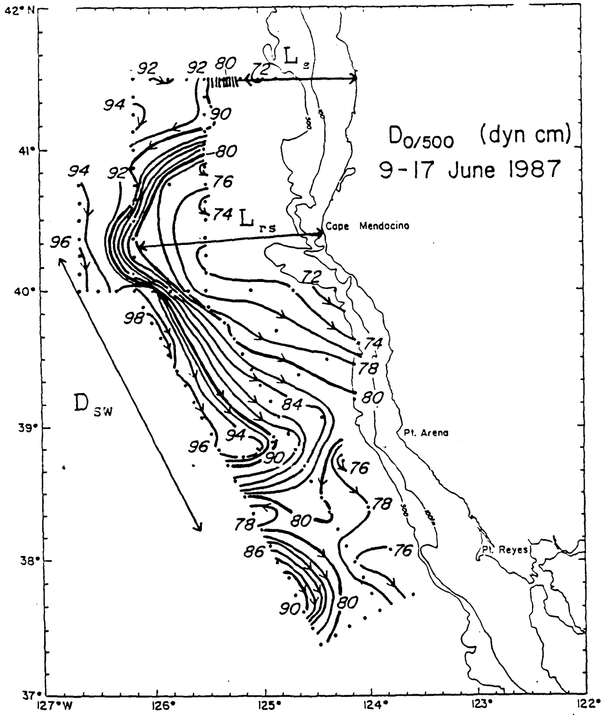
Figure 3.3 Map of dynamic height of the sea surface relative to 500 db for the June 1987 data. This shows the measurements for L_s , L_m , and D_{sw} . [From "OSU Data Report for CTD Observations in the Coastal Transition Zone Off Northern California, 9-18 June 1987".]
