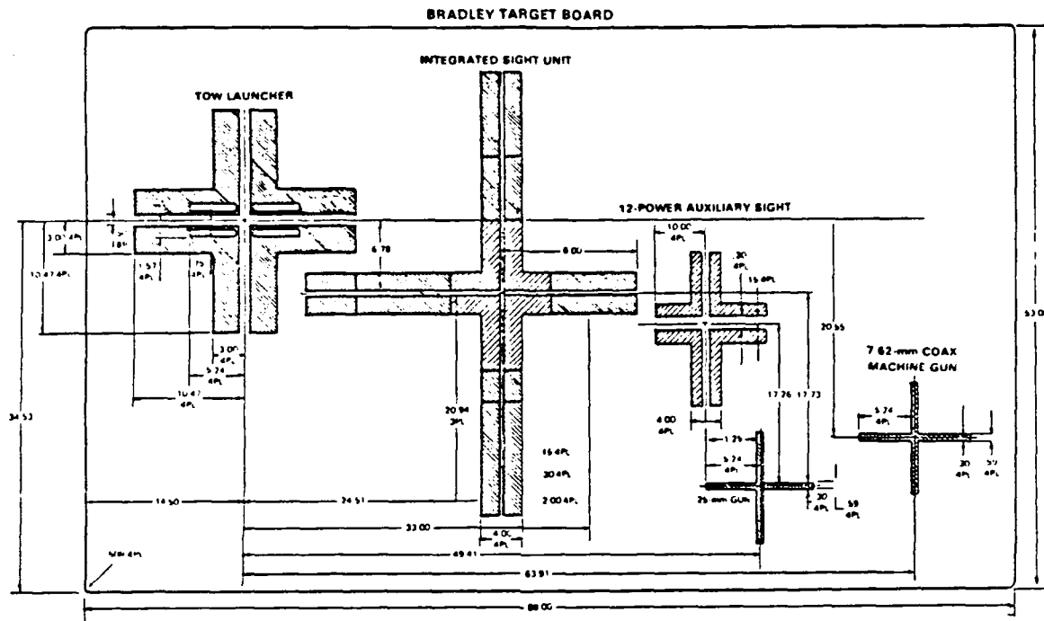
Figure 7. The close-in boresight panel (FM 23-1, 1986).
