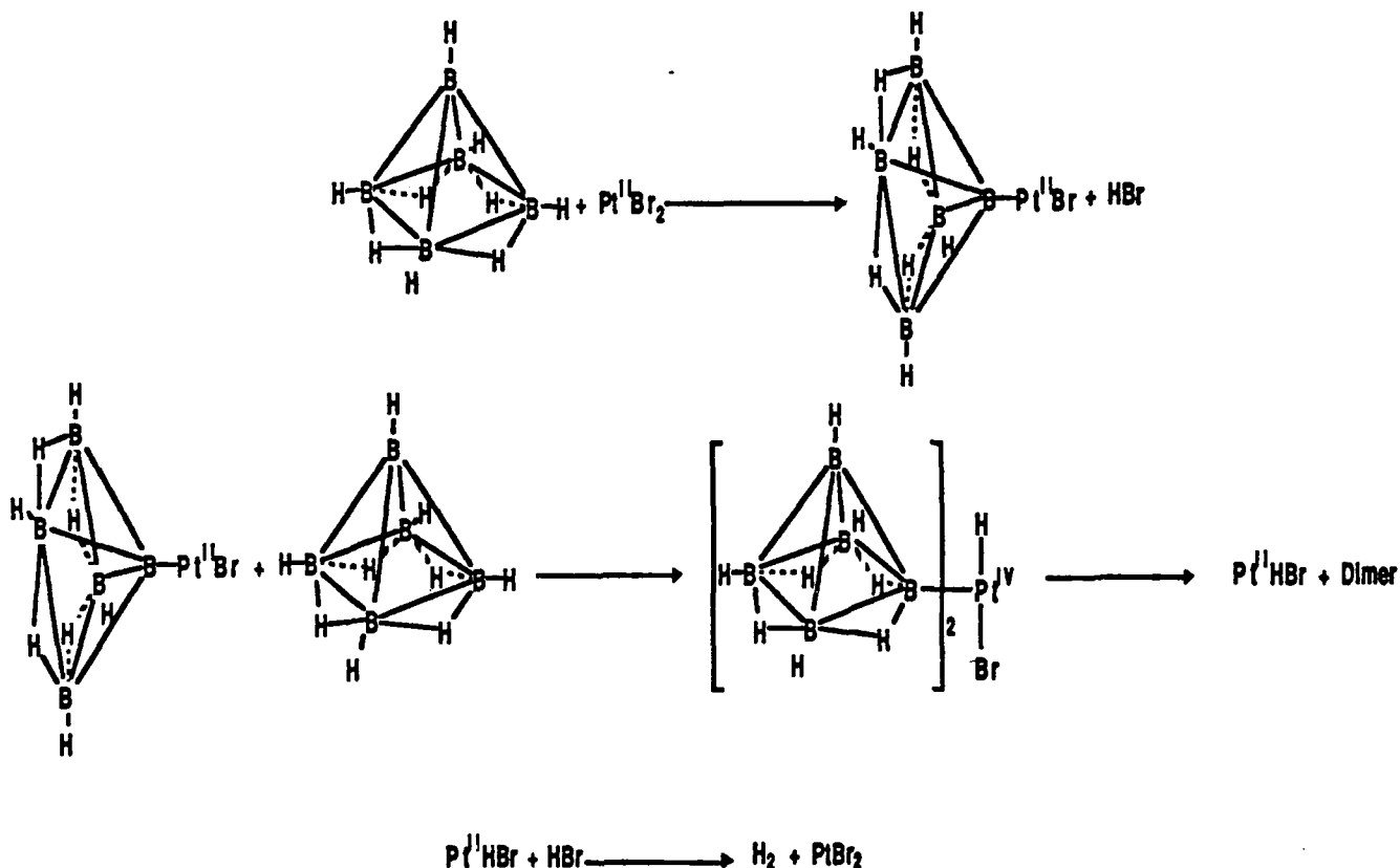
If the apical site is blocked with a methyl group, no reaction occurs. This, coupled with the exclusive formation of the 1:2'-[B 5 H 8 ] 2 isomer, is consistent with a mechanism where oxidative addition occurs only at the apical site. These results are also consistent with earlier work on transition metal
