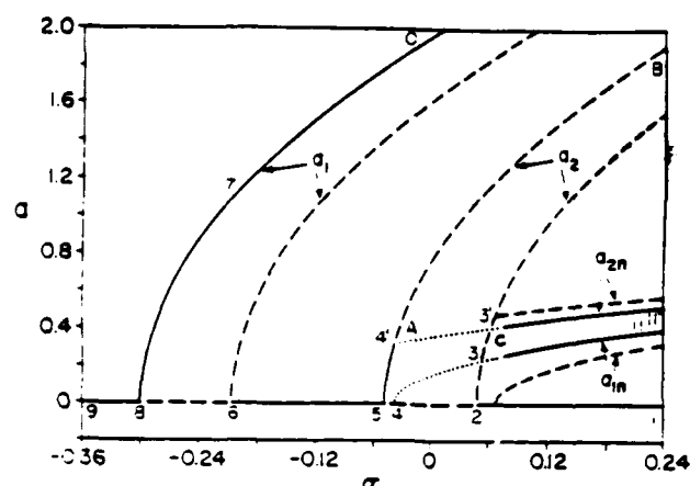
Figure 5. Response curves of the first mode for a beam with an aspect ratio \hat{b}/h \approx 1.0 : mode (1,1), \omega_{11} = \omega_{21} , \delta_0 = 0.0 , \delta_2 = -0.5 , \mu = 0.05 , b = 0.03 , \beta_1 = 0.7692 .
