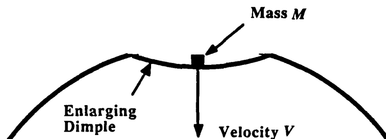
Figure 1 – Spherical shell impacted by mass M . For large amplitude displacement an effective approximation is that an inverted dimple forms. The significant strain energy is in the localized bending at the edge of the dimple which provides the effect of a nonlinear spring.
