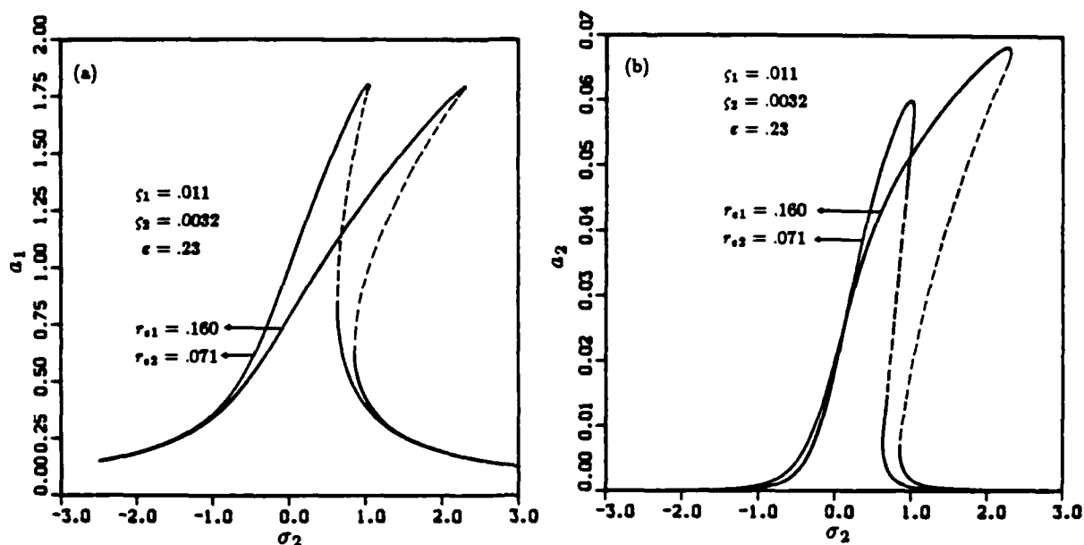
Fig. 3 The variation of response amplitude a , as a function of detuning parameter \sigma_2 , with asymptote d ( M_H = 37.27 Slugs, k = 4,658 lb f /Ft, r_{MB} = 8.44 , r_{MD} = 0.3 , eccentricity \epsilon = 0.008 Ft, d_1 = 0.02 Ft, d_2 = 0.03 Ft). (a), (b) Internal resonance condition with \Omega = \omega_1 when \omega_2 = 3\omega_1 .
