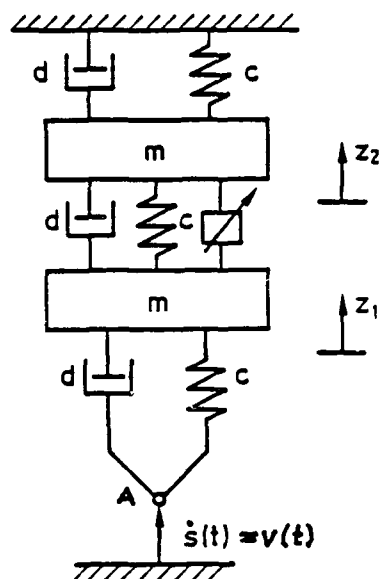
Fig.3: Nonlinear system with two degrees of freedom
