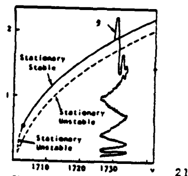
Fig. 5.15. Combination Resonance \nu = 2\nu_2 + \nu_3 , Table 5.4.
