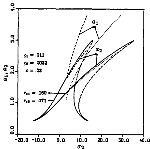
Fig. 4 The variation of response amplitude a , as a function of detuning parameter \sigma_2 , with asymptote d ( M_H = 37.27 Slugs, k = 4,658 lb f /Ft, r_{MB} = 8.44 , r_{MD} = 0.3 , eccentricity \epsilon = 0.008 Ft, d_1 = 0.02 Ft, d_2 = 0.03 Ft). Internal resonance condition with \Omega = \omega_2 when \omega_2 = 3\omega_1 . — a_1 = 0, a_2 \neq 0 with r_{e1} = 0.16 and r_{e2} = 0.071 , - - - a_1 \neq 0, a_2 \neq 0 with r_{e2} = 0.071 , ... a_1 \neq 0, a_2 \neq 0 with r_{e1} = 0.16 .
