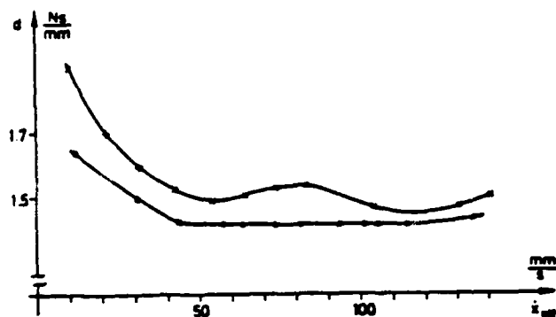
Fig.3 Equivalent damping rates for harmonic signals ( f=2 Hz (x) and f=6 Hz (O)).
