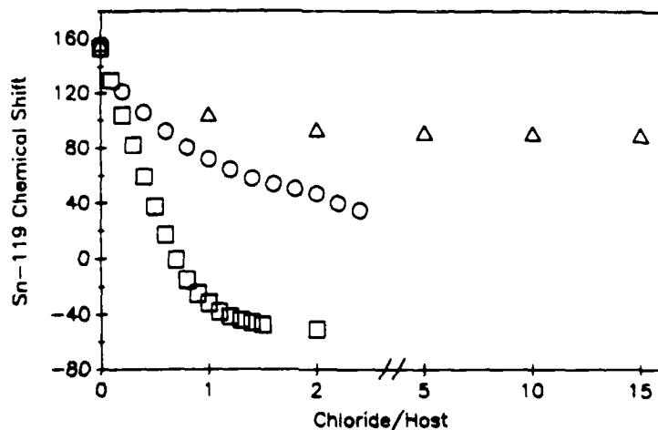
Figure. Titration Curves for \text{Bu}_3\text{SnCl} ( \square ), bicycle 2 ( n = 12 ) ( \circ ), and host 7 ( \triangle ) in \text{CDCl}_3 .
