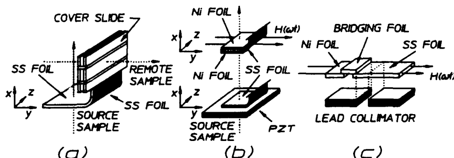
FIG. 1. Schematic representation of the mounting arrangements used in the excitation of sidebands on the Mössbauer absorption line of ^{57}\text{Fe} in the 2.5\text{-}\mu\text{m} -thick stainless-steel (SS) foil. (a) The optical path from \gamma source to detector is shown by the dotted arrow for the orthogonal x and y directions arranged to sample sideband development at the source of the phenomenon and at a remote point, respectively, as marked. Excitation is injected into the horizontal face of the SS foil and the vertical face is mechanically stabilized by the 100\text{-}\mu\text{m} -thick glass cover slides sandwiching the absorber foil. (b) Upper: spin waves injected by the periodic oscillation of the Ni foils pressed onto the absorber foil by additional cover slides not shown and excited by the magnetic field in an inductor containing the Ni foils. The vertical section protrudes from the coil between windings. Lower: vibrational excitation injected by the X -cut quartz-crystal transducer connected to a radio-frequency oscillator. (c) Geometry used in the experiments designed to bridge a break in the conductive path with 25\text{-}\mu\text{m} -thick foils of various materials.
