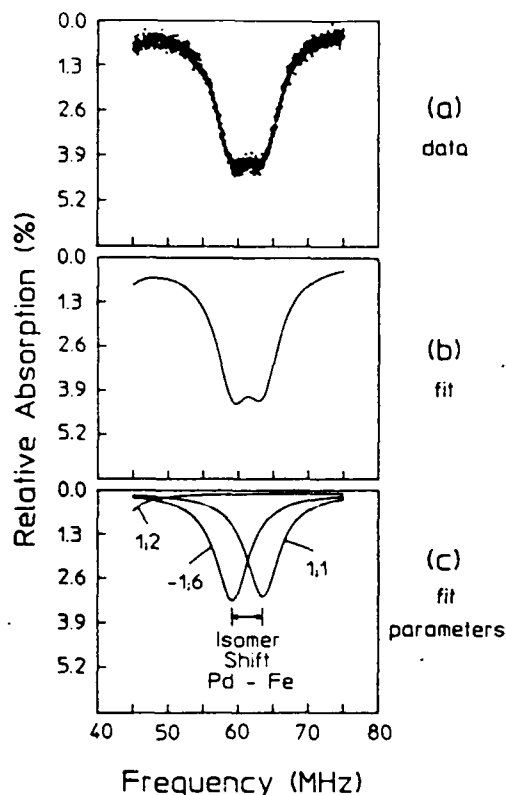
FIG. 3. (a) FMS spectrum of the same enriched foil. The two peaks represent sidebands +1;1 and -1;6. The separation of these peaks is equal to twice the isomer shift of an iron foil relative to a ^{57}\text{Co} source in Pd. (b) Spectrum constructed from fitting the data of Fig. (a) using the Levenberg-Marquardt method for a nonlinear least-squares fit. (c) Spectral components resulting from the fitting procedure shown before summation.
