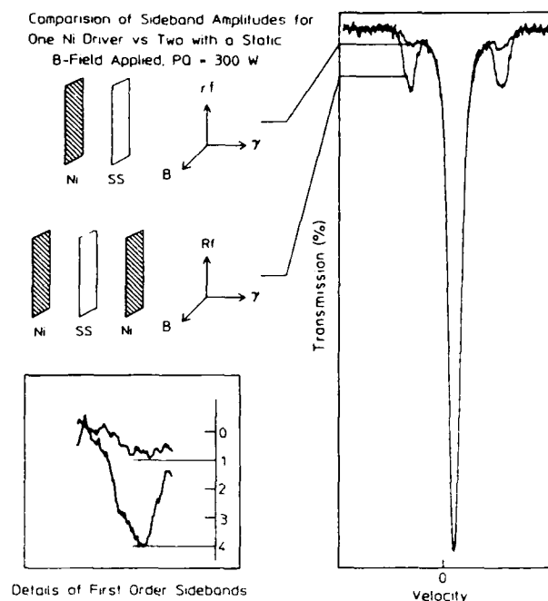
FIG. 5. Comparison of sideband amplitudes for one driver foil vs two when both are biased by a static B field with PQ = 300 W. Here two foils give four times the effect of one thus giving a modulation index of 4m^2 .
