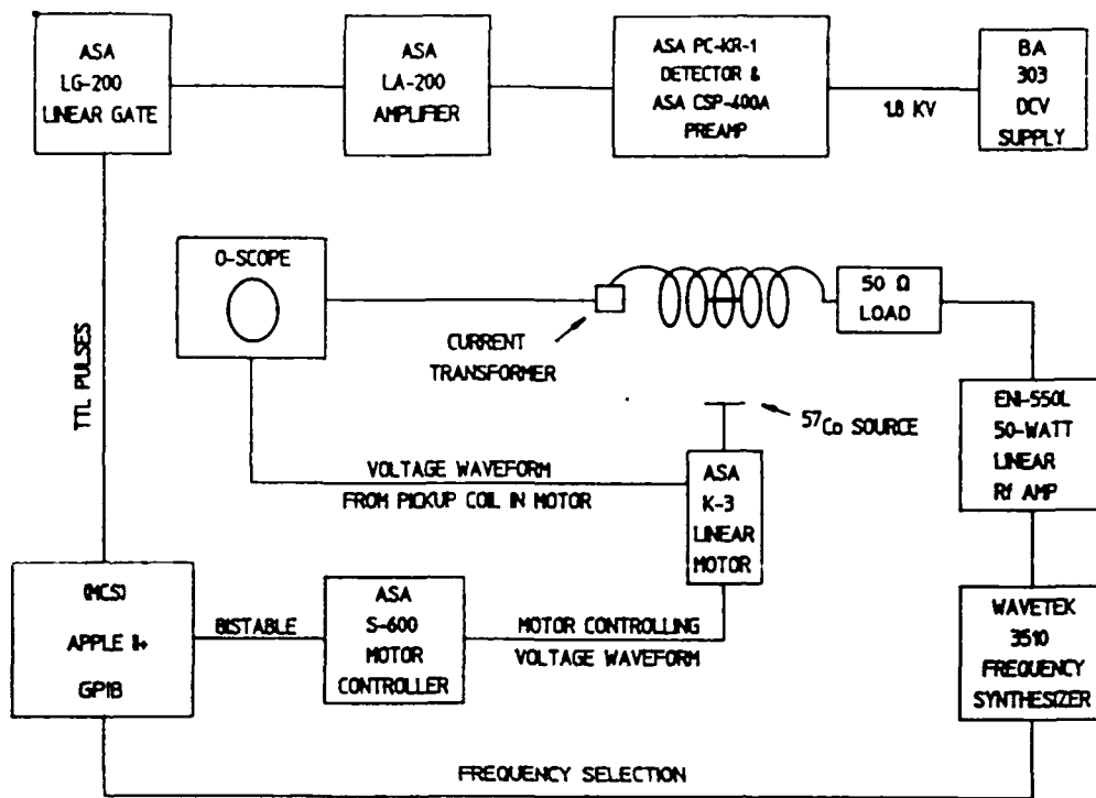
FIG. 1. Schematic representation of a frequency modulation spectrometric (FMS). Please Retype Caption 8.5 Picas
