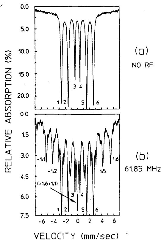
FIG. 2 (a) Mössbauer absorption spectrum of a 2.5- \mu\text{m} foil of iron isotopically enriched with 958 ^{57}\text{Fe} obtained with a ^{57}\text{Co} source in a Pd matrix. The six allowed magnetic dipole transitions are labeled 1 through 6 going from the lowest- to the highest-energy transition. (b) Spectrum of the same foil subjected to an oscillating radio-frequency field with a frequency of 61.85 MHz.
