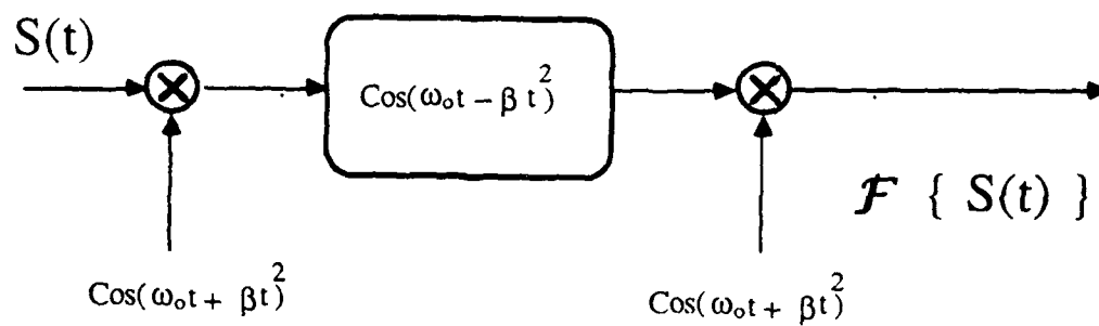
Figure 2b. Multiply-convolve-multiply real time transformation technique.
