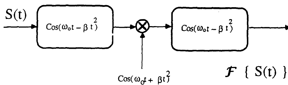
Figure 2a. Convolve-multiply-convolve real time transformation technique.
