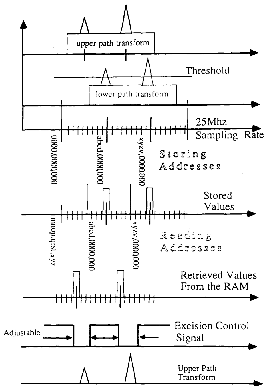
Figure 5b. Detail timing of the implemented excision scheme.
