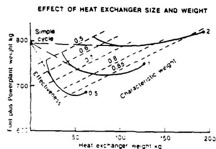
Fig 10 The Influence of Heat Exchanger Effectiveness and Weight
