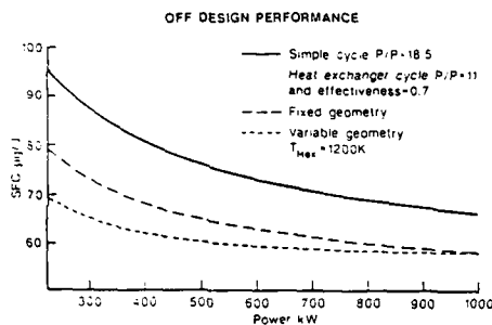
Fig 7 Off Design Performance
