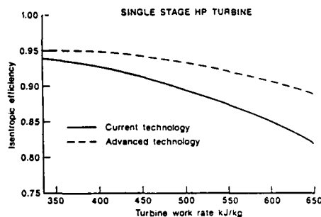
Fig 2 Single Stage Gas Generator Turbine Efficiency
