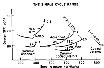
Fig 6 The Simple Cycle Range
