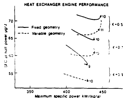
Fig 8 Specific Fuel Consumption at Half Power
