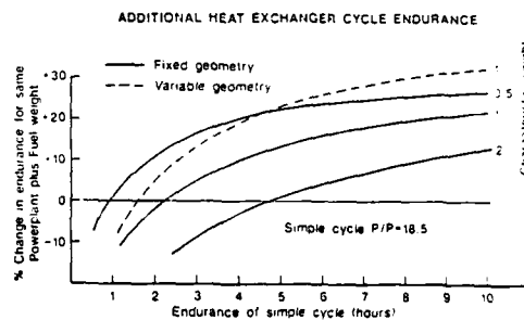
Fig 9 Increase in Endurance of Heat Exchanger Cycle
