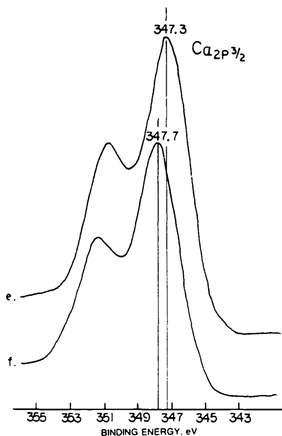
Figure 42. \text{Ca}_{2p_{3/2}} spectra for (e) hydrated cement and (f) 0.5% PI/cement samples.
