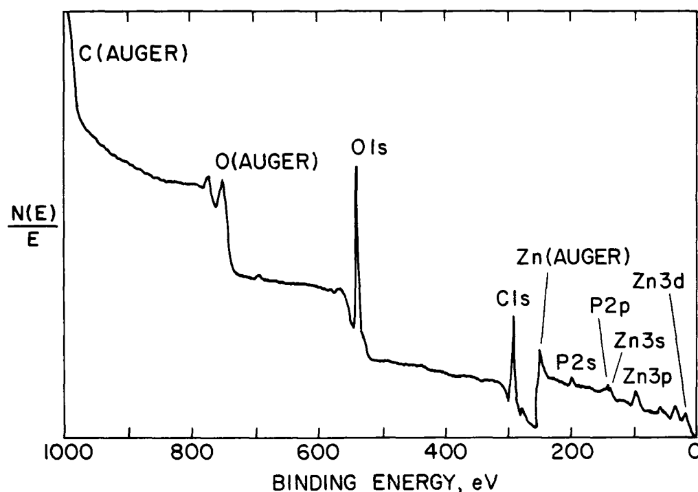
Figure 8. ESCA survey spectrum taken from a p(AA)-complexed Zn·Ph conversion precoating surface.
