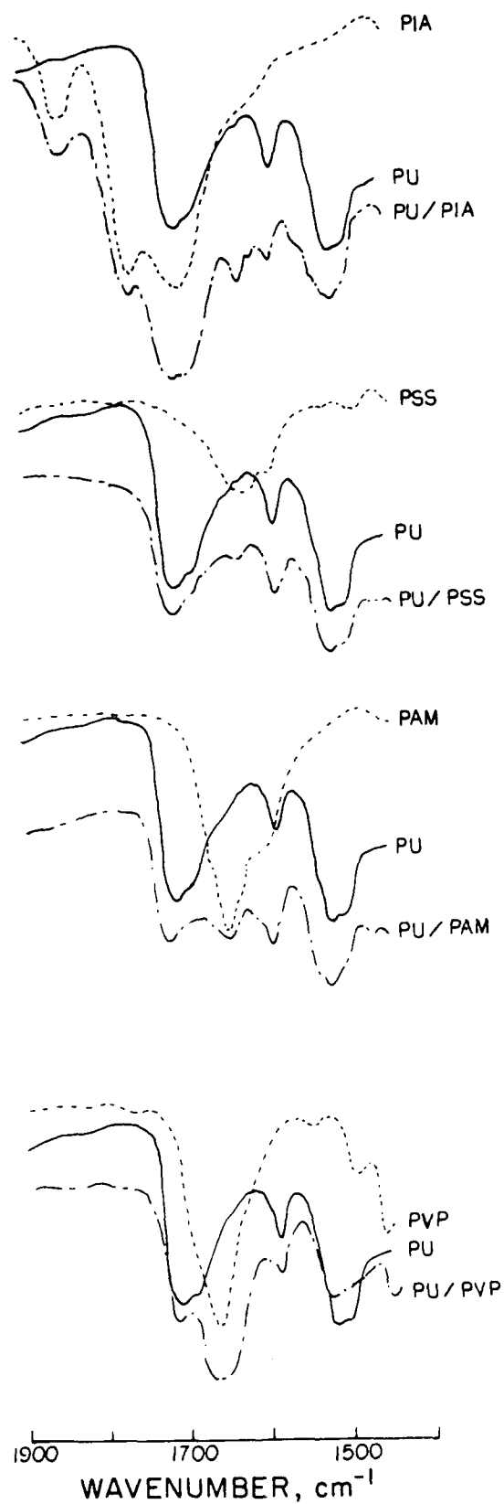
Figure 23. Specular reflectance IR spectra at the interface of PU/p(IA), p(SSA), p(AM), and p(VP) joints.
