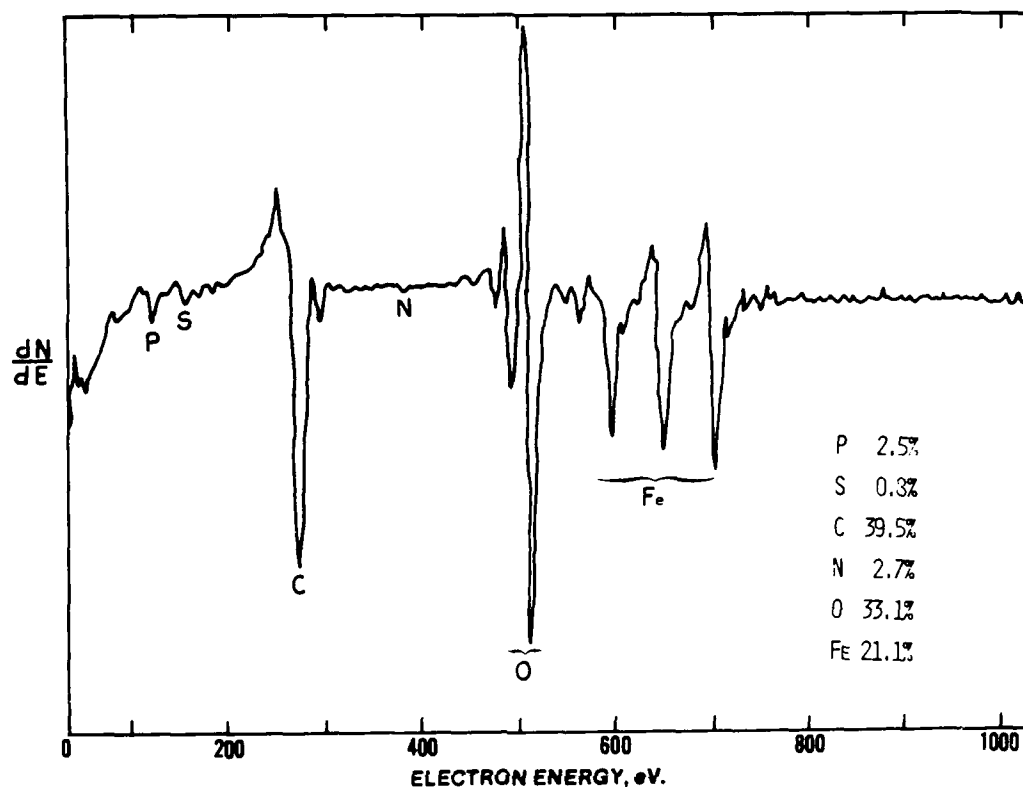
Figure 1. Auger survey spectrum from a solvent-cleaned steel surface.
