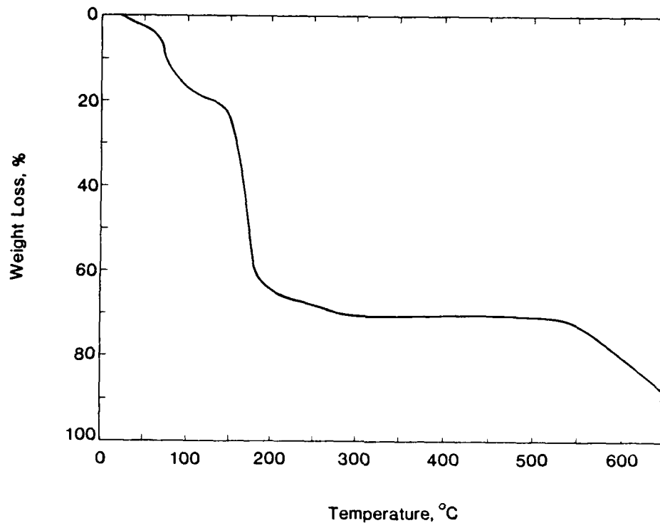
Figure 37. TGA curve for PAA solution.
