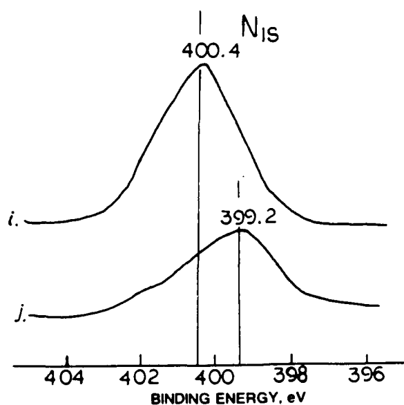
Figure 44. \text{N}_{1s} spectra for (i) bulk PI and (j) 0.5% PI/cement samples.
