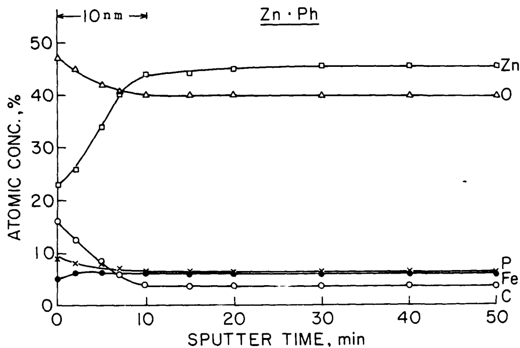
Figure 4. Auger depth profiles for an unmodified Zn·Ph conversion layer.
