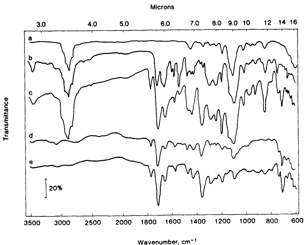
Figure 38. Infrared spectra for (a) BME solvent, (b) PAA solution, (c) 100°C-heated (d) 200°C-heated and (e) 280°C-heated films.
