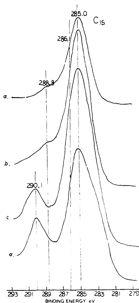
Figure 41. XPS C_{1s} regions for (a) bulk PI, (b) 5% PI-, (c) 1% PI- and (d) 0.5% PI-covered cement samples. Integrated intensity ratio of C ( COO ) and C ( \text{—}\bigcirc\text{—} ): (c) 0.22; (d) 0.35.
