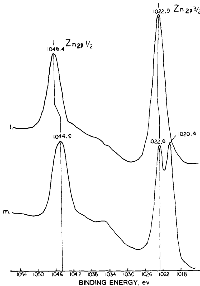
Figure 20. Zn2p regions for unexposed (l) and NaOH - exposed p(AA)-Zn•Ph (m).
