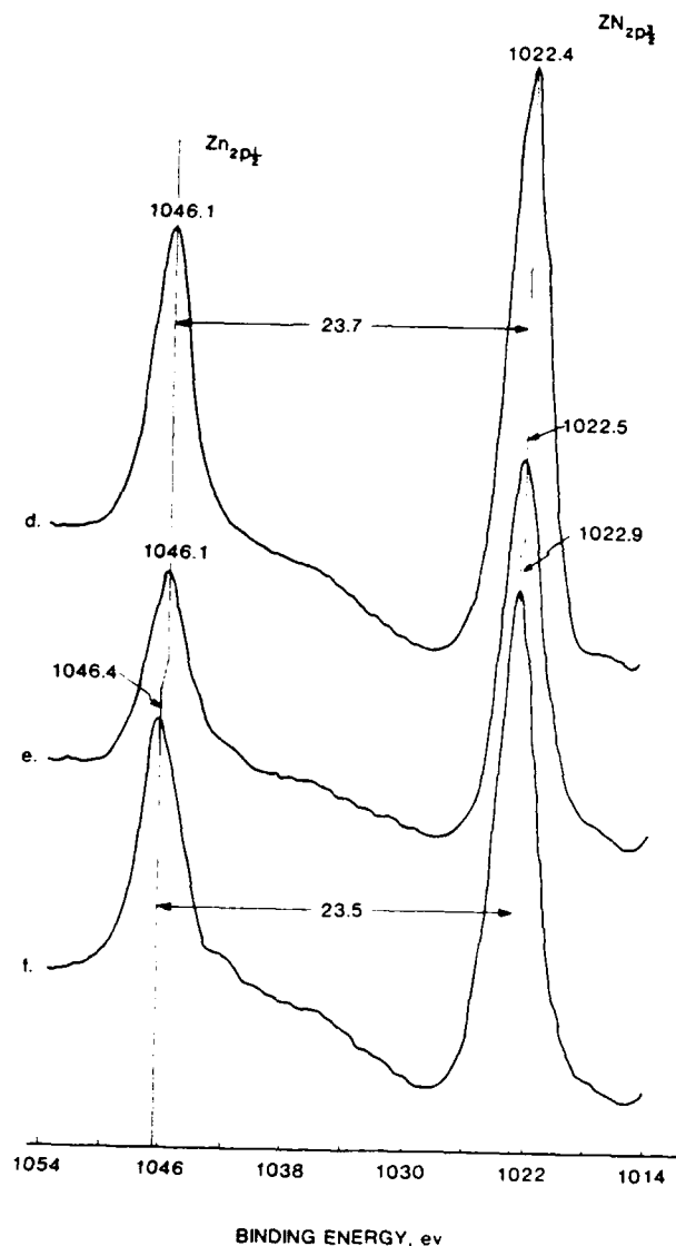
Figure 10. Zn2p separation spectra for unmodified Zn·Ph (d), 5% p(AA)-modified (e) and 1% p(AA)-modified Zn·Ph (f).
