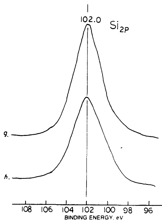
Figure 43. \text{Si}_{2p} spectra for (g) hydrated cement and (h) 0.5% PI/cement samples.
