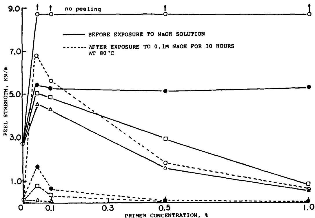
Figure 1. Peel strength as a function of primer concentration for the PU/p(IA)/Al (o), p(VPD)/ (e), /p(AM)/ (□), and /p(SSA)/ (Δ) joint systems before and after exposure for 30 hr to hot alkali at 80°C.
