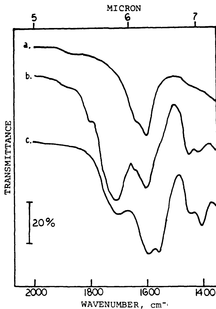
Figure 21. Infrared spectra for \text{Zn}_3(\text{PO}_4)_2 \cdot 2\text{H}_2\text{O} powder (a), p(AA)- \text{Zn}_3(\text{PO}_4)_2 \cdot 2\text{H}_2\text{O} composite (b) and composite subjected to NaOH exposure (c).
