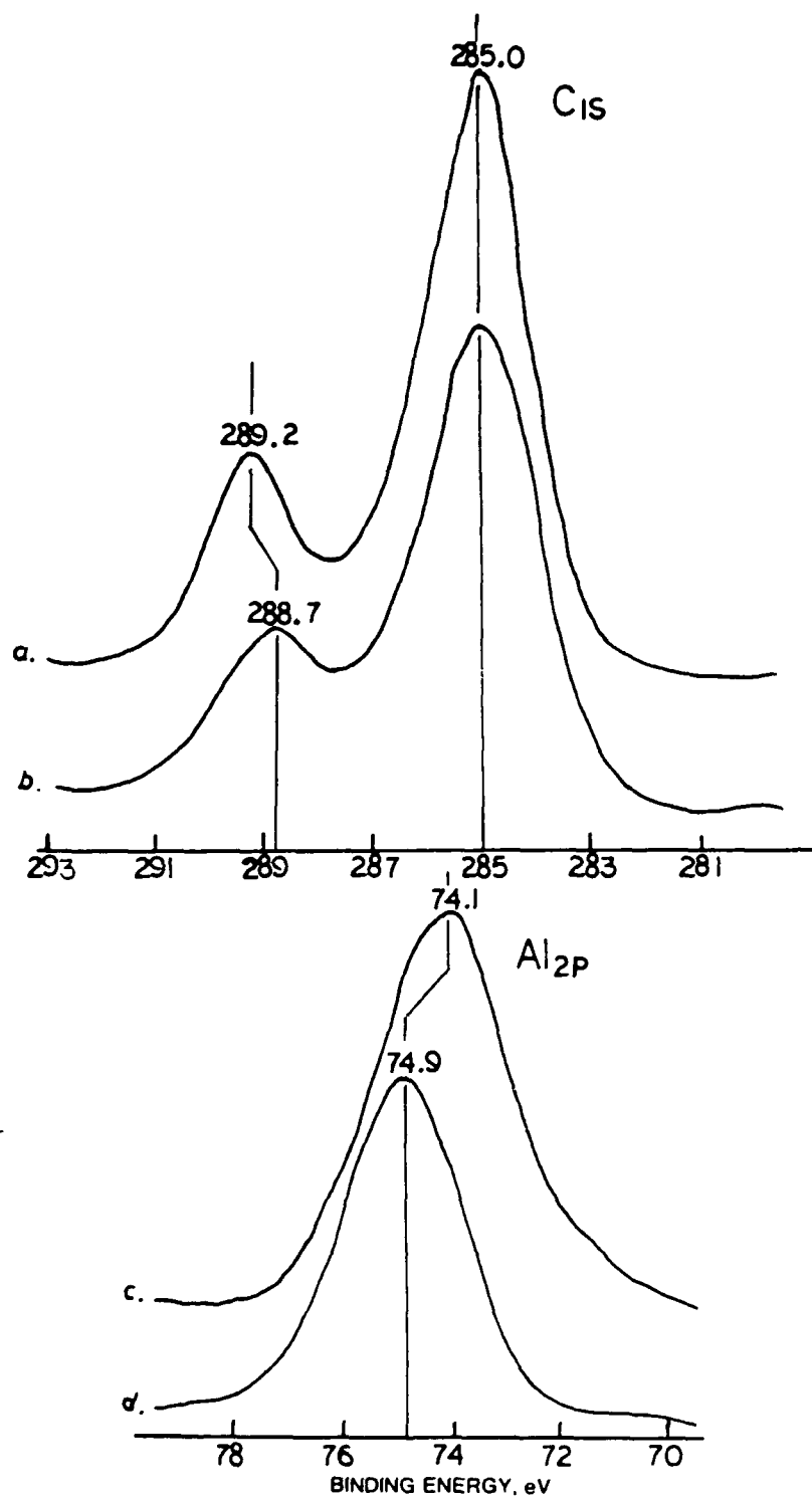
Figure 28. C_{1s} and Al_{2p} regions of bulk p(IA) surface (a), Al_2O_3 surface (c), and the p(IA)- Al_2O_3 interfaces (b and d).
