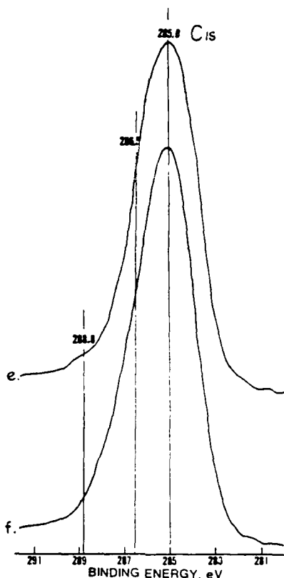
Figure 33. XPS spectra of C_{1s} region for peeled PU/0.05% p(VPD)/ Al_2O_3 systems before (e) and after (f) exposure. Integrated intensity ratio of C(C-N \text{ and } C-O)/C(CH_2) : (e) 0.34; (f) 0.19.
