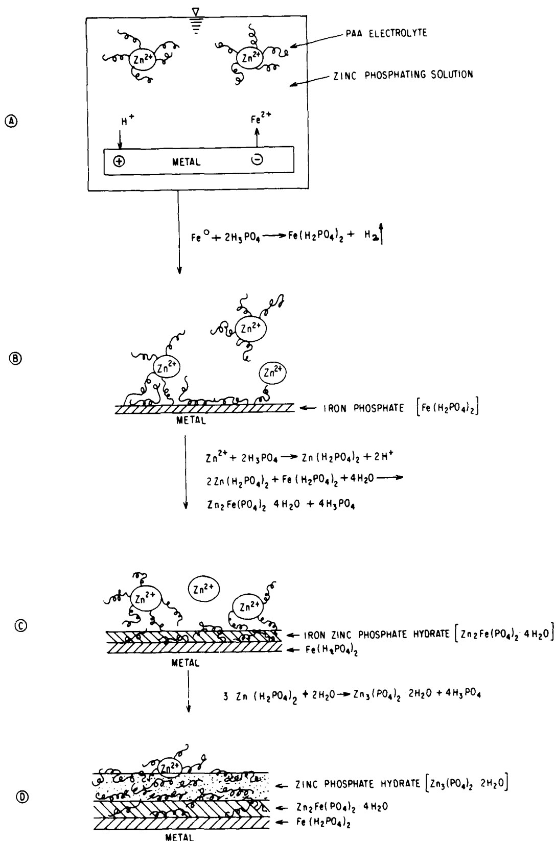
Figure 12. Schematic conversion mechanism of polyelectrolyte-zinc phosphate systems deposited on steel surfaces.
