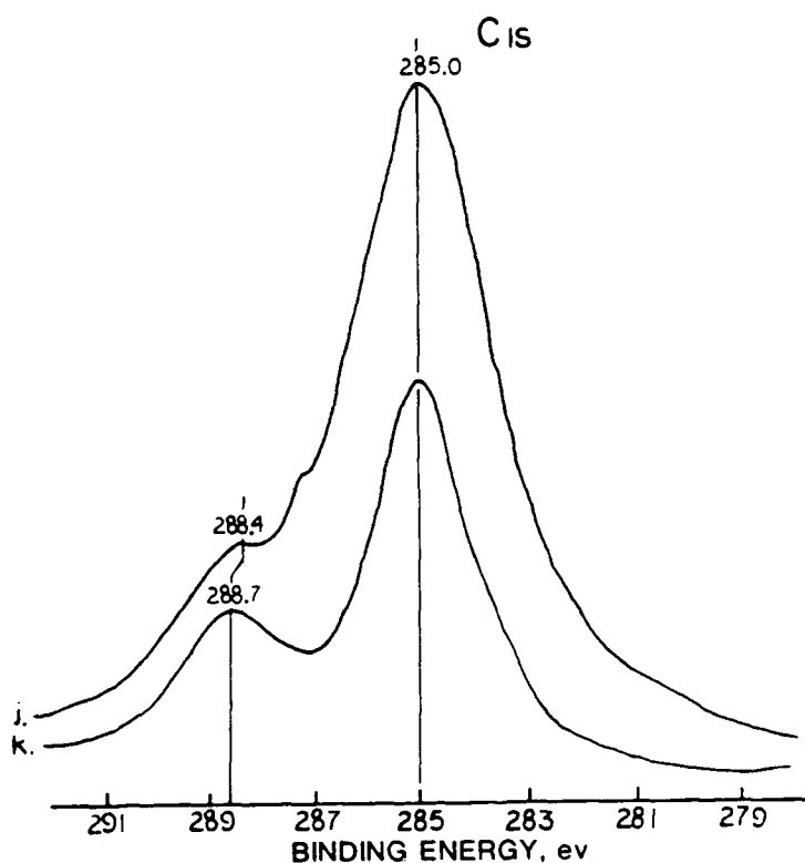
Figure 19. C_{1s} spectra for 1% p(AA)-modified Zn·Ph before (j) and after (k) exposure in 0.1M NaOH solution.
