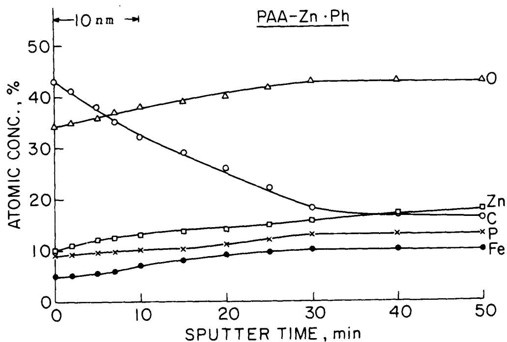
Figure 5. Auger depth profiles for a p(AA)-chemisorbed Zn·Ph layer system.
