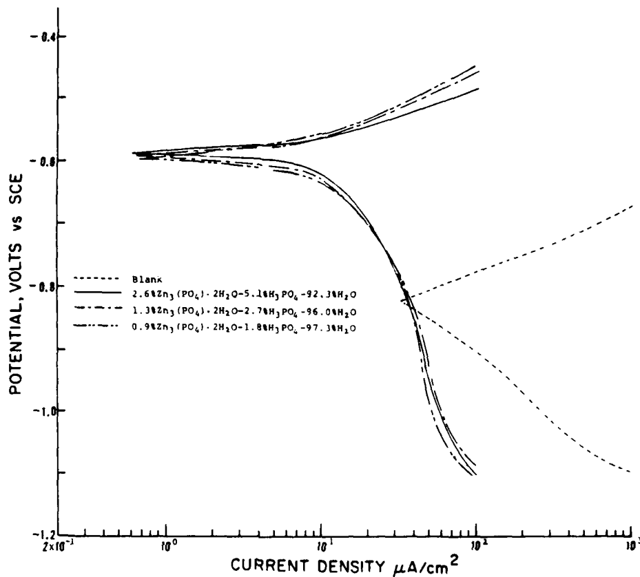
Figure 14. Comparisons of polarization curves for blank steel and steel containing conversion coatings deposited through dissolution-recrystallization processes.
