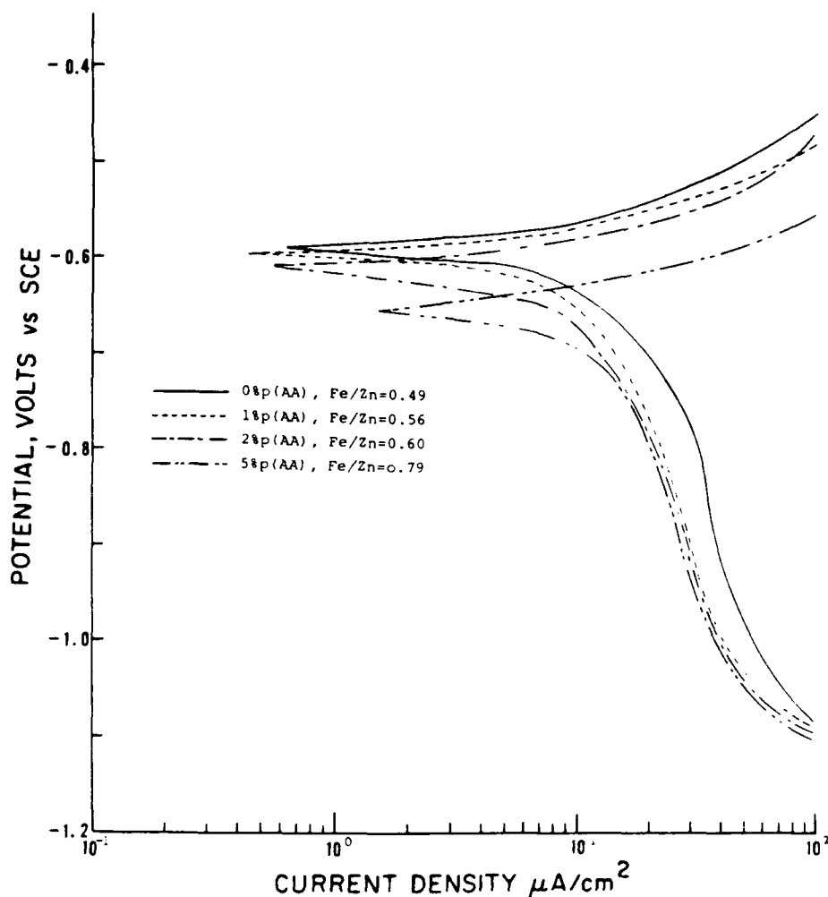
Figure 18. Polarization curves for zinc phosphated steel specimens containing p(AA) concentrations of up to 5% in aerated 0.5M NaCl solutions.
