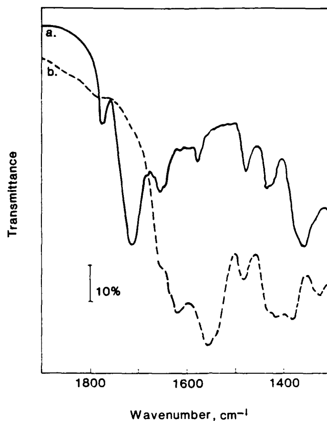
Figure 45. Infrared spectra for cement-filled PI specimens before (a) and after (b) exposure to steam at 300°C.
