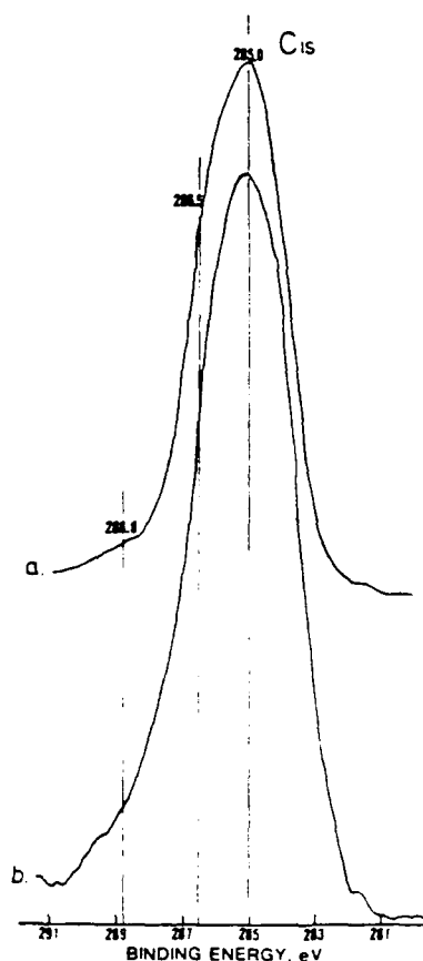
Figure 31. C 1s spectra of peeled Al 2 O 3 surfaces from PU/Al 2 O 3 joints before (a) and after (b) exposure. Integrated intensity ratio of C(C-N and C-O)/C(CH 2 ) (a) 0.52; (b) 0.29.
