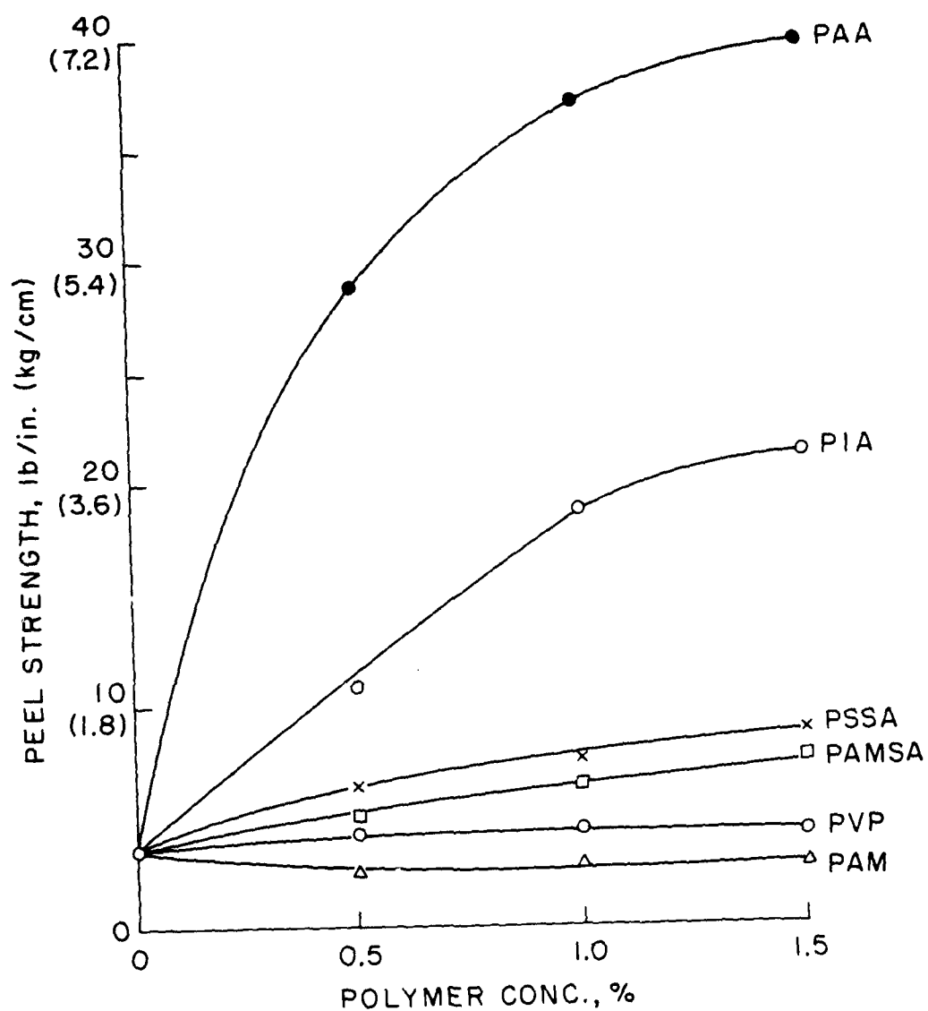
Figure 22. Changes in the 180°-peel strength at PU-to-modified Zn·Ph joints as a function of polyelectrolyte and non-polyelectrolyte macromolecule concentrations.
