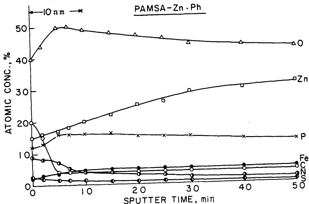
Figure 7. Auger depth profiles for a semipolyelectrolyte p(\text{AMSA})\text{-Zn}\cdot\text{Ph} composite layer.
