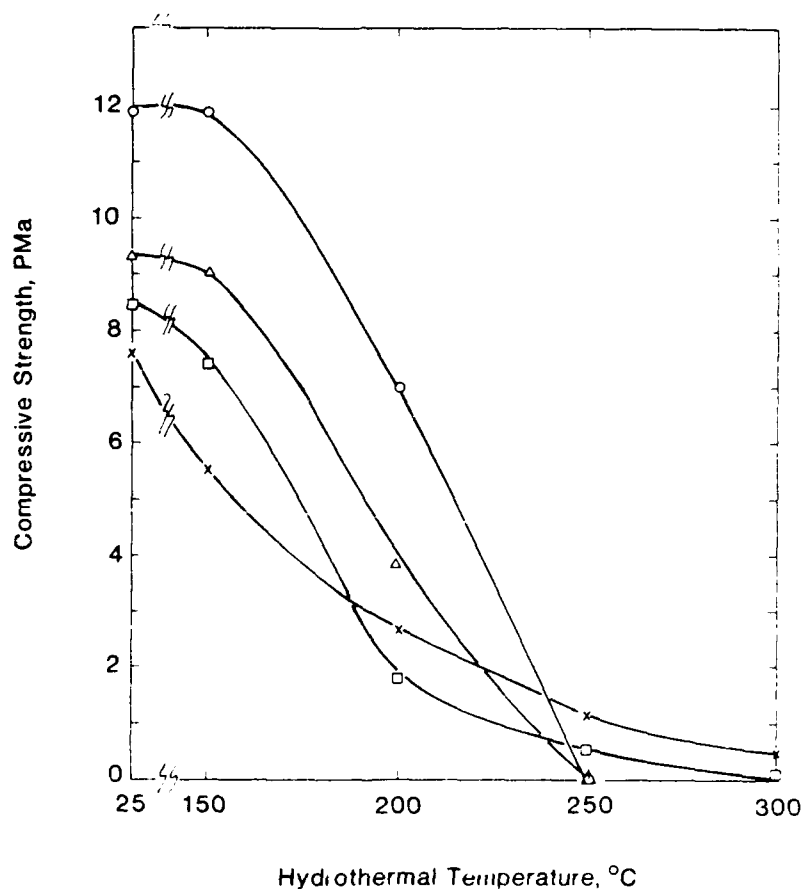
Figure 40. Compressive strength vs hydrothermal temperature for PI specimens containing 0% (o), 2% (Δ), 5% (□) and 8% (x) cement.
