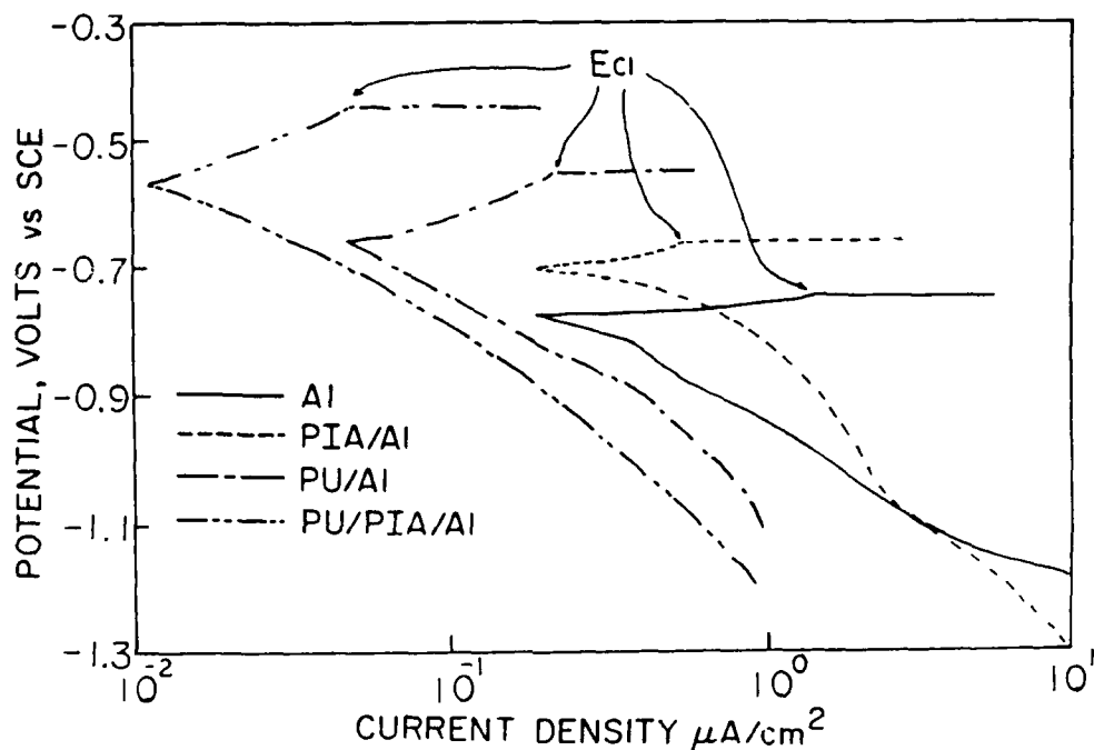
Figure 36. Polarization curves for uncoated, p(IA), PU-, and PU-p(IA)-coated aluminum immersed in deaerated 0.5 M NaCl solution at 25°C.
