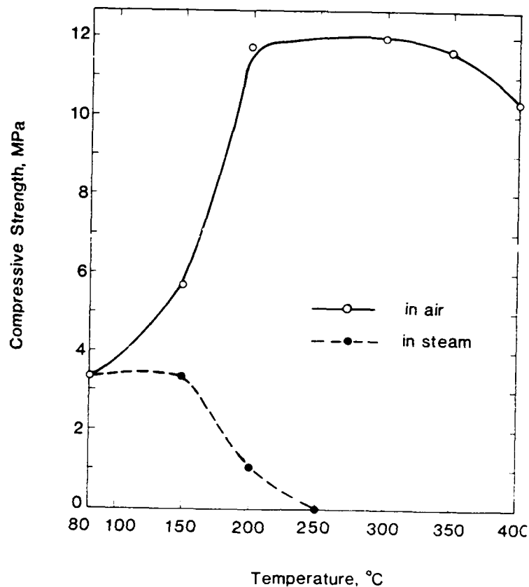
Figure 39. Changes in compressive strength of 80°C air-precured PI specimens after exposure to air or steam at temperatures up to 400°C.
