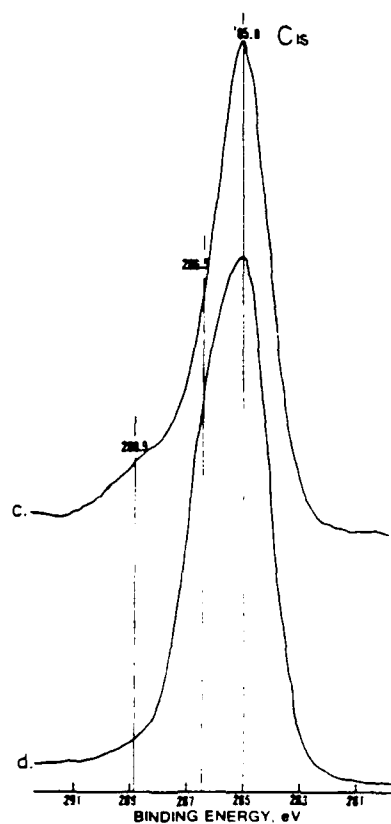
C 1s peaks of Al 2 O 3 surface removed from PU/0.05% p(IA)/Al 2 O 3 (c) and /1.0% p(IA)/ (d) joints after exposure. Integrated intensity ratio of C (C-N and C-O)/C (CH 2 ): (c) 0.38; (d) 0.66.
