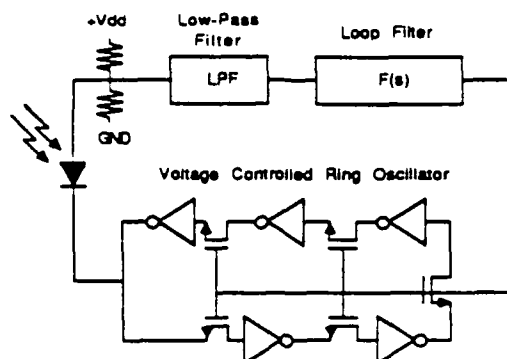
Figure 2.2: Block diagram of Clymer's phase-locked loop design
