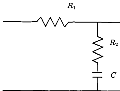
Figure 21: Lag-lead low pass loop filter.
