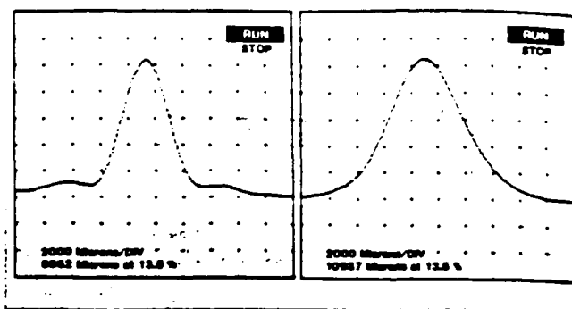
Fig. 6 Horizontal (left) and vertical (right) intensity profiles of the 79426 Laser System at 4m from the laser output.
