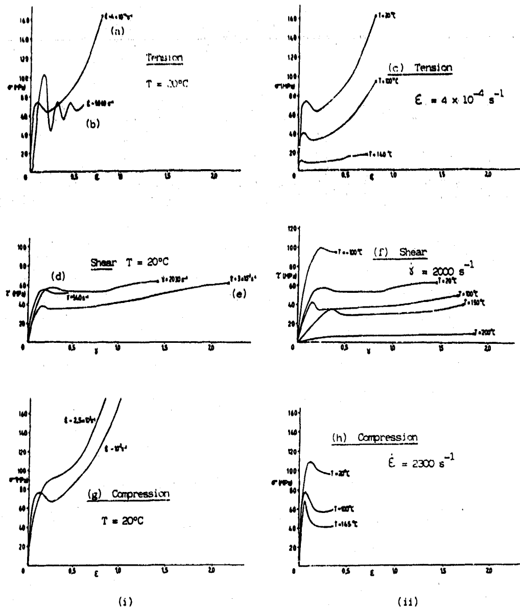
Fig. 1. Stress-strain response of PC. (i) Effect of strain rate; (ii) Effect of temperature. Sources: (a),(c) Vest, Aneddo and Lee (1987); (b),(d),(f) the authors; (g) Walley et al (1989); (h) Steer (1985); x at the end of a curve denotes fracture.
