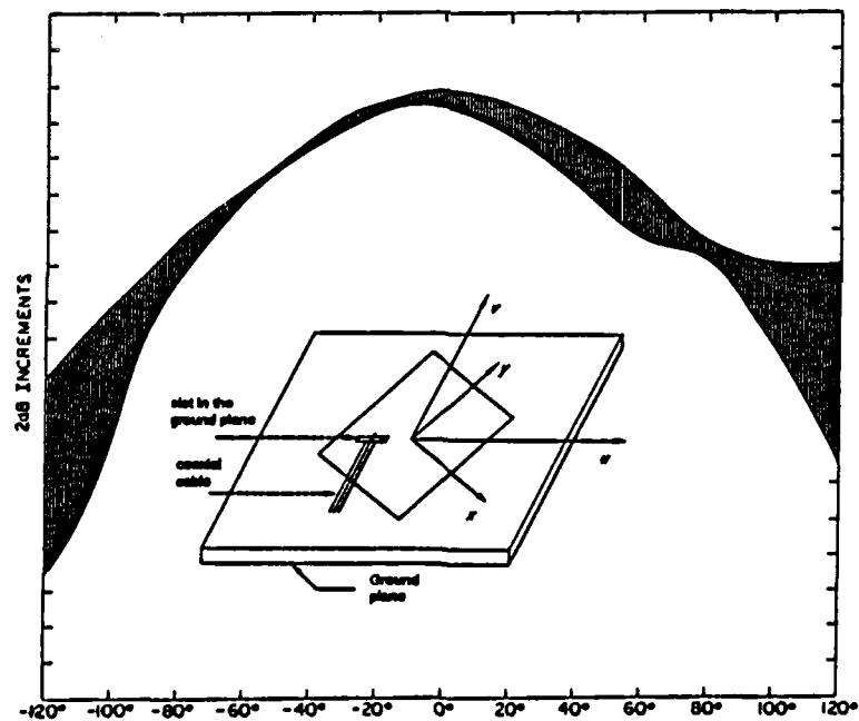
Fig. 2. Radiation pattern for RHCP slot-fed antenna on a 1/8" thick substrate.
