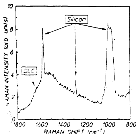
FIG. 2 Spectrum of the Raman scattering of the 514.5\text{ nm} output of an argon ion laser from a 180\text{-Å} -thick film of DLC grown on a Si(111) substrate from carbon ions from the laser ion source.
