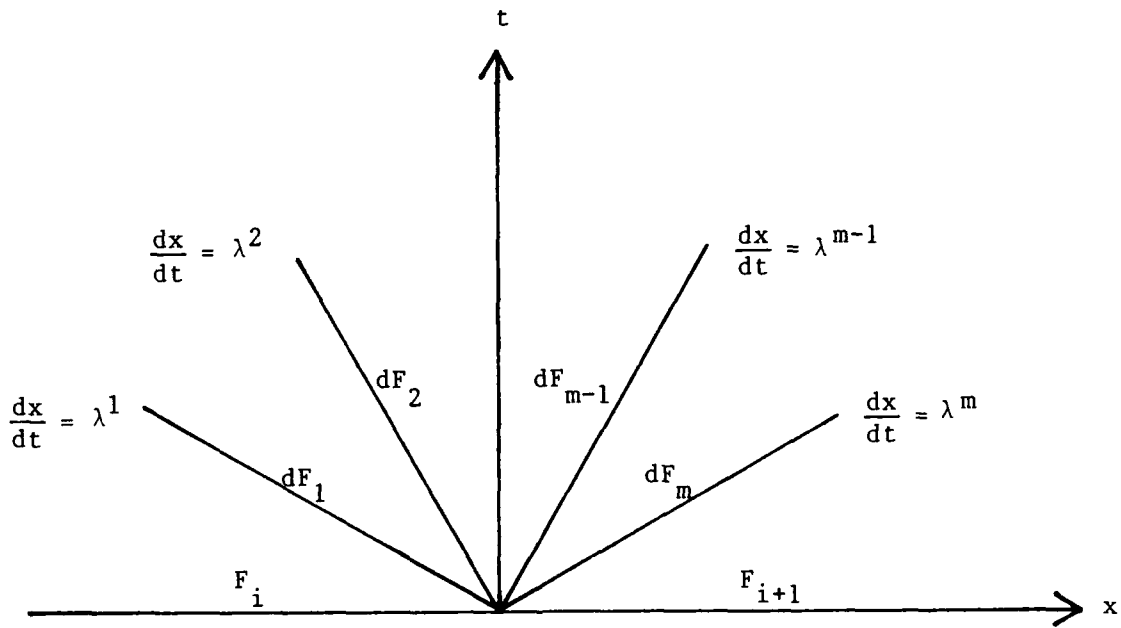
Figure 3.1 Characteristic Waves
