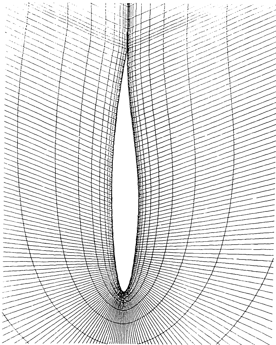
Figure 10. "C" grid for RAE 2822 airfoil (221 x 31 x 2)
