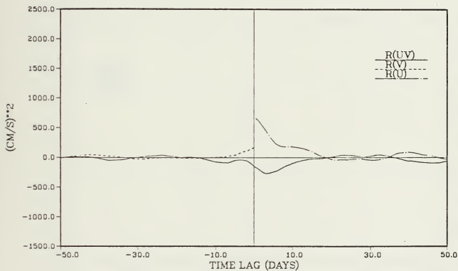
Figure 24. Buoy 53 Lagrangian Velocity Correlations: Computed after removing the effects of the Mindanao Eddy. Days 204-257.
