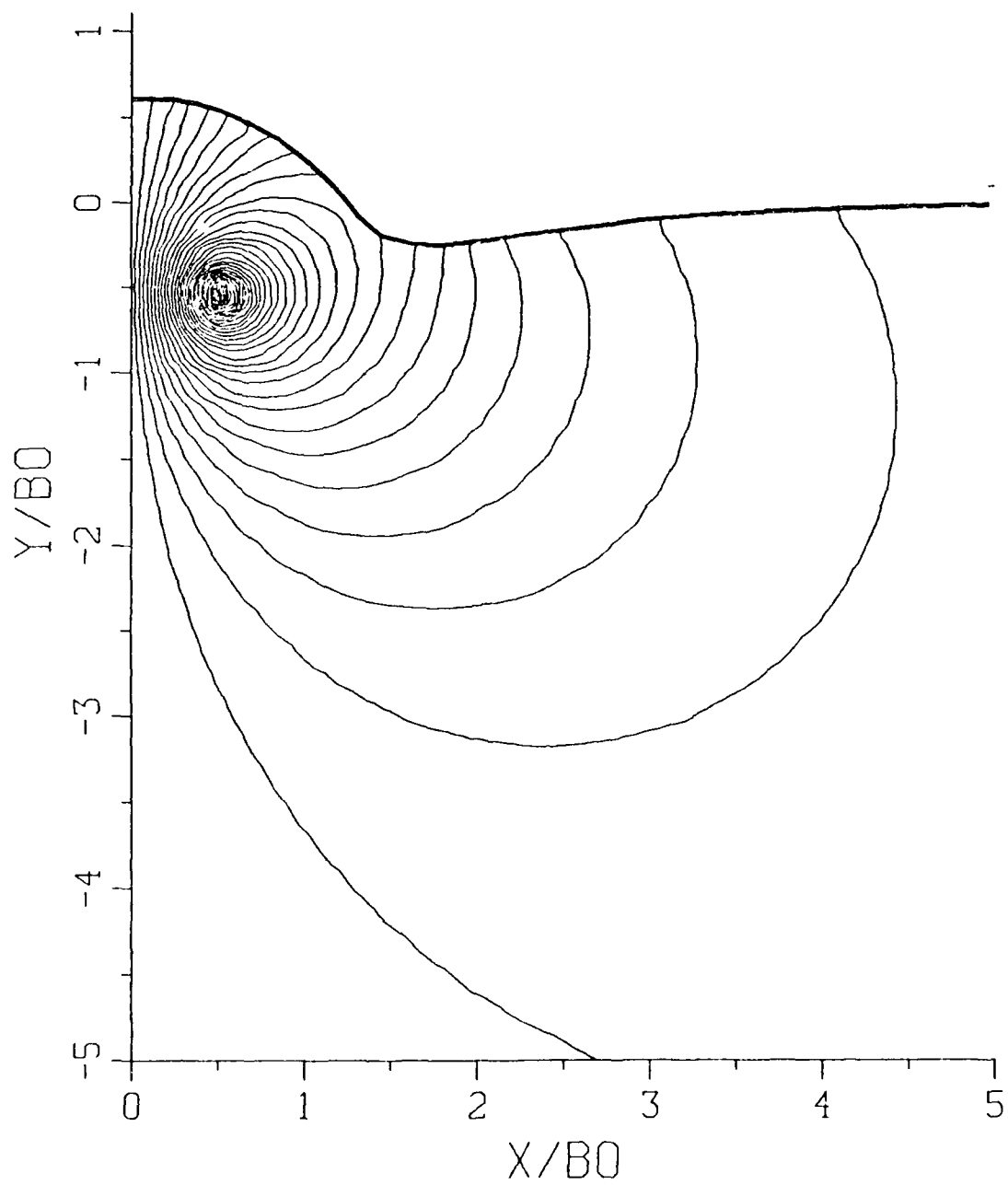
Figure 13. Streamlines at T = 0.65
