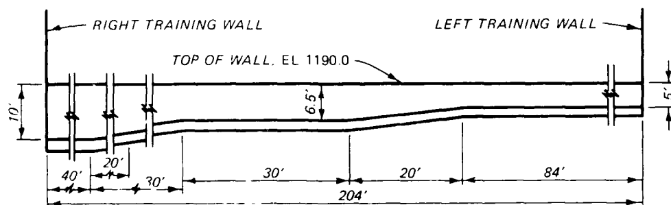
DOWNSTREAM ELEVATION
