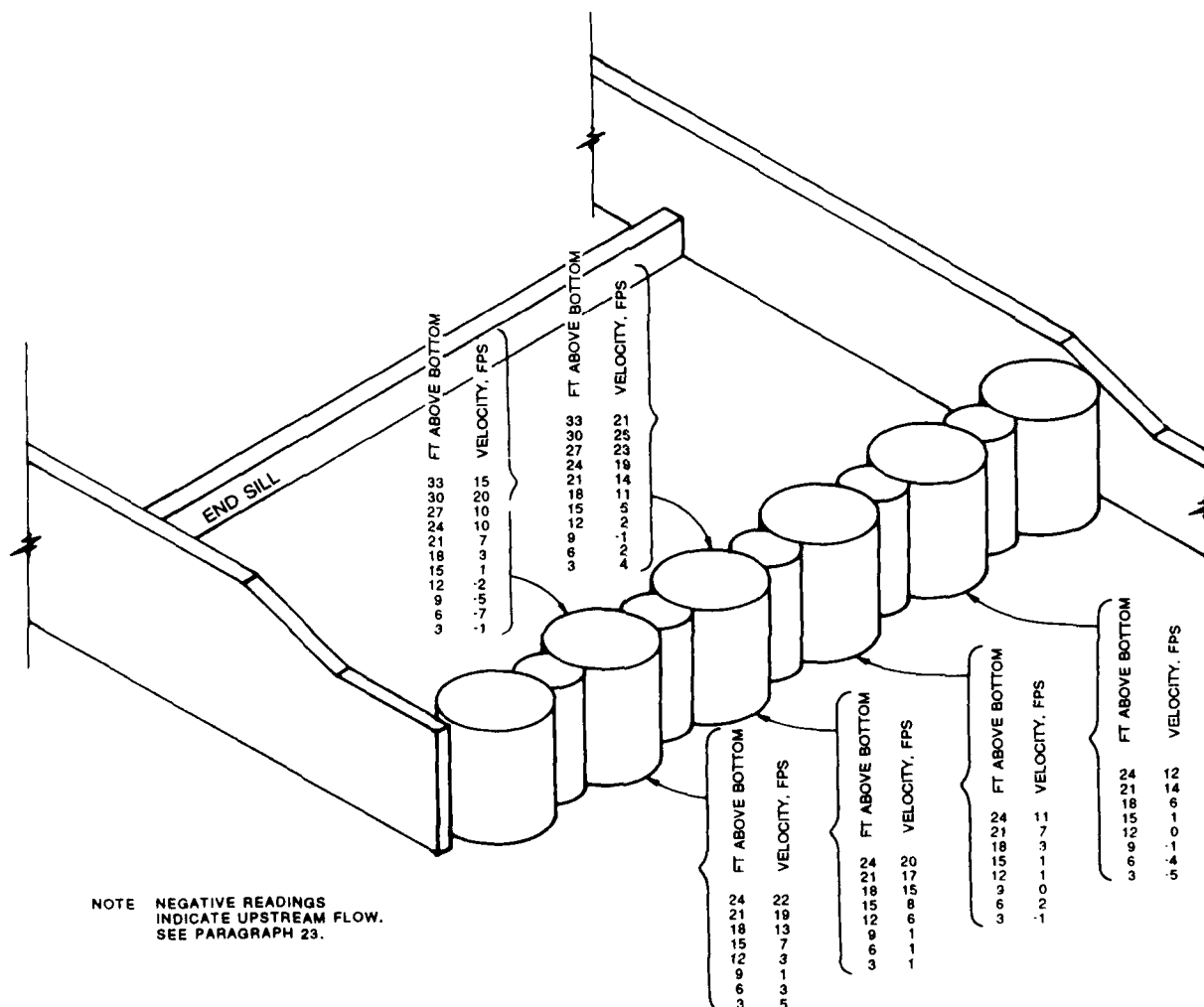
Figure 4. Sluices 3, 4, 7, and 8 fully open (10 ft each), tailwater el 1,207.5
