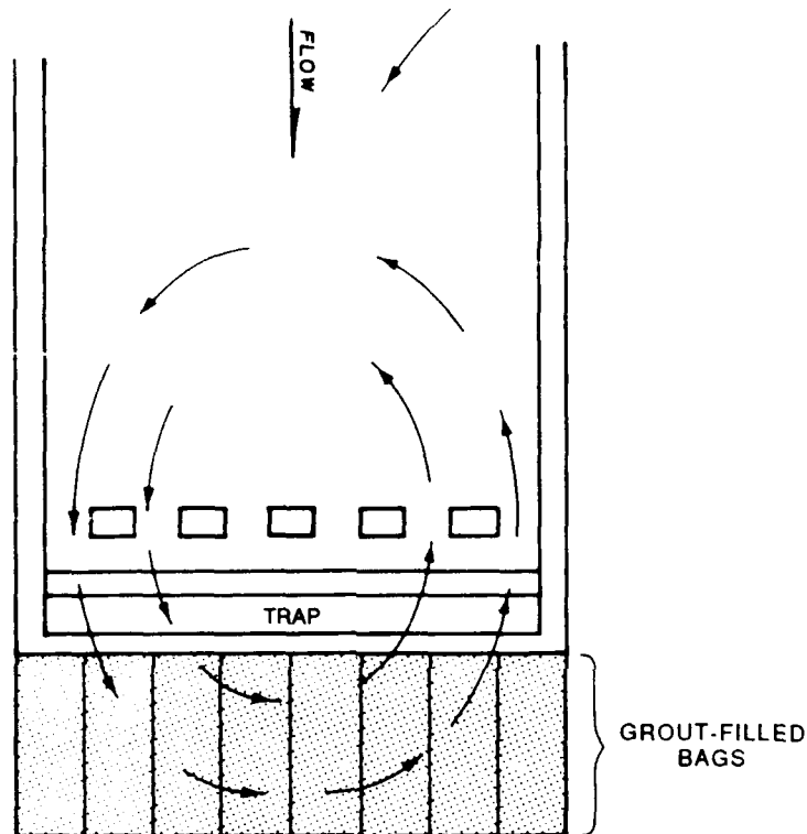
Grout-Filled Bags
