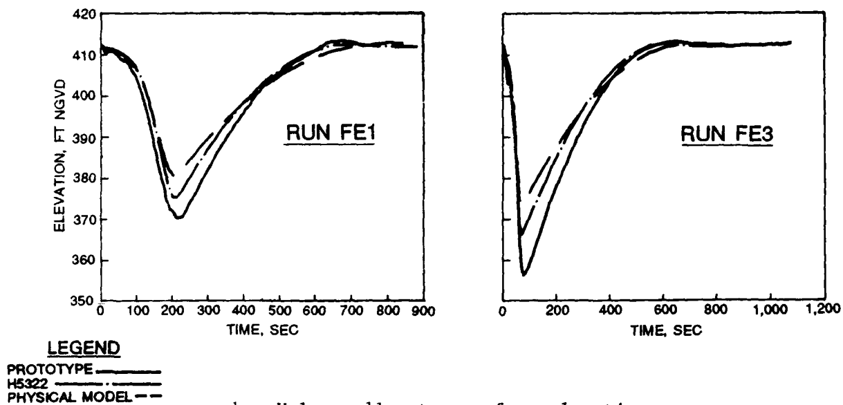
b. Valve well water-surface elevation
