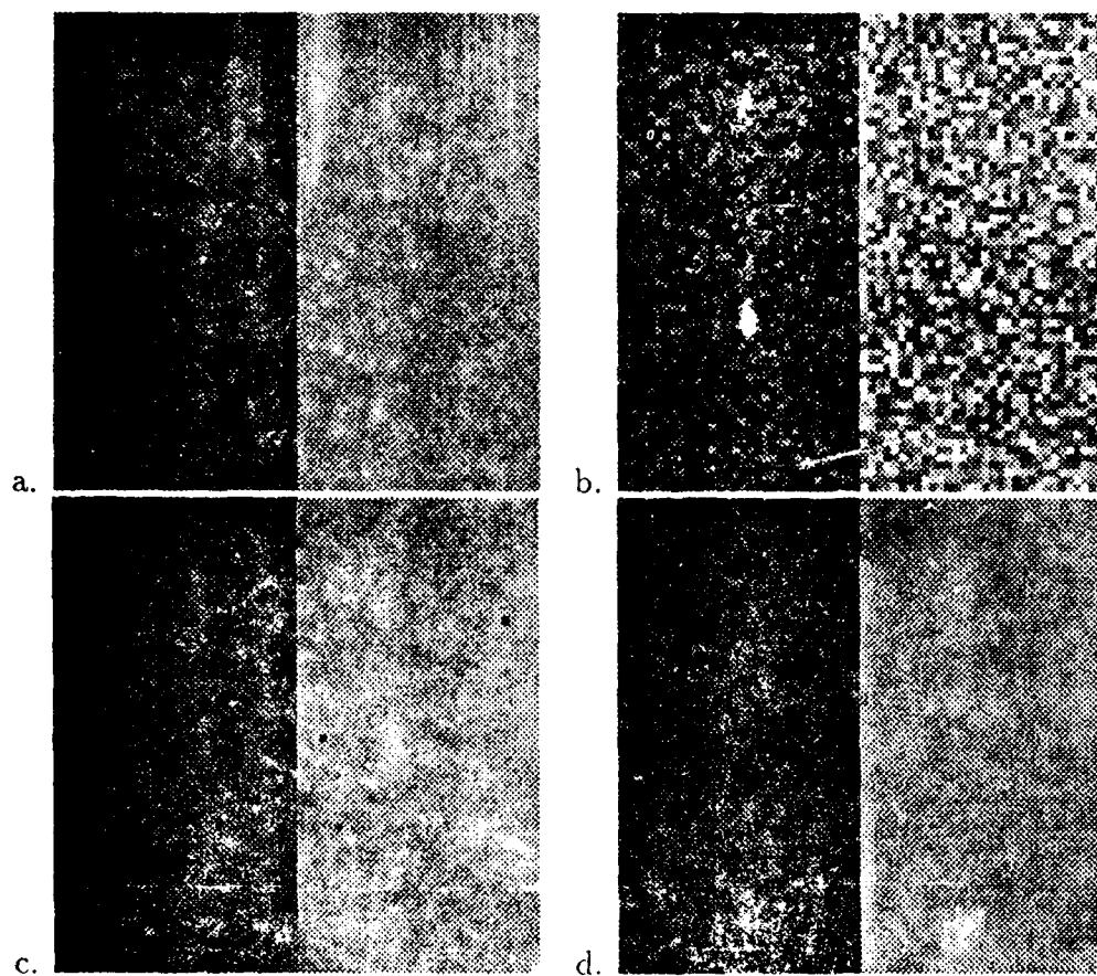
Figure 9: a) Step edge with 140 grey value units for the step. b) White noise with standard deviation 30 grey value units has been added. c) The noisy image after 20 iterations for \alpha = 4 , \gamma = 24000 , \epsilon = 0 . d) The noisy images after 20 iteration for \alpha = 4 , \gamma = 45000 , \epsilon = 0.9
