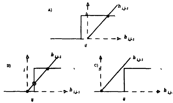
Figure 5: The three figures illustrate the solution of (3.12) according to different values of the gradient field f ( \Delta_{ij}^h ) a) The line process is on ( h_{ij} = 1 ) b) Two solution (three solution for temperature different then zero) c) Shows the solution of no line-process ( h_{ij} = 0 )
