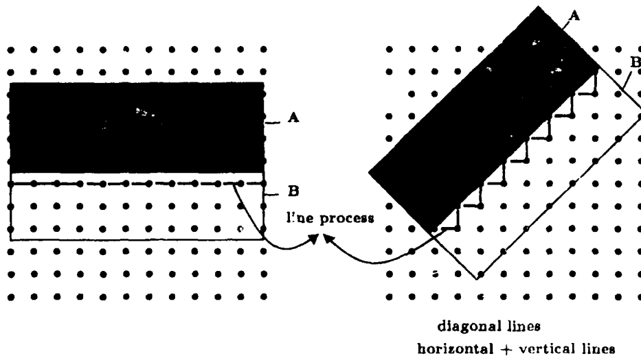
Figure 2: a) At the discontinuity, \Delta_{i,j}^{h,2} = (B - A)^2 and \Delta_{i,j}^{v,2} = 0 . A chain of horizontal line processes are created for (\frac{\gamma}{\alpha} < (B - A)^2) . b) At the discontinuity, \Delta_{i,j}^{h,2} = (B - A)^2 and \Delta_{i,j}^{v,2} = (B - A)^2 . A chain of horizontal and vertical line processes are created for (\frac{\gamma}{\alpha} < (B - A)^2) .
