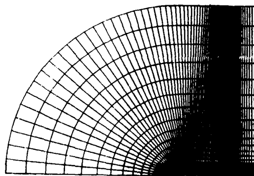
b. Transonic Grid
