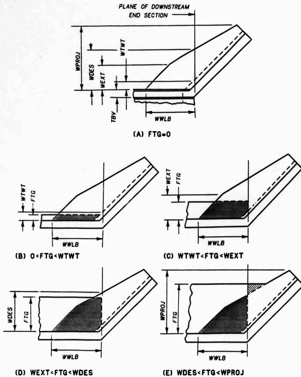
Figure 53. Basin-wingwall footing possibilities
