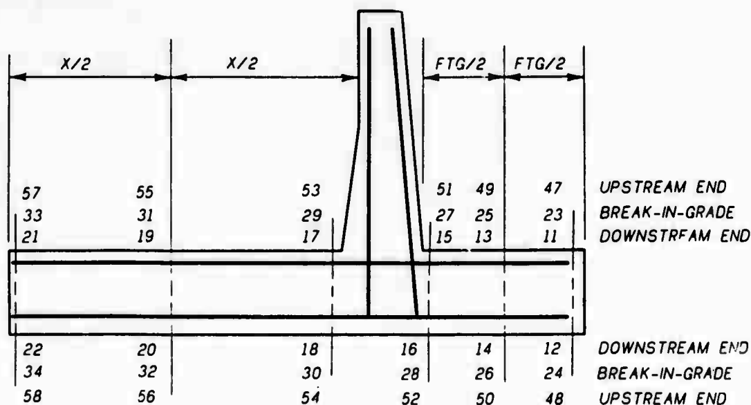
Figure 45. Base slab steel layout and point locations
