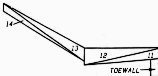
(B) SLAB VOLUMES
