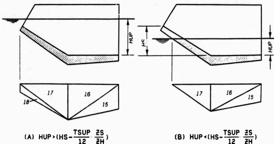
Figure 20. Components of uplift for LC#1 or LC#2
