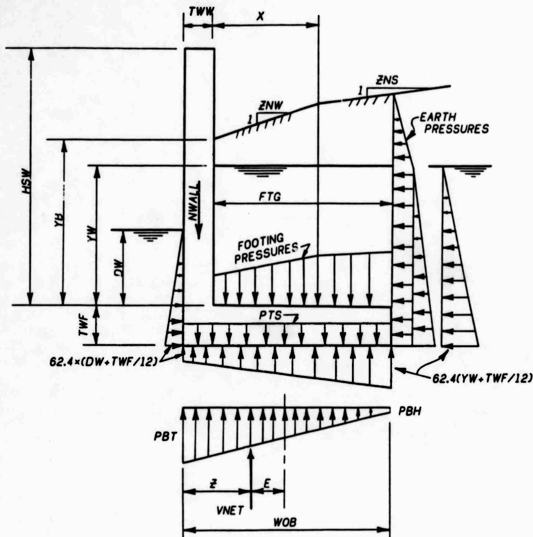
Figure 39. Wingwall overturning and bearing
