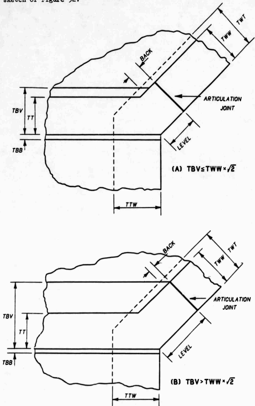
Figure 52. Corner detail, wingwall-to-sidewall
