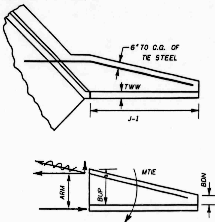
Figure 41. Wingwall-to-basin tie steel area
