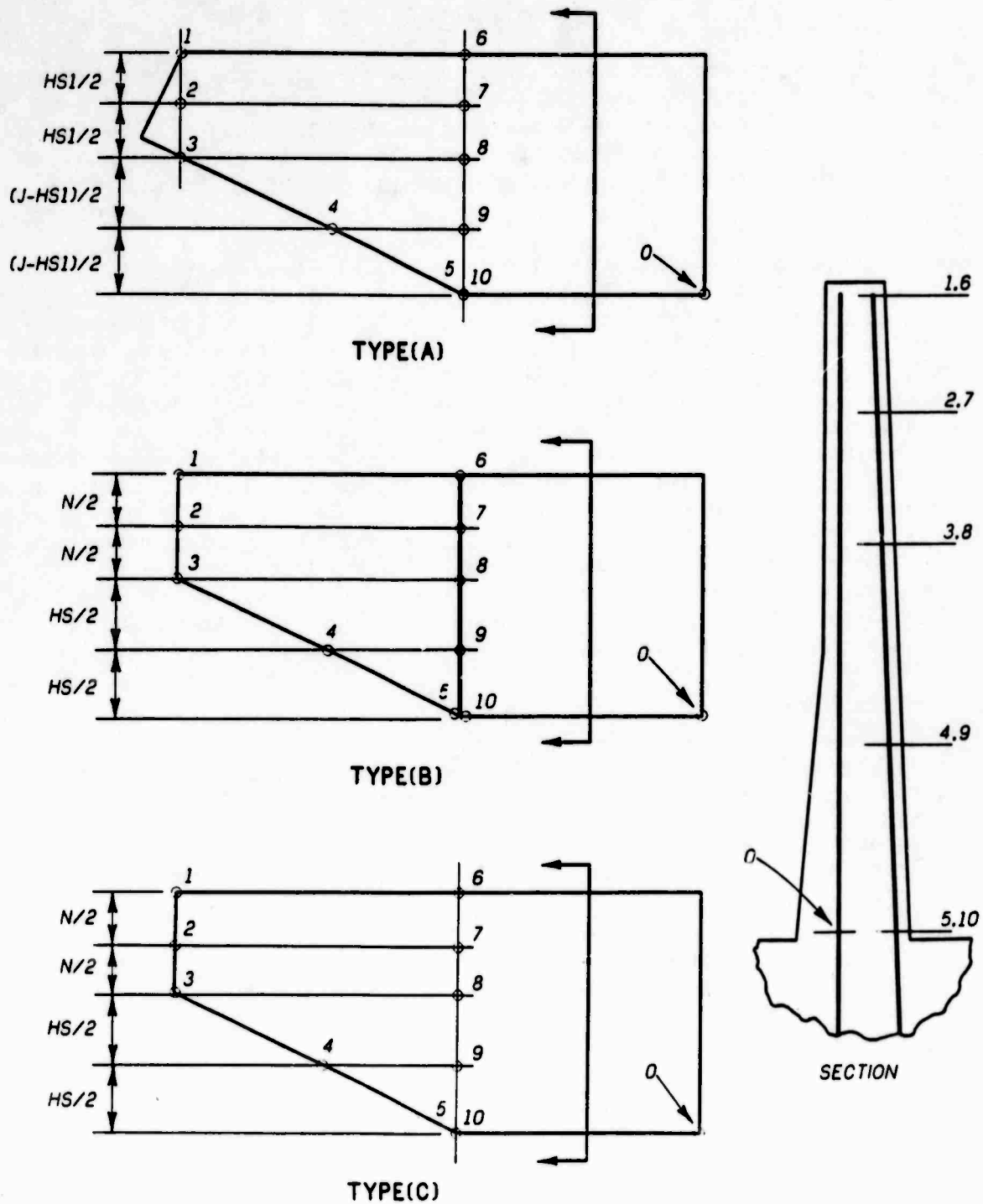
Figure 42. Sidewall steel layout and point locations
