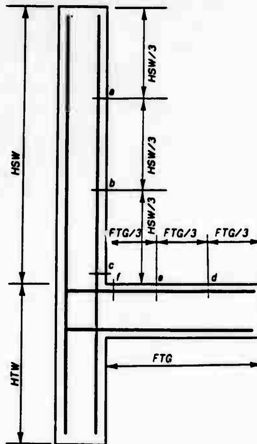
Figure 48. Wingwall section steel layout
