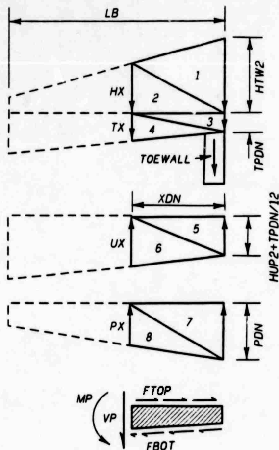
Figure 30. Shear and moment in pavement slab, LC#2
