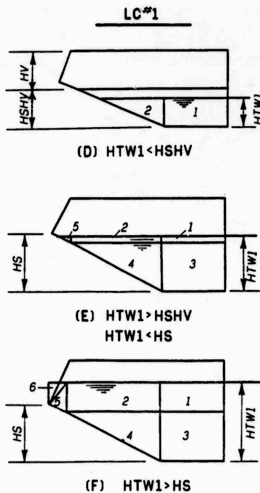
Figure 18. Components of volume of water in basin
