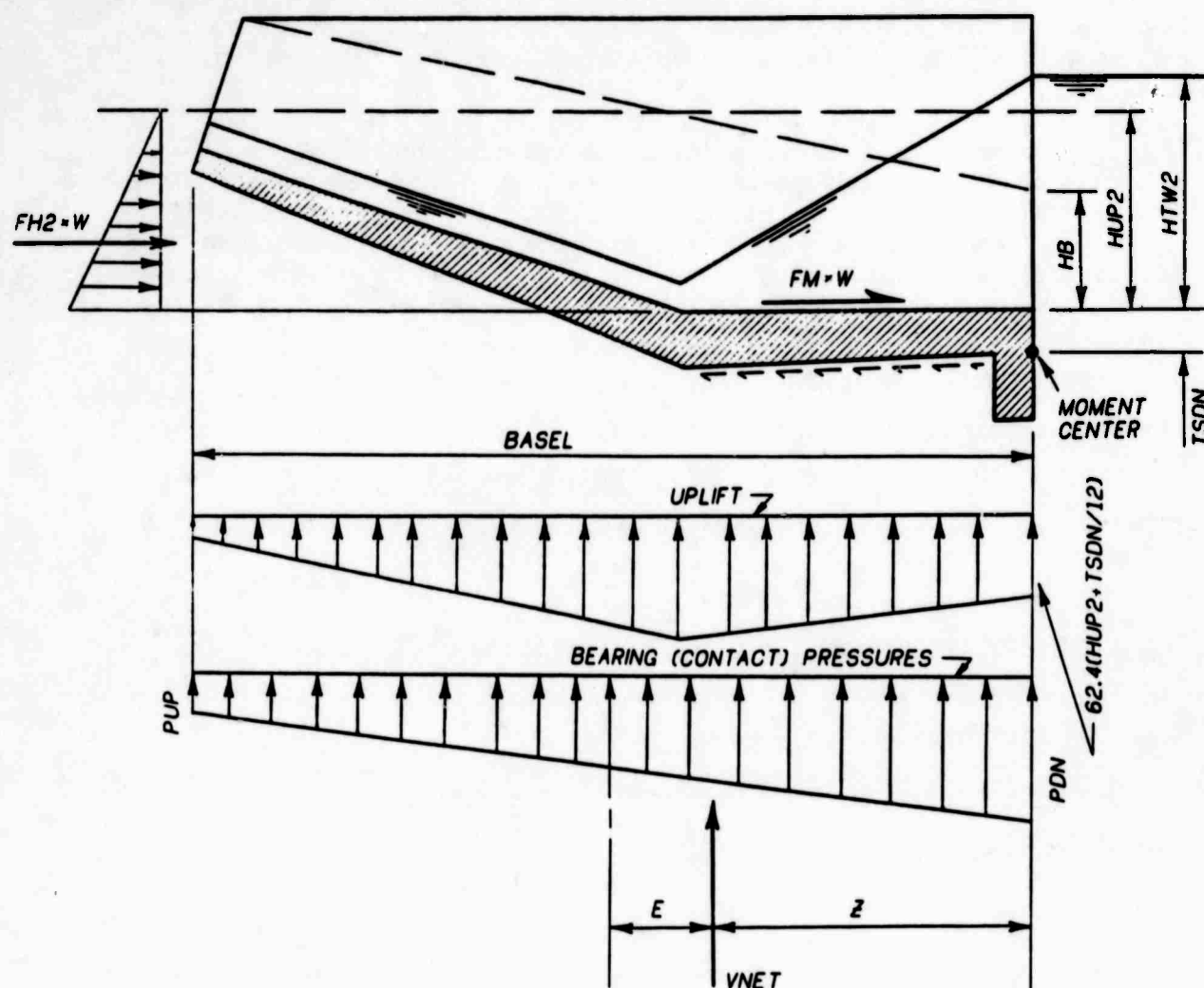
Figure 21. Determination of bearing pressures for LC#2
