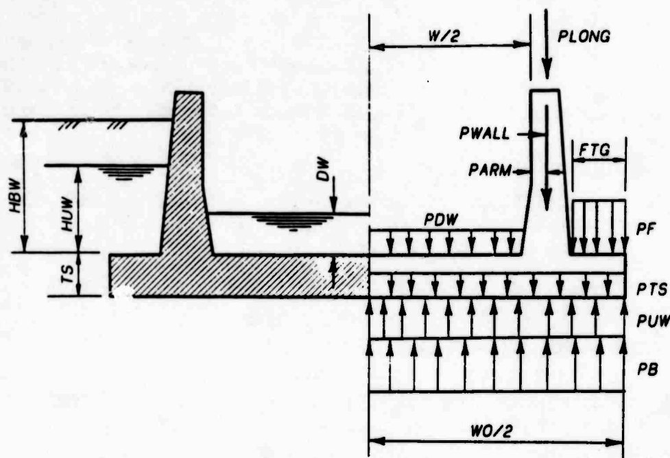
Figure 22. Loads for floor slab shear and bending
