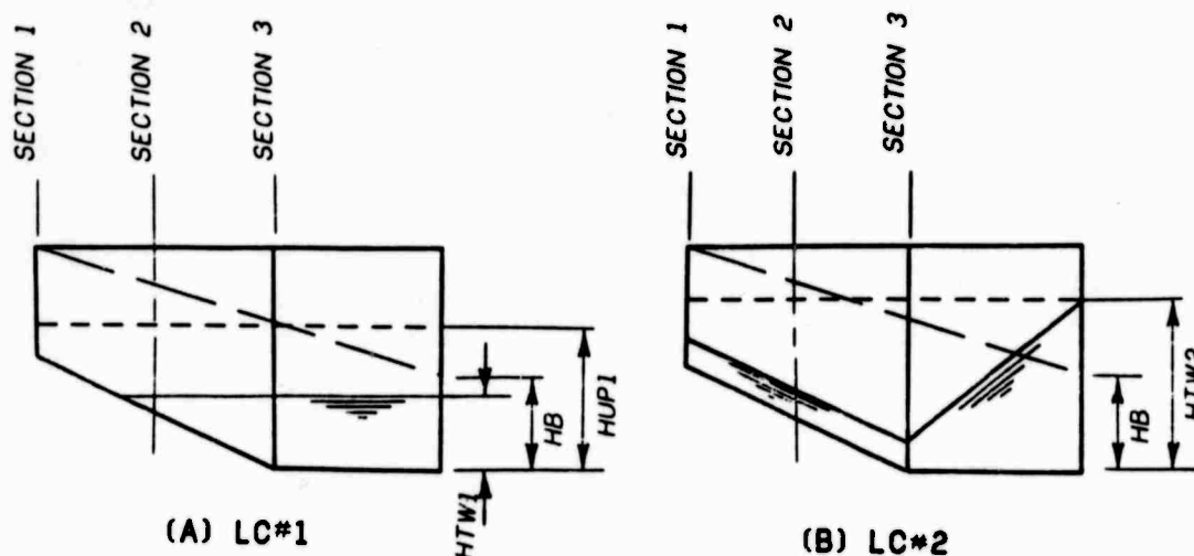
Figure 23. Considerations for sidewall bending, Type (B) basin
