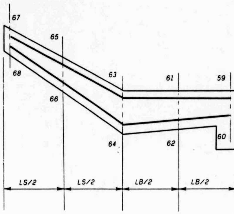
Figure 46. Pavement slab steel layout and point locations
