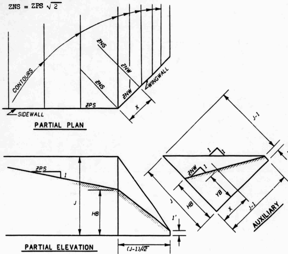
Figure 35. Wingwall earthfill surfaces and slopes
