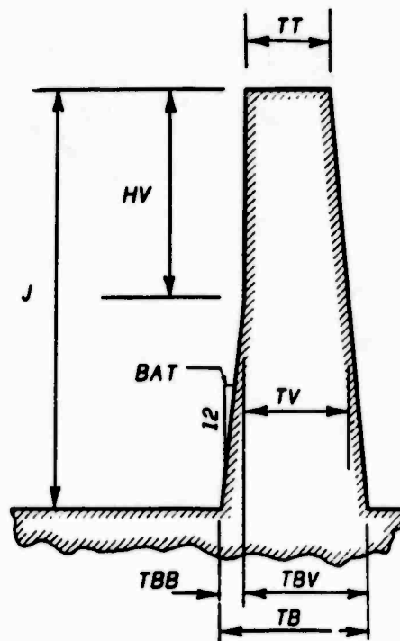
(B) SIDEWALL SECTION
