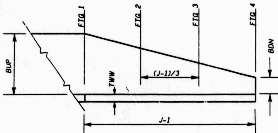
Figure 38. Wingwall footing projections
