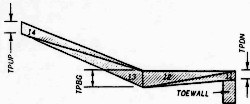
(A) PAVEMENT SLAB THICKNESSES AND VOLUMES
