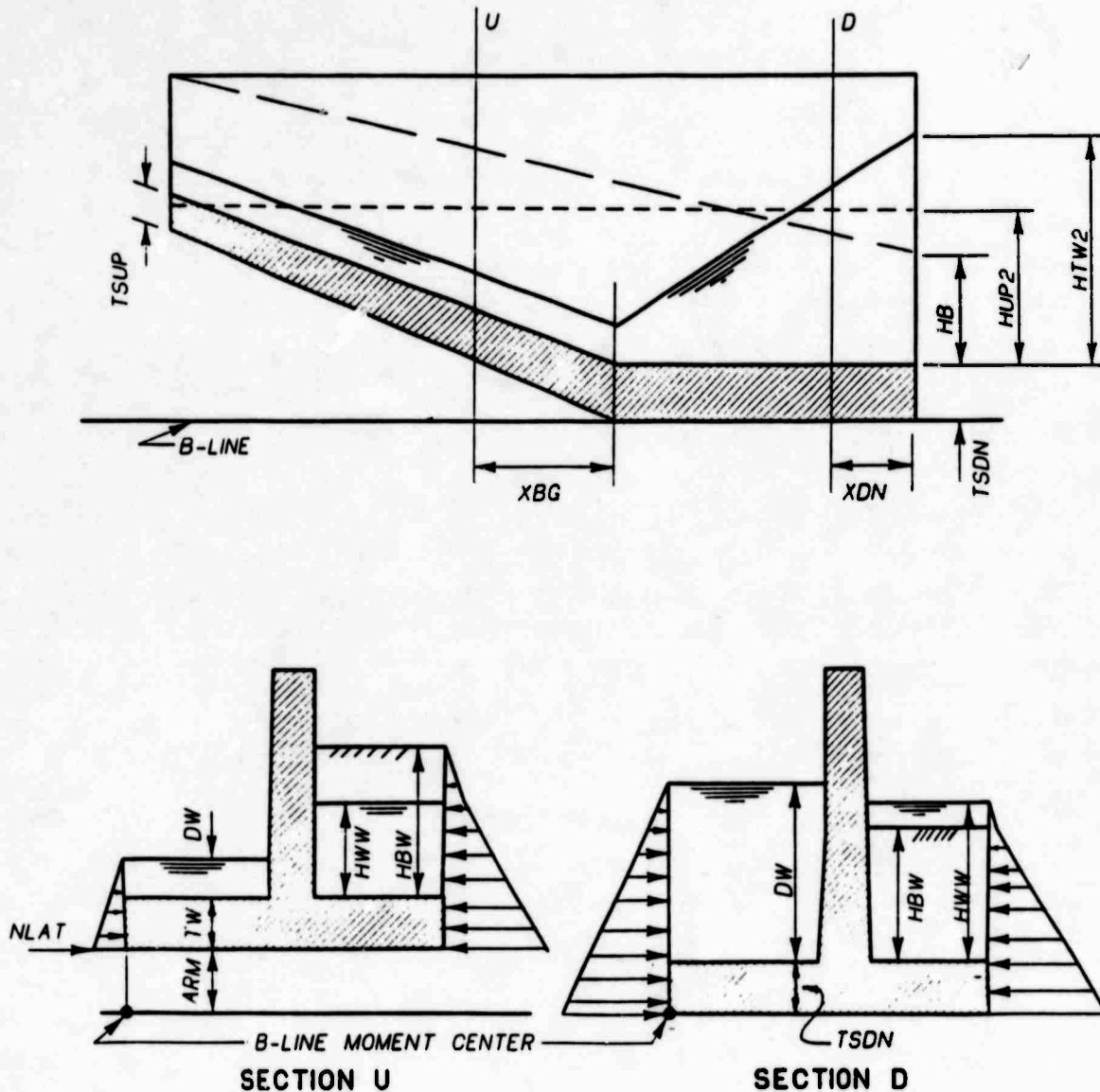
Figure 32. Retaining wall portion lateral force moments, LC#2
