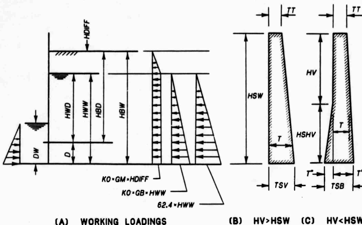
Figure 15. Thickness at bottom of section when HBW > HWW
