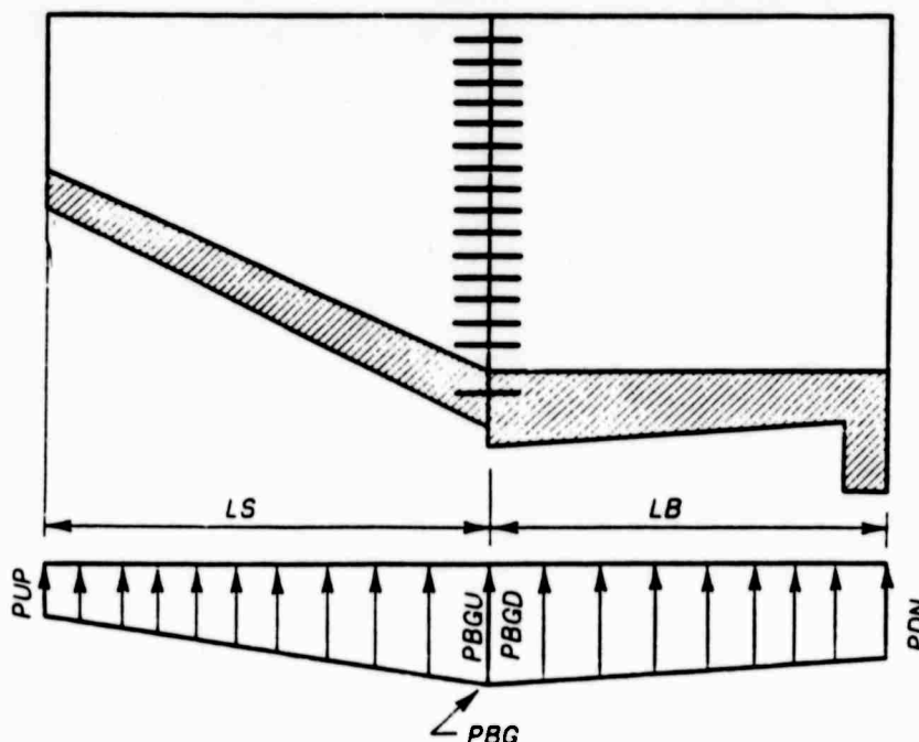
Figure 25. Distribution of bearing pressures type (B) basin
