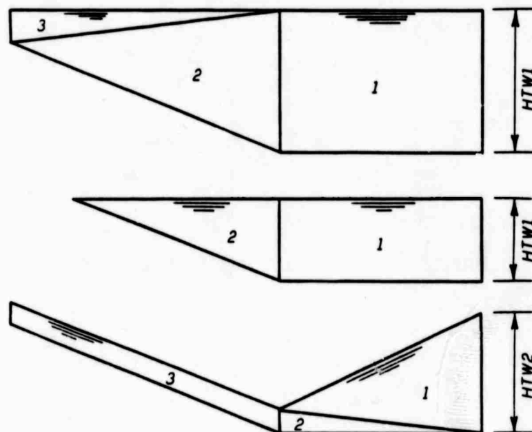
(B) POSSIBLE WATER VOLUMES, LC#1 AND LC#2.
