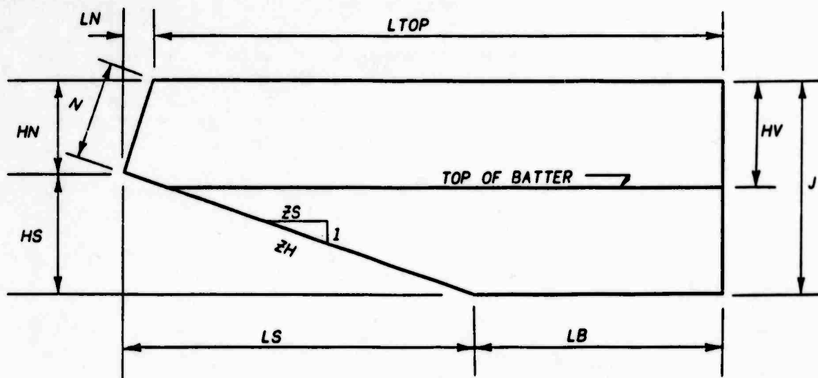
(A) SIDEWALL ELEVATION
