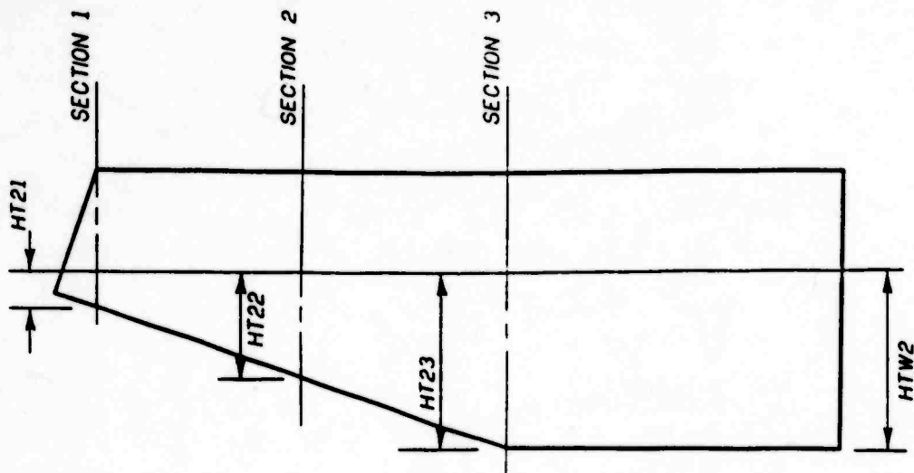
Figure 13. Tailwater depths for load condition No. 2
