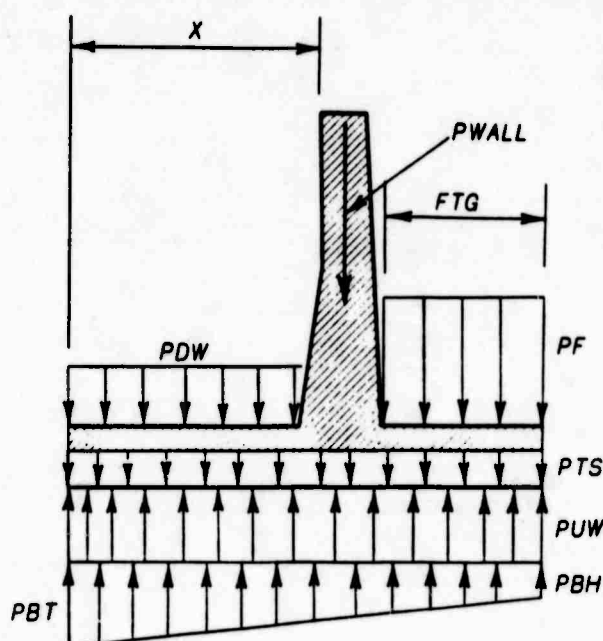
Figure 33. Loadings for base slab shear and moment
