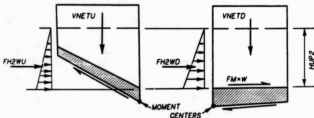
Figure 27. Division of horizontal force, LC#2
