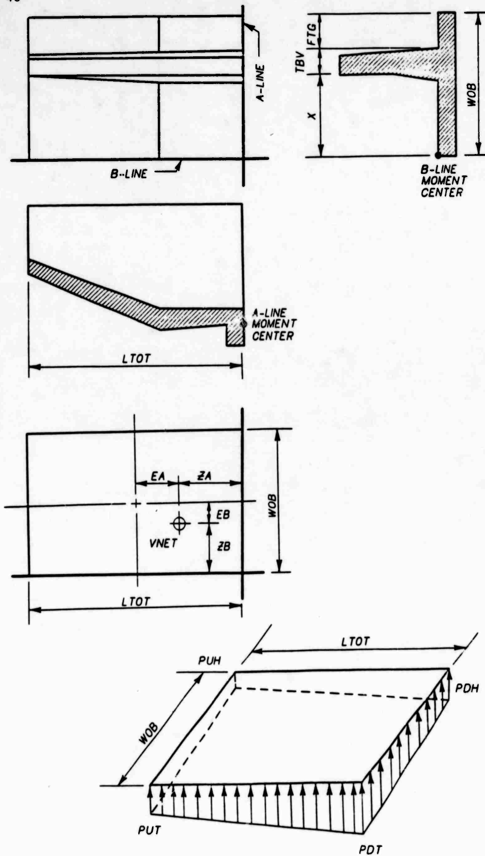
Figure 31. Determination of retaining wall portion bearing pressures
