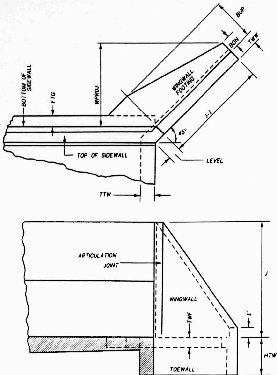
Figure 4. Wingwall layout
