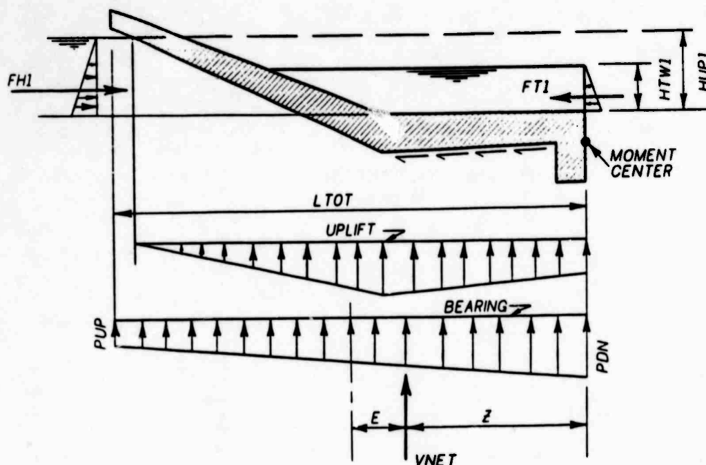
Figure 29. Determination of pavement slab bearing pressures, LC#1
