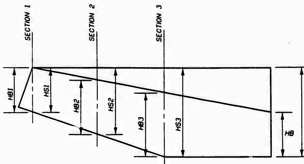
Figure 12. Section and earthfill heights
