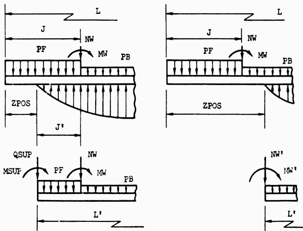
Figure 28. Corrections for indicated tensile reactions.
