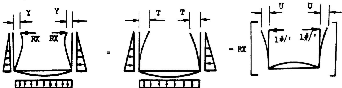
Figure 16. Type TLS frame displacements, typical loading.
