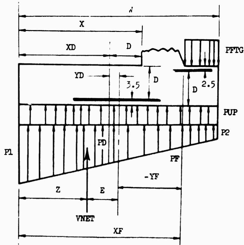
Figure 8. Investigation of footing shears.
