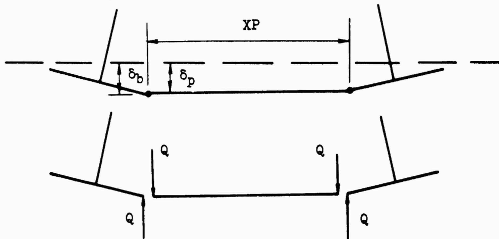
Figure 10. Joint shears in Type T3FV channels.
