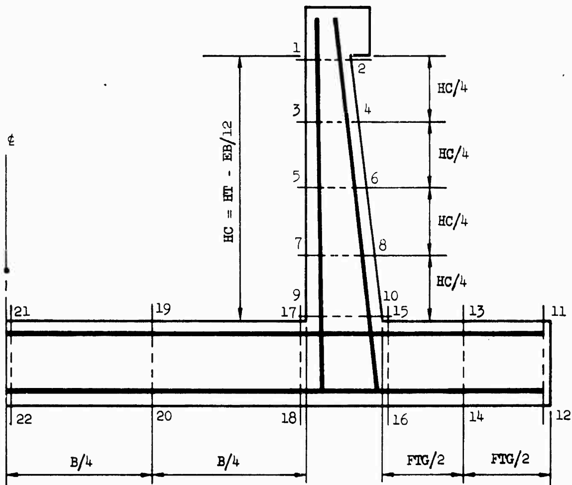
Figure 39. Type T1S steel layout and point locations.
