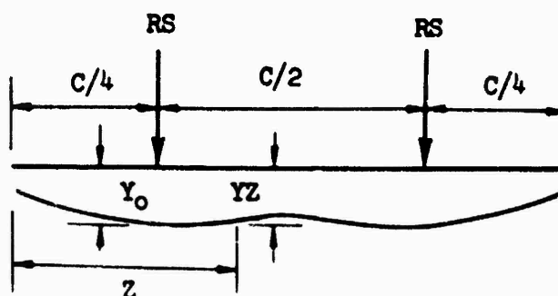
Figure 17. Alternate method of solution for edge beam analyses.
