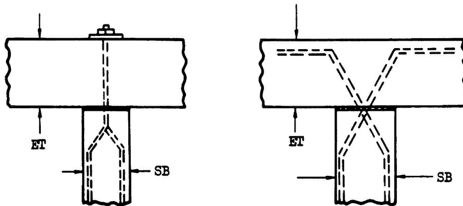
Figure 14. Possible strut-to-wall connections.
