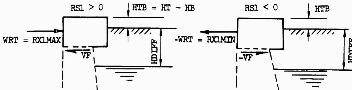
Figure 23. Shear at top of wall; LC#1 when HB > HW1 , HTB < EB/12 , and HW1 < HT - EB/12 .
