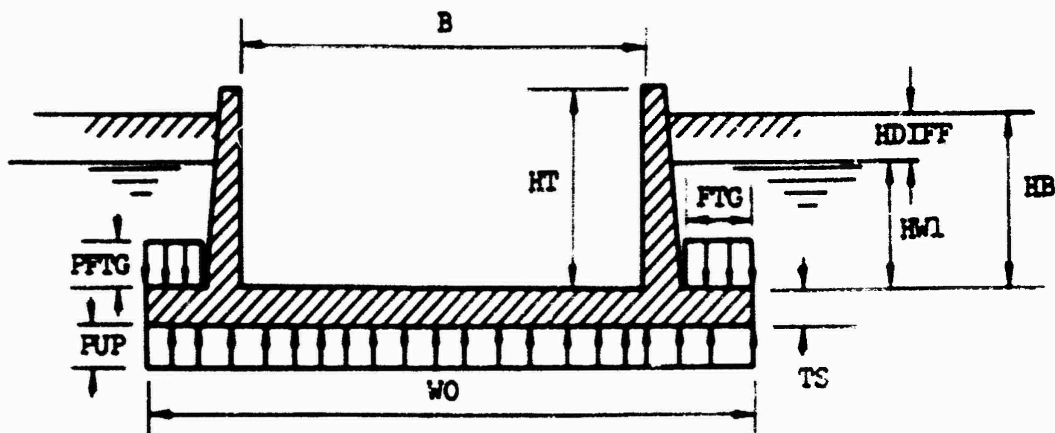
Figure 6. Flotation condition, \text{LC}\#1 when \text{HB} > \text{HWL} .
