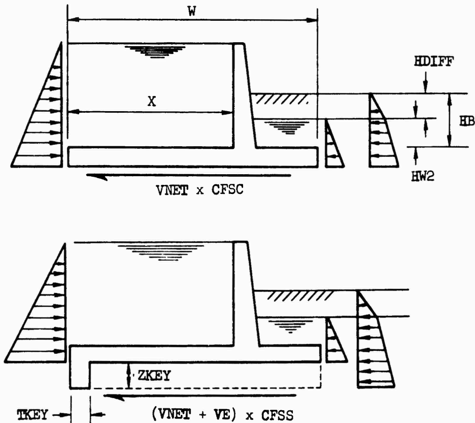
Figure 34. Sliding of type T3F retaining wall portion.
