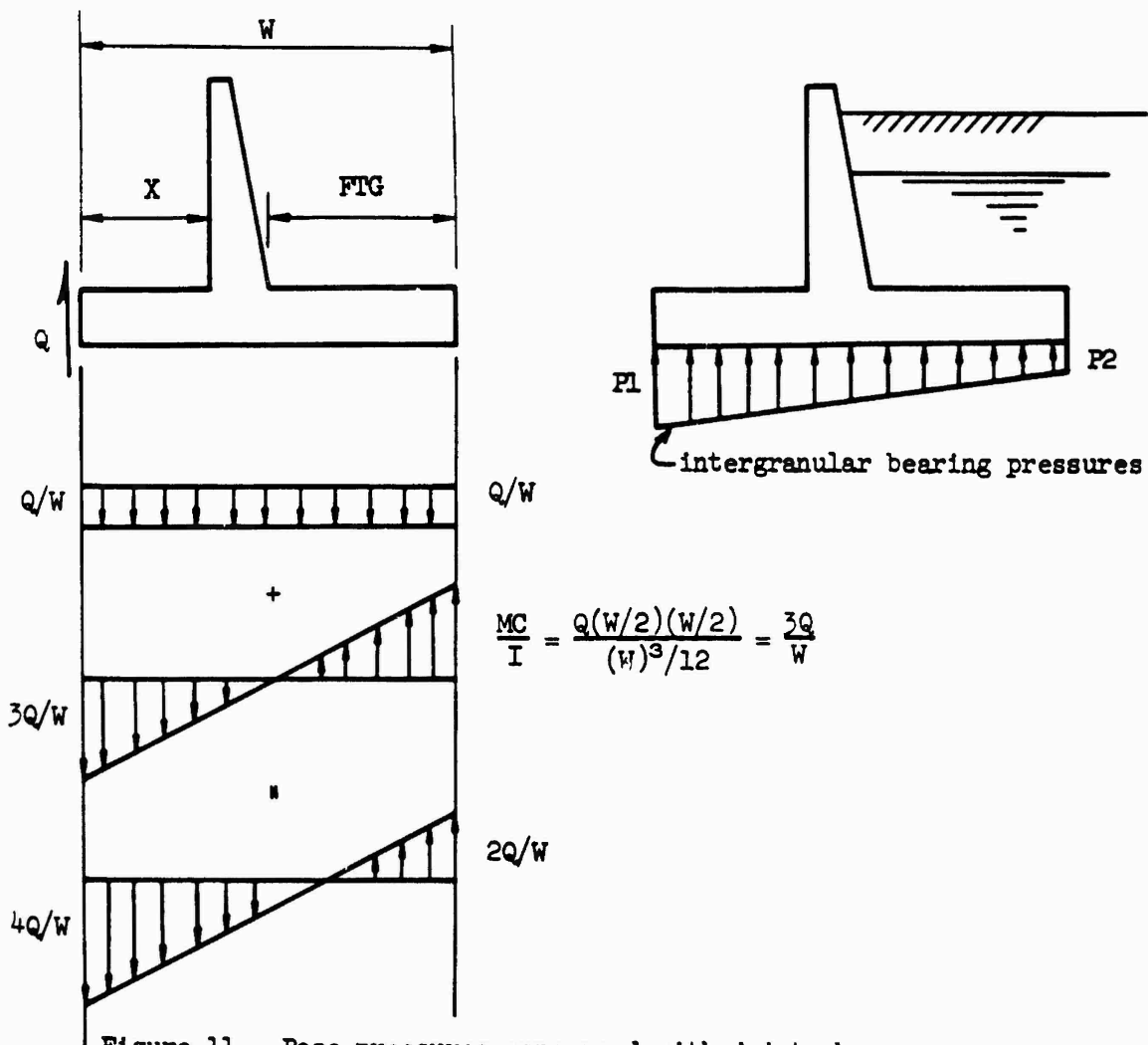
Figure 11. Base pressures concerned with joint shears.
