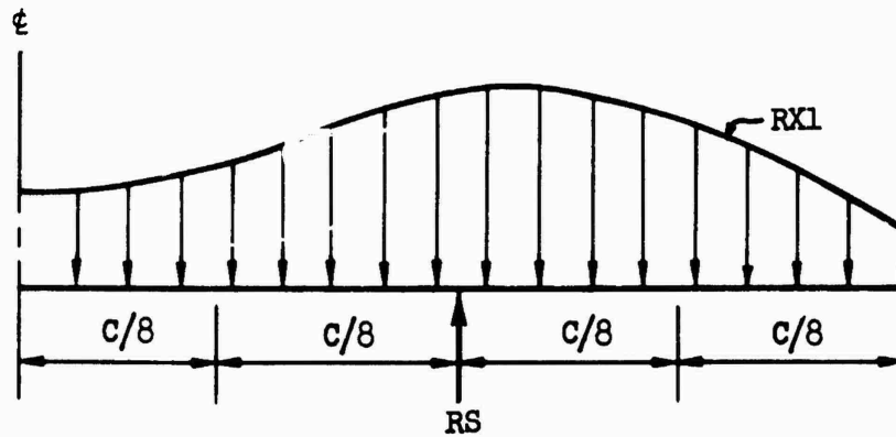
Figure 41. Edge beam loading for LC#1 when RX1 > 0 .
