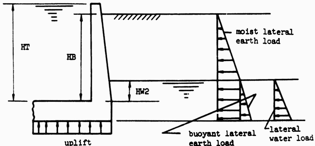
Figure 3. Load condition No. 2.
