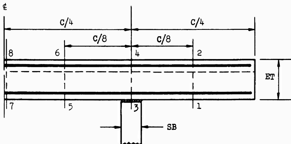
Figure 40. Plan of edge beam, steel layout and point location.
