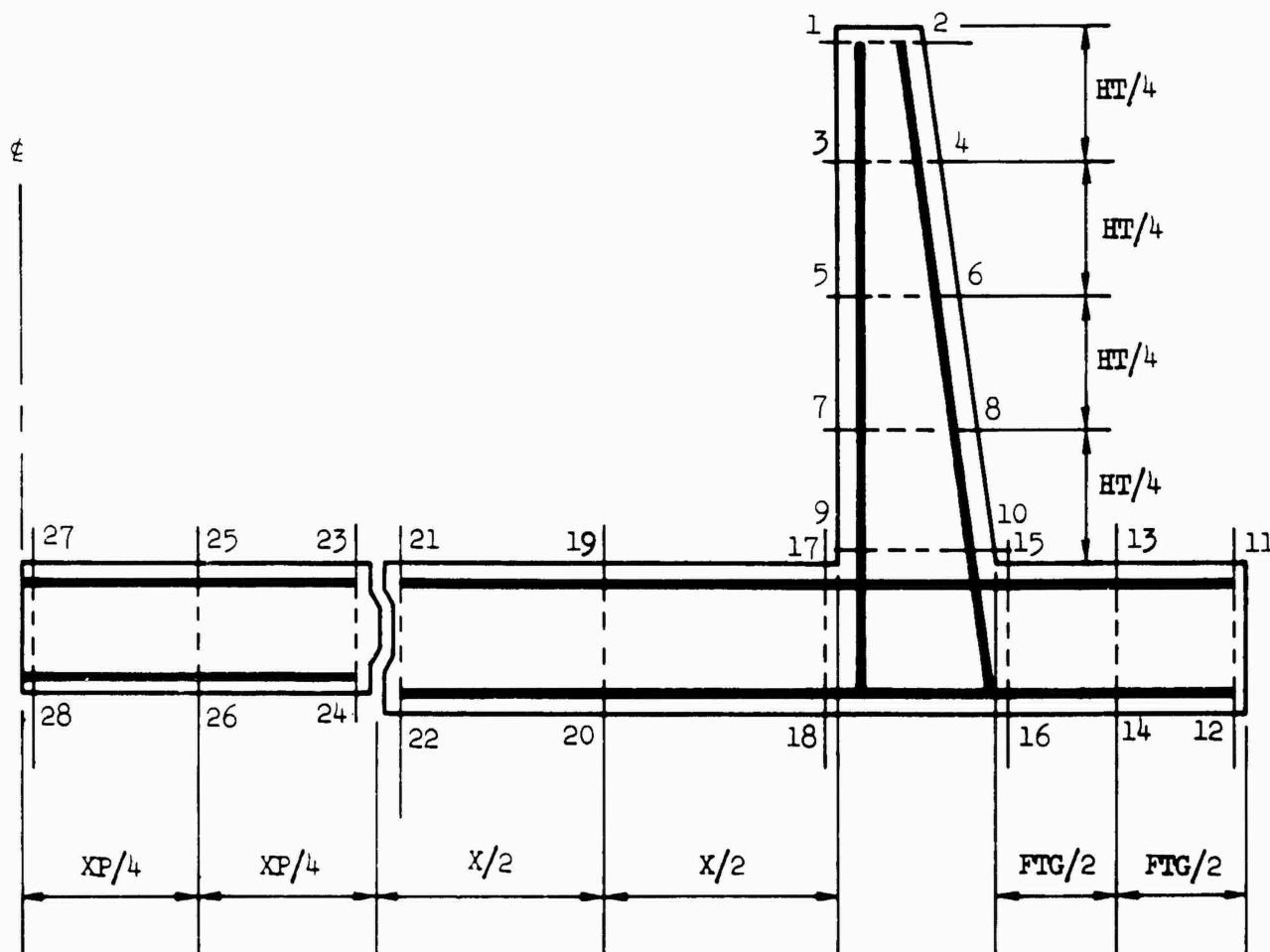
Figure 36. Type T3FV steel layout and point locations.
