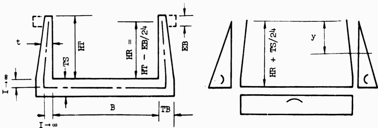
Figure 18. Evaluation of frame U and n.
