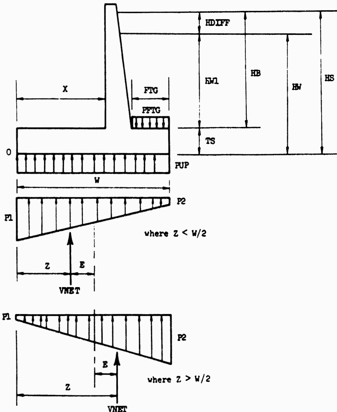
Figure 7. Bearing pressures, LC#1 when H_B > H_{W1} .
