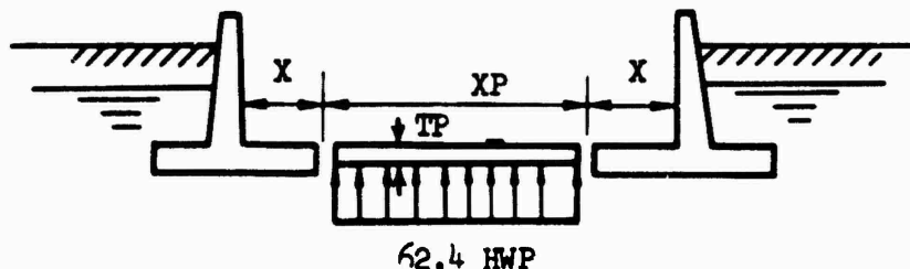
Figure 9. Pavement slab flotation, type T3F.
