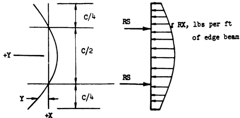
Figure 15. Edge beam loading and displacement.
