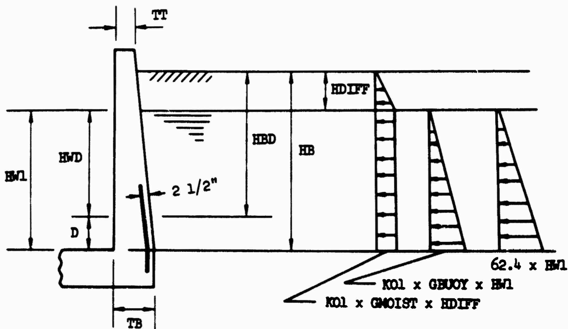
Figure 5. Thickness TB for LC#1 when HB > HWL.
