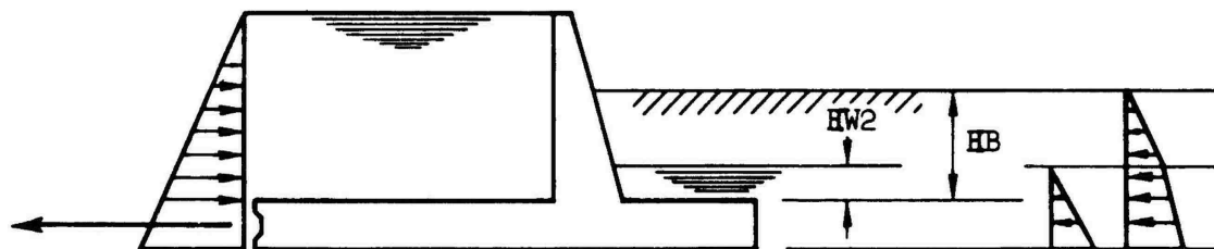
Figure 37. Direct tension through shear joint for LC#2.
