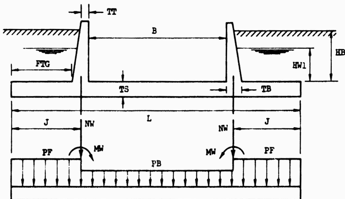
Figure 31. Floor slab analyses and loading for LO#1 when H_B > H_{W1} .
