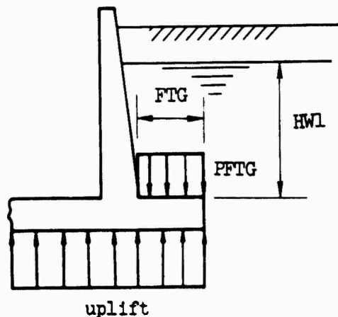
Figure 4. Flotation conditions.
