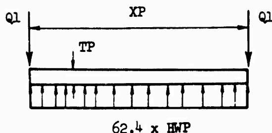
Figure 12. Pavement slab flotation, type T3FV.
