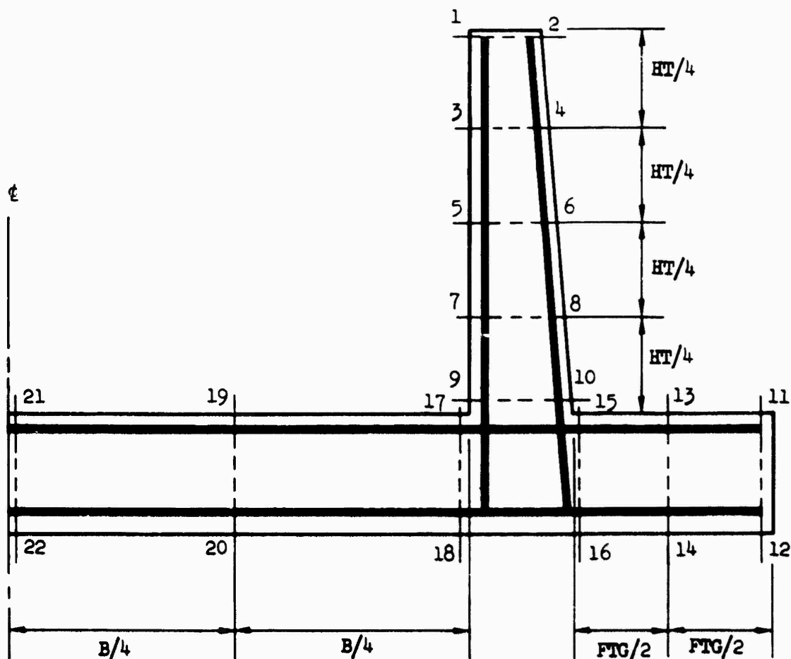
Figure 29. Type T1F steel layout and point locations.
