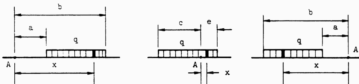
Figure 26. Uniform loading cases, infinite beams.
