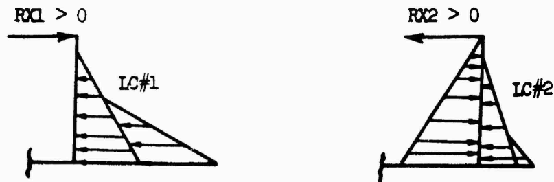
Figure 21. Sense of positive edge beam loading.
