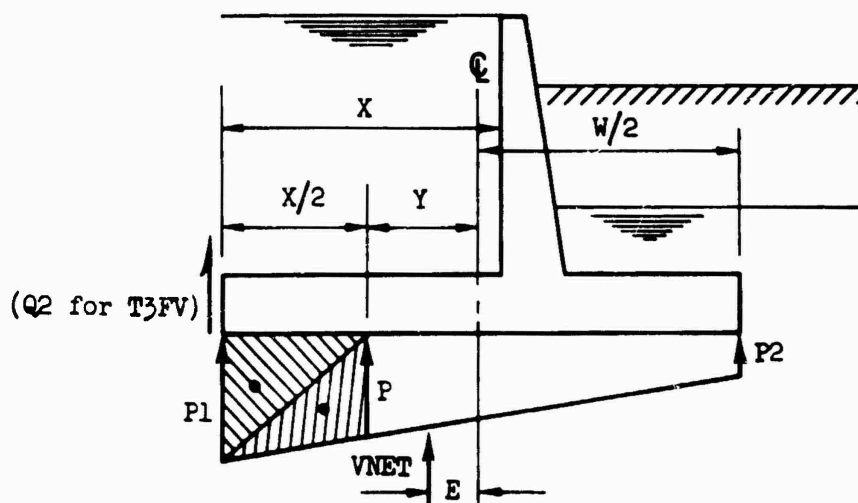
Figure 35. Contact pressure distribution for LC#2.
