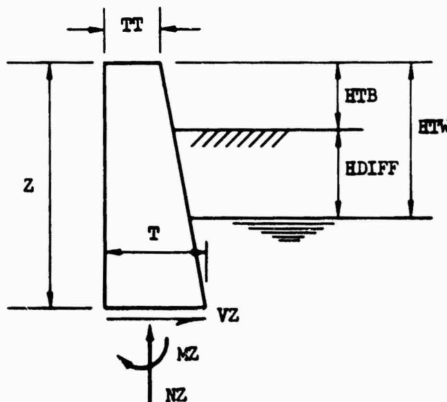
Figure 30. Wall steel design for LC#1, HB > HW1 , and Z > HTW .
