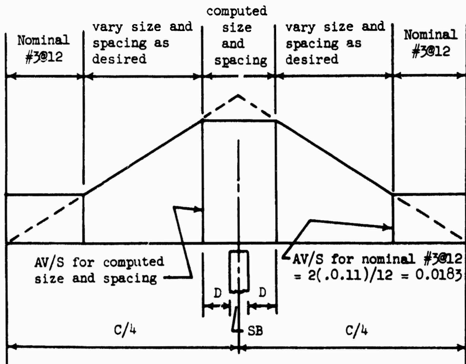
Figure 42. Layout of edge beam stirrups.
