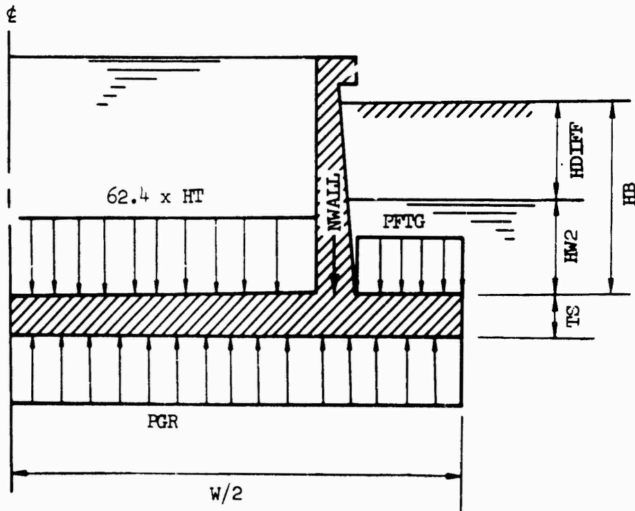
Figure 19. Vertical forces involved with frame T and m, LC#2 when H_B > H_{W2} .
