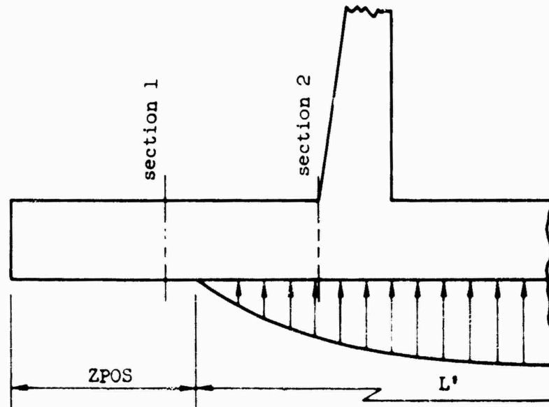
Figure 32. Determination of form of shear and moment computations.
