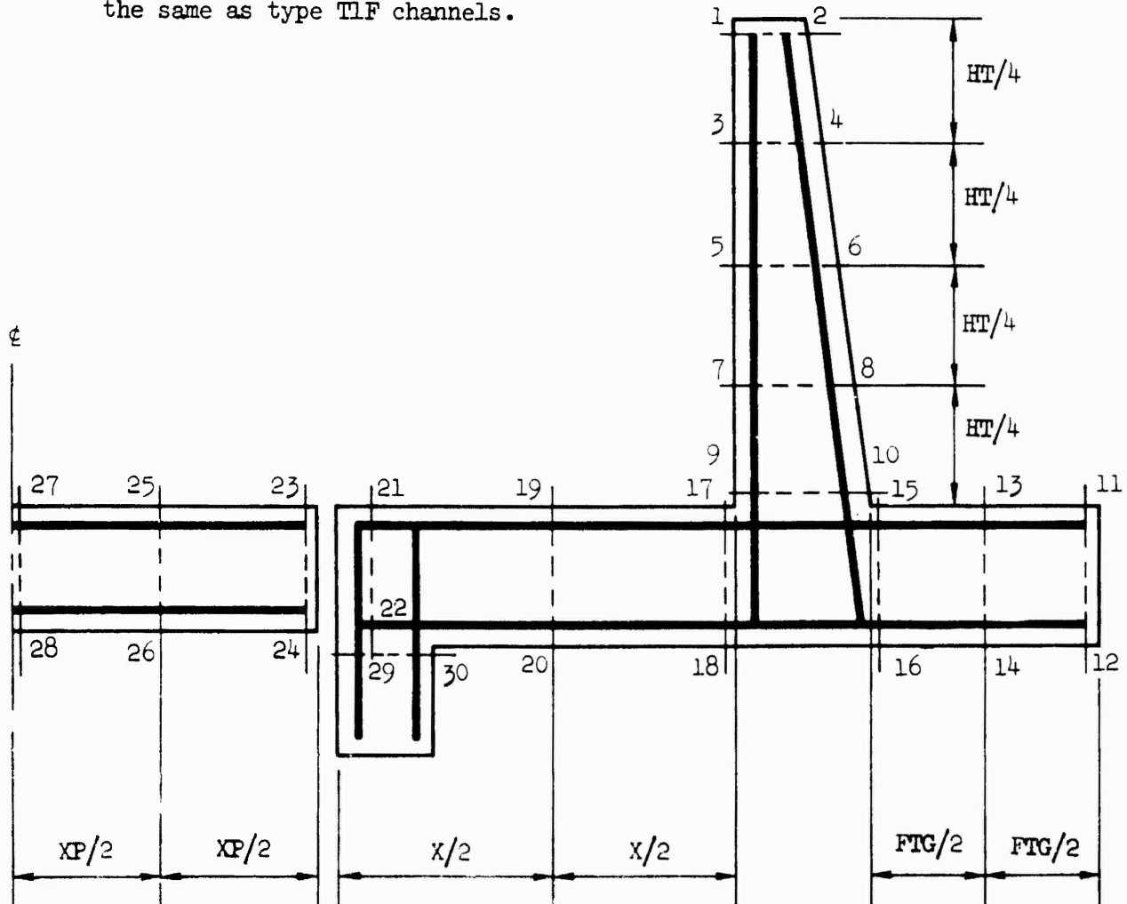
Figure 33. Type T3F steel layout and point locations.
