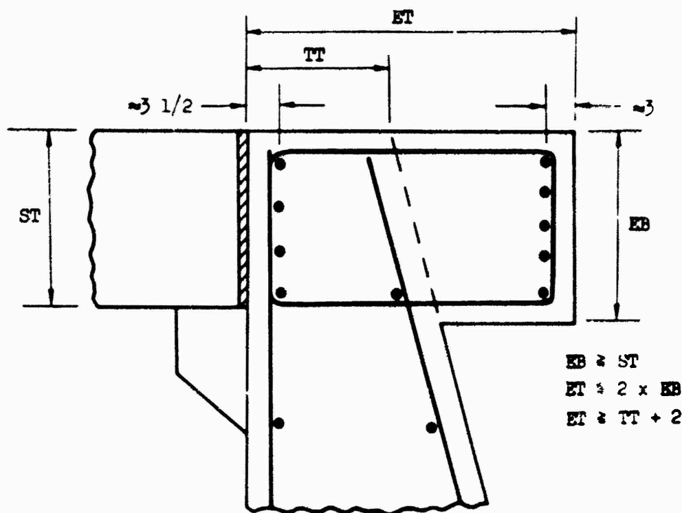
Figure 22. Edge beam section.
