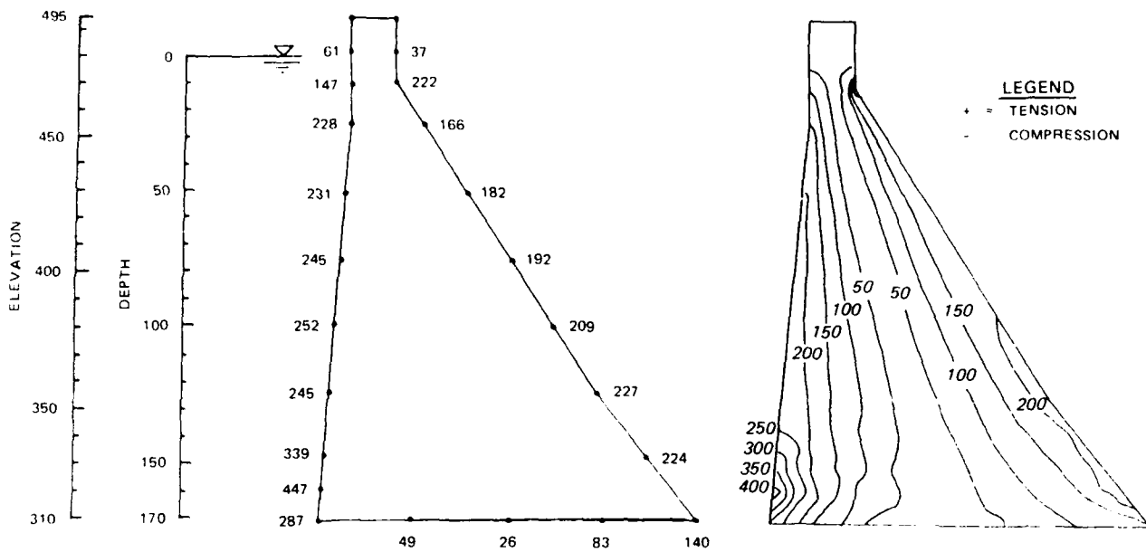
Figure 34. Dynamic stresses (SYY) for E_r/E_c ratio of 0.25
