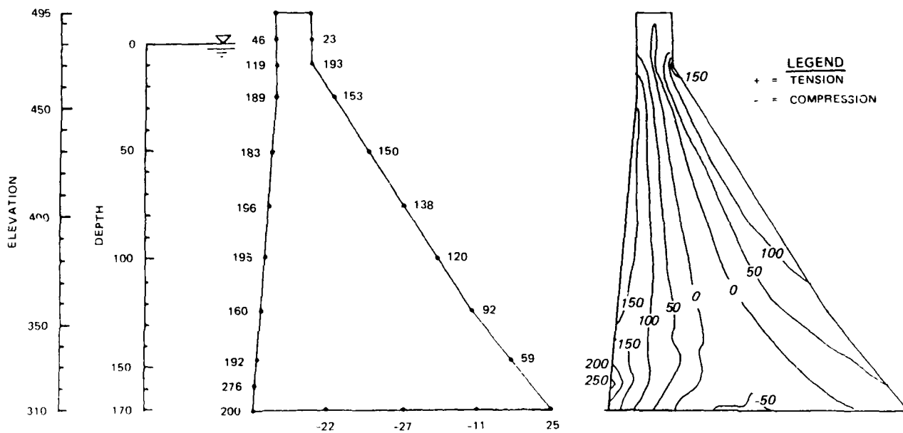
Figure 35. Maximum tensile (static plus dynamic) stresses (SYY) for E_r/E_c ratio 0.25
