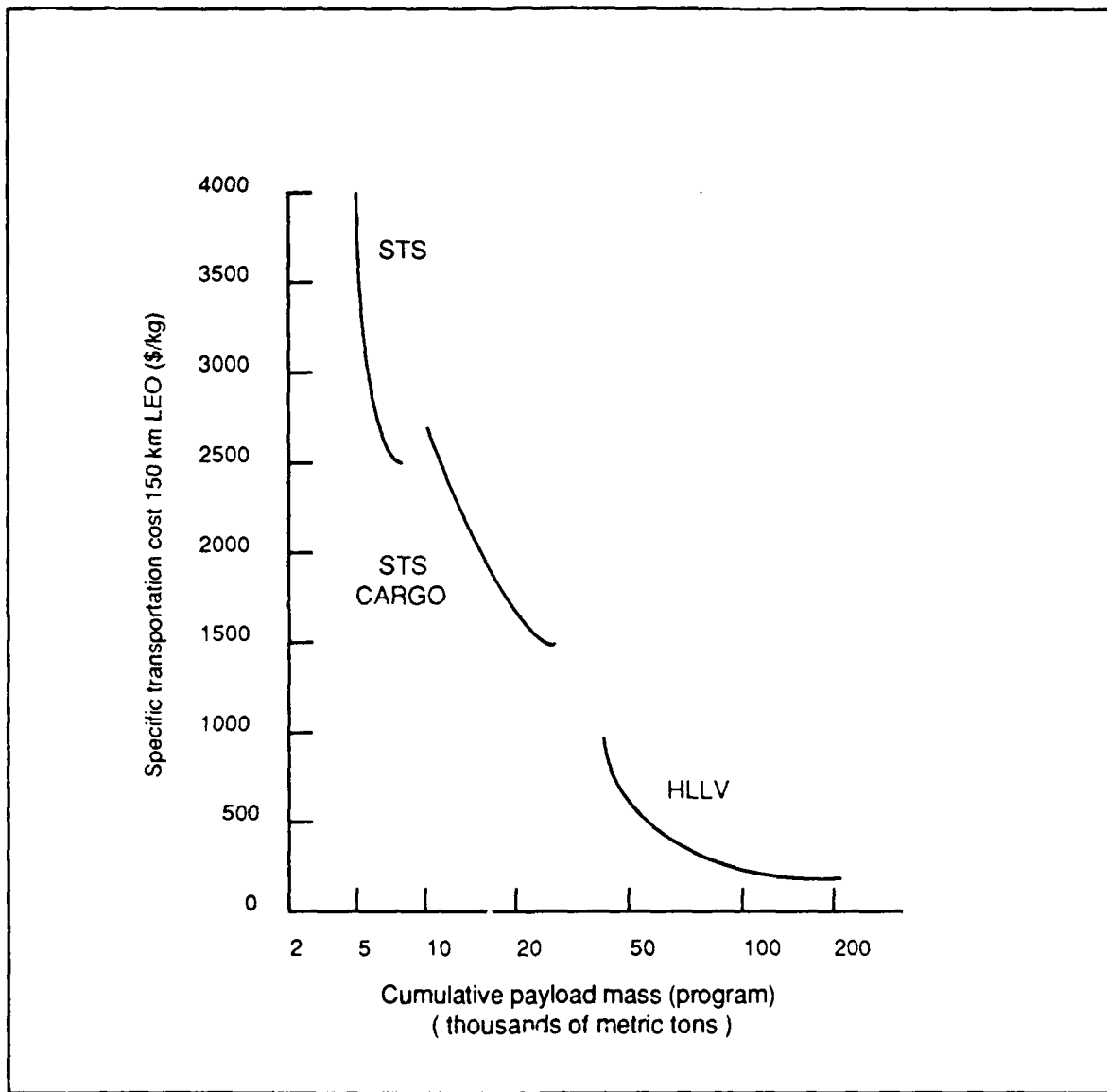
Figure 6.6 Cost-effectiveness of Launch Vehicles
