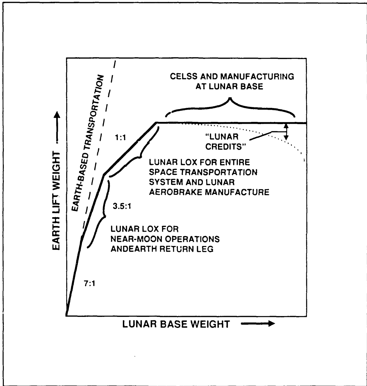
Figure 3.6 Earth Lift Weight Versus Lunar Base Weight
