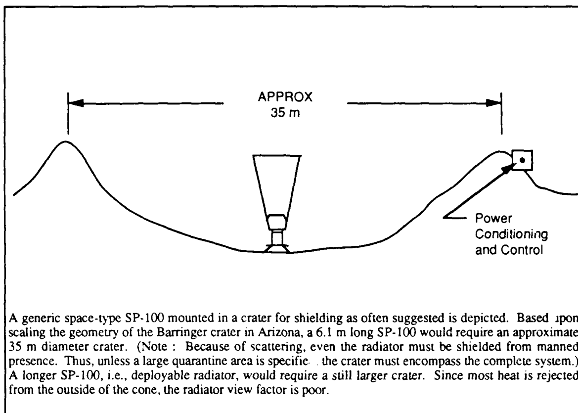
Figure 5.4 SP-100 Crater Concept
