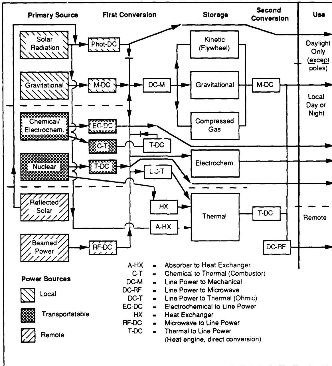
Figure 5.1 Possible Power Sources
