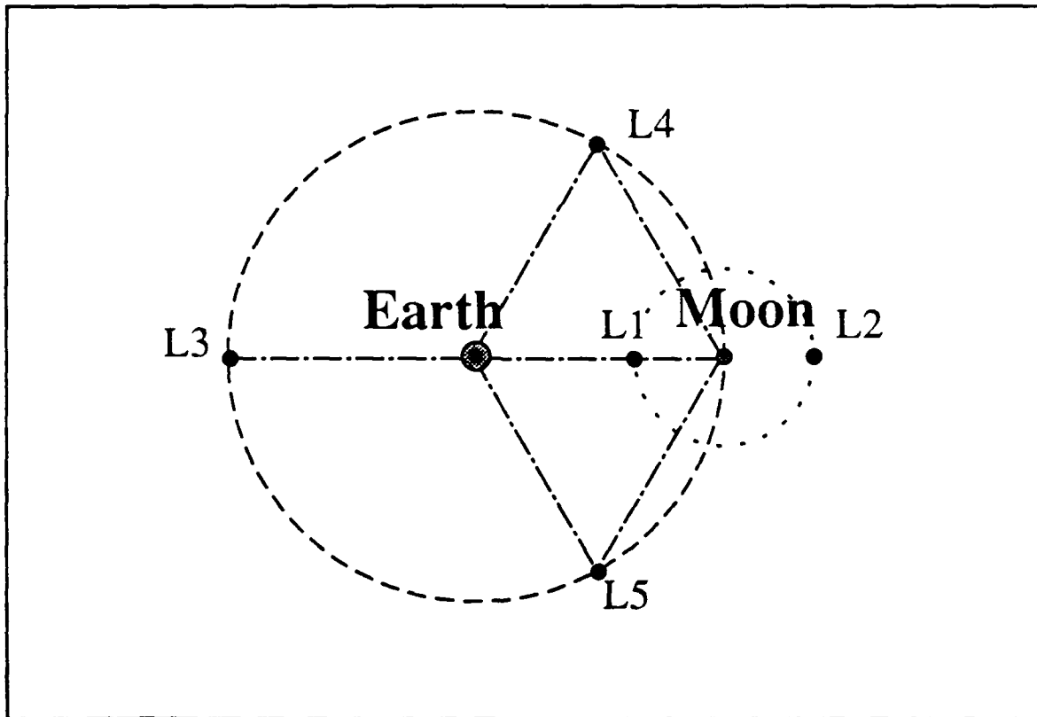
Figure 6.3 Libration Points in the Earth-Moon System
