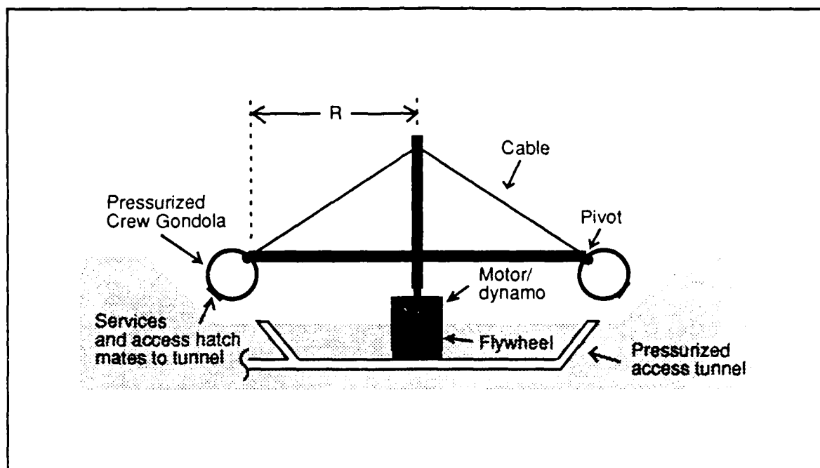
Figure B.1 Artificial Gravity Carousel
