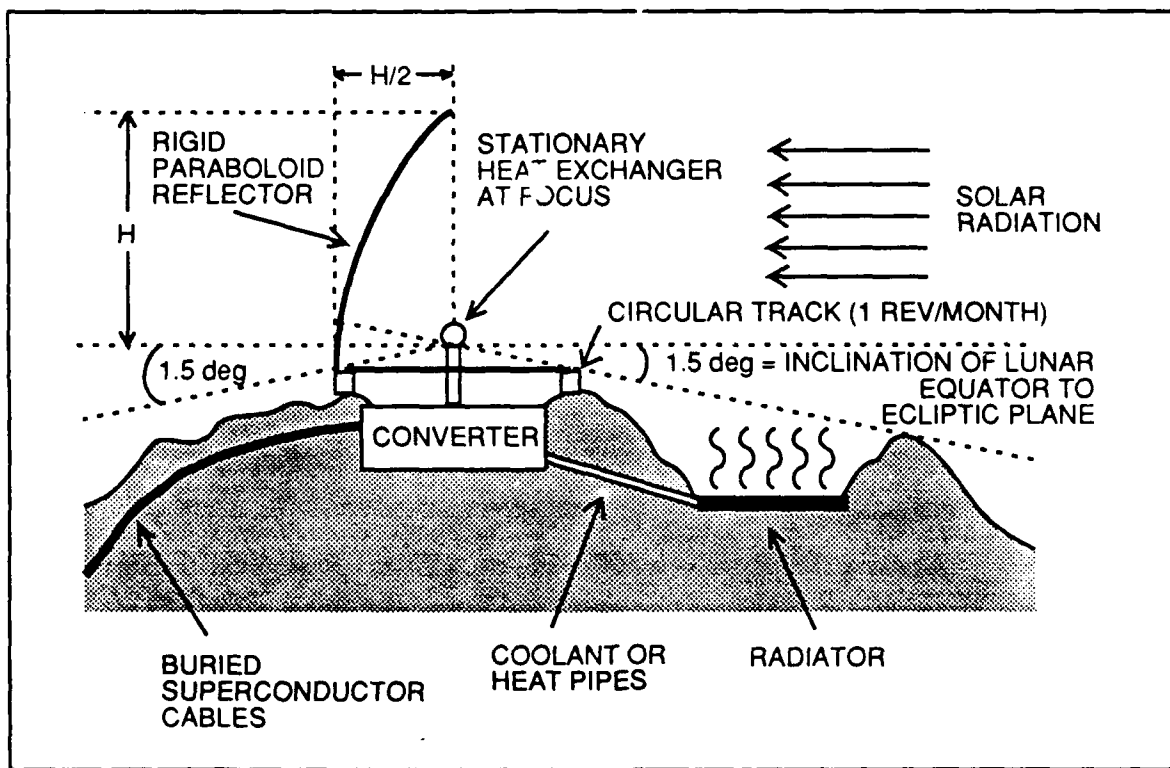
Figure A.1 Solar-Electric Power Plant at Lunar Pole
