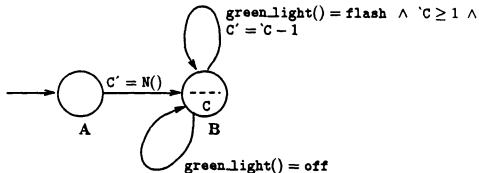
Figure 1: A_P , an example automaton diagram.
