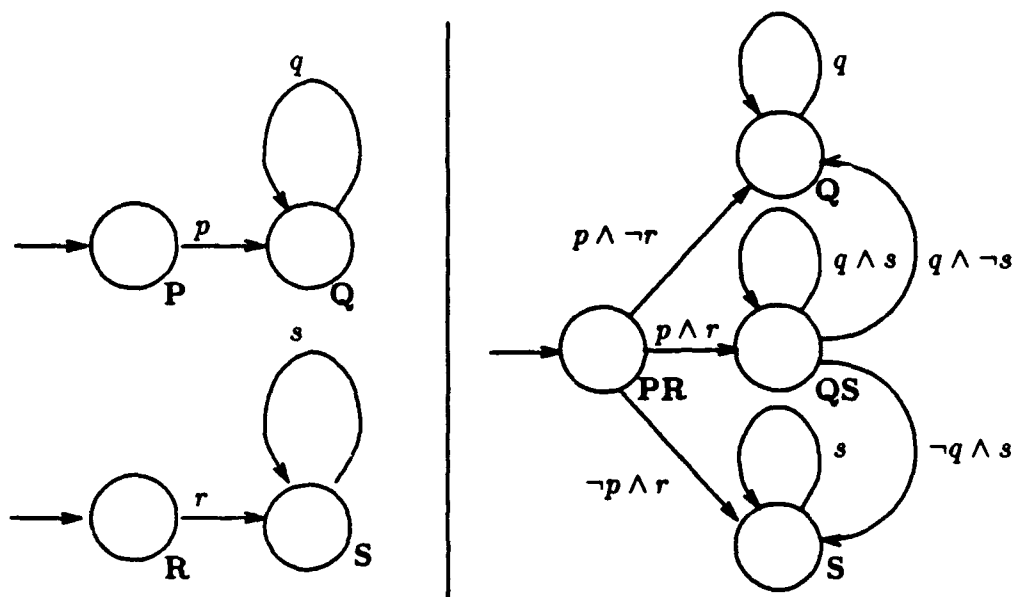
Figure 2: A_K (left) and A_{K_s} (right).
