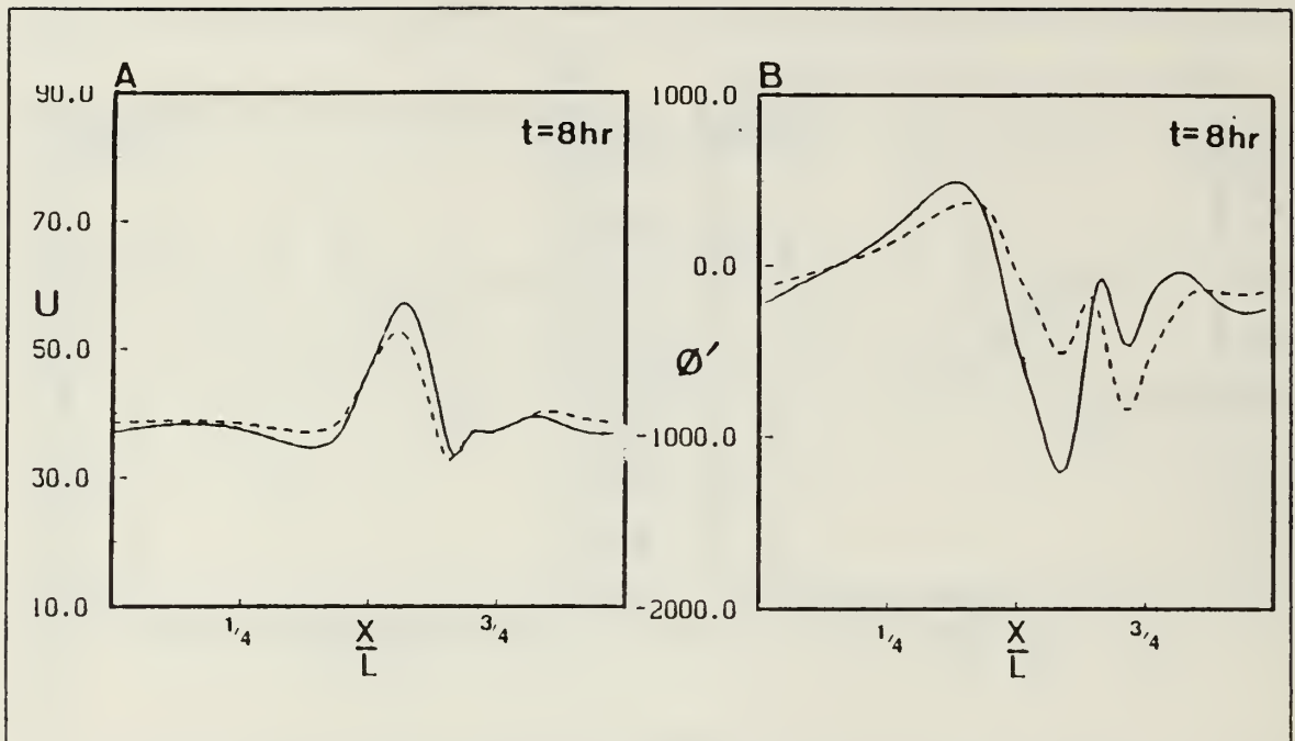
Figure 18. Comparison of Perturbations in Rotating and Non-rotating System (m/s)^2 for Case II A) u and B) \phi' with IIRSL. Solid line indicates non-rotating system; the dashed line indicates solution for the rotating system.
