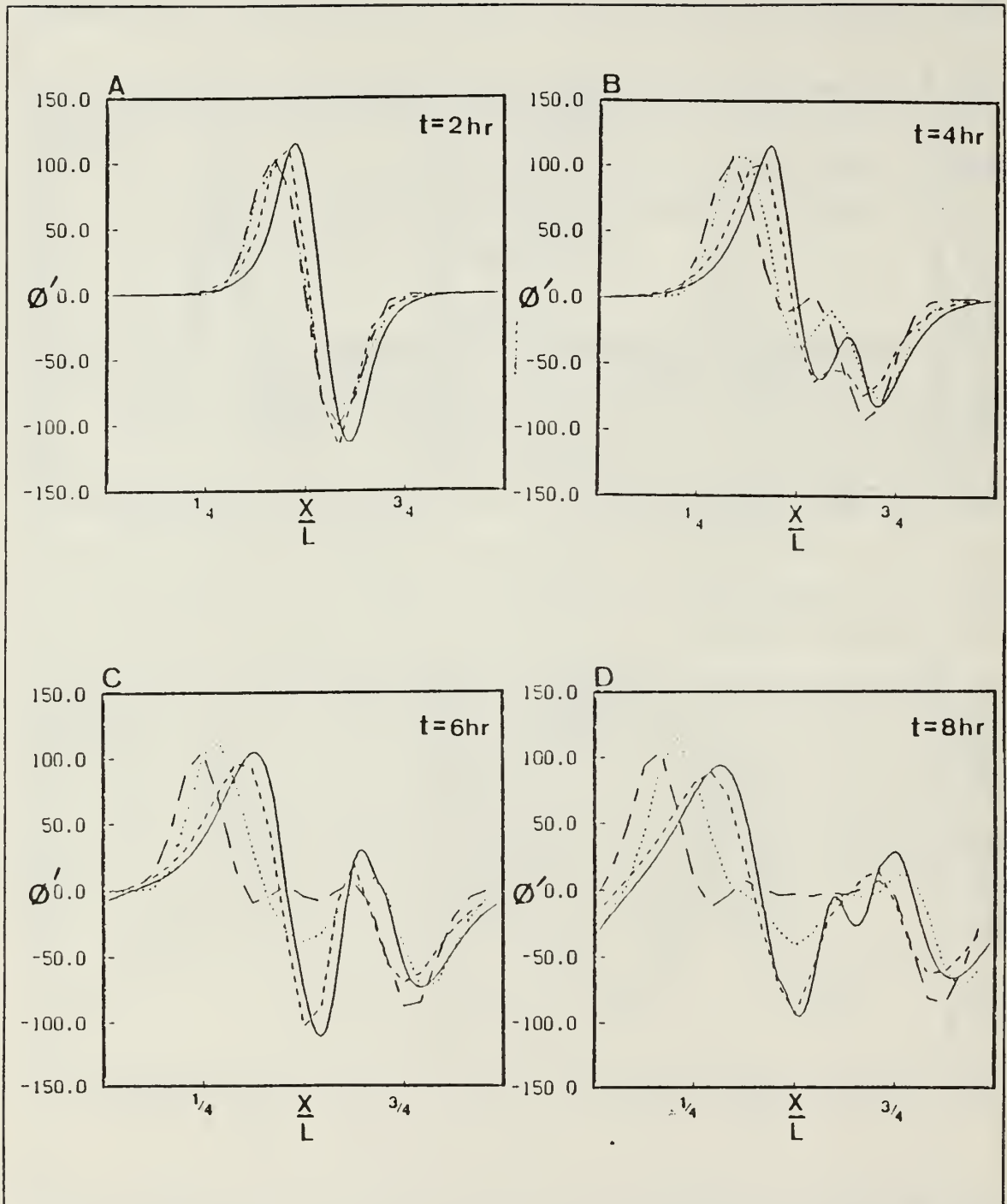
Figure 8. Experiment 1, Case I: \phi' Field ( m/s^2 ) after A) Two B) Four C) Six D) Eight Hours of Integration for IIRSL (solid line), SLSI (dashed line), SLEX (broken line) and FDEX (dotted line).
