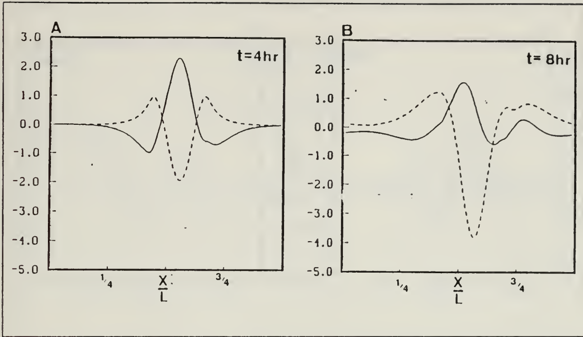
Figure 17. Experiment 2, Case I: u' and v' (m/s) after A) Four B) Eight Hours of Integration with HRSL.
