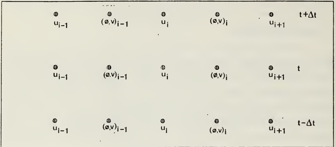
Figure 5. Staggered Grid
