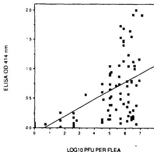
FIGURE 4. Comparison of ELISA OD obtained on 99 single X. cheopis fleas with PFU/flea determinations on pooled fleas from the same cohorts. Regression line of data is ELISA\ OD = -0.098 + 0.144\ log_{10}\ PFU/flea . Includes 14 infected fleas (0 days postinfection) with overlapping ELISA values at 0 = log_{10}\ PFU/flea . Only 1 of these 14 fleas exceeded the OD cutoff for rickettsial positivity ( OD = 0.059 ).
